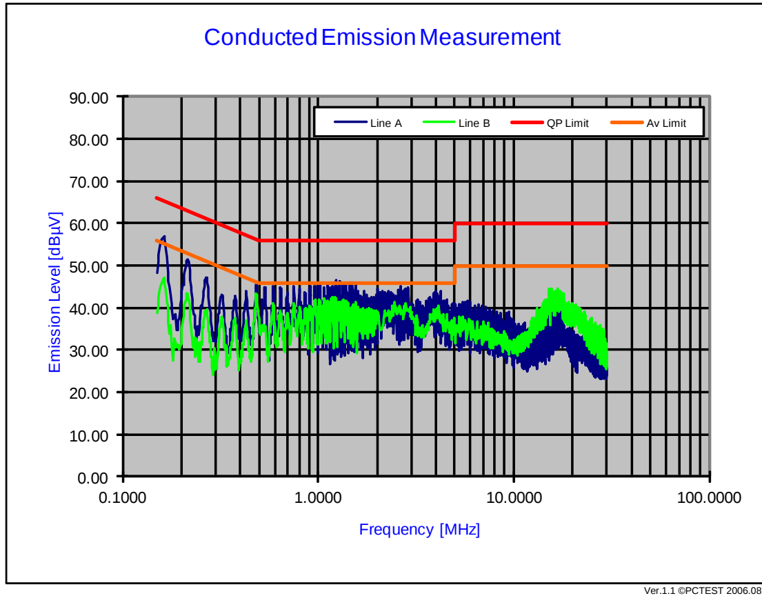
Plot 6-54. Line Conducted Plot with 802.11a (UNII Band 1)
