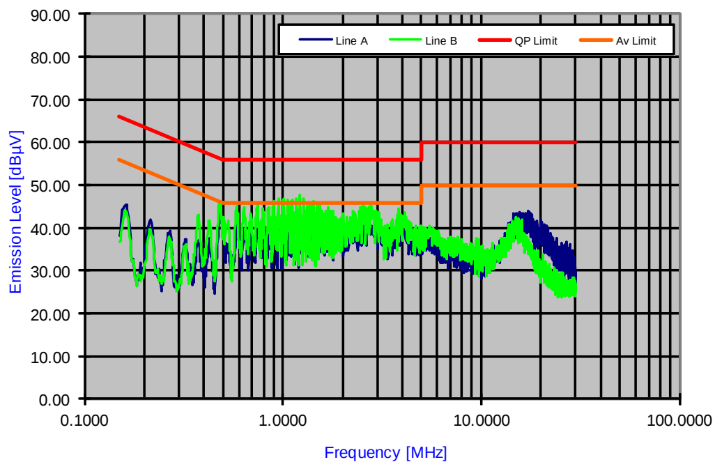
Plot 6-55. Line Conducted Plot with 802.11a (UNII Band 2)
