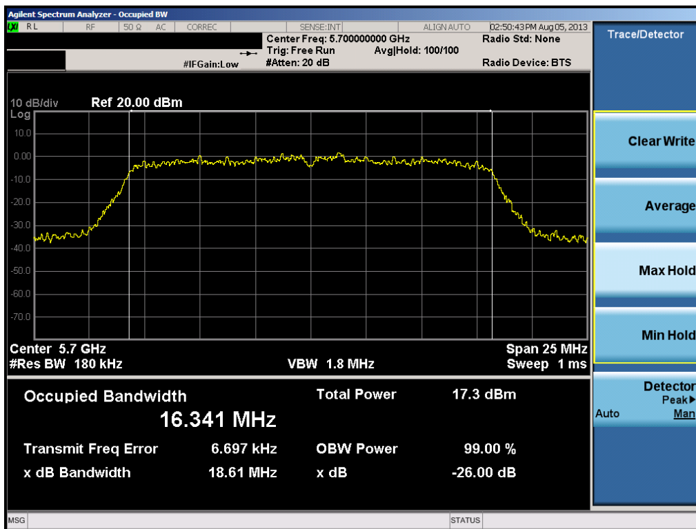
Plot 6-19. 26dB Bandwidth Plot (802.11a (UNII Band 3) – Ch. 140)
