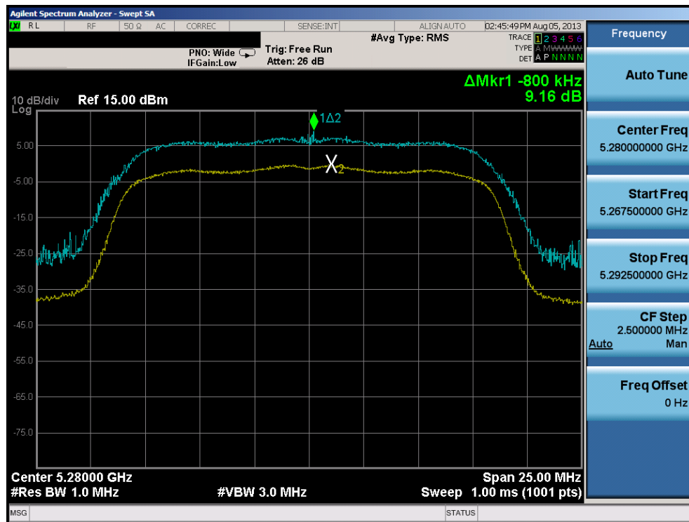
Plot 6-51. Peak Excursion Ratio Plot (802.11a)
