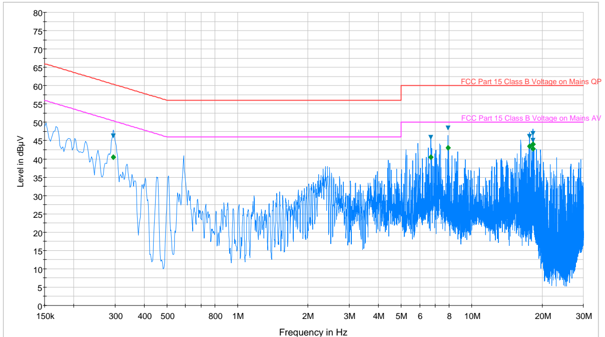
Plot 6-56. Line Conducted Plot with 802.11a UNII Band 2 (L1)
