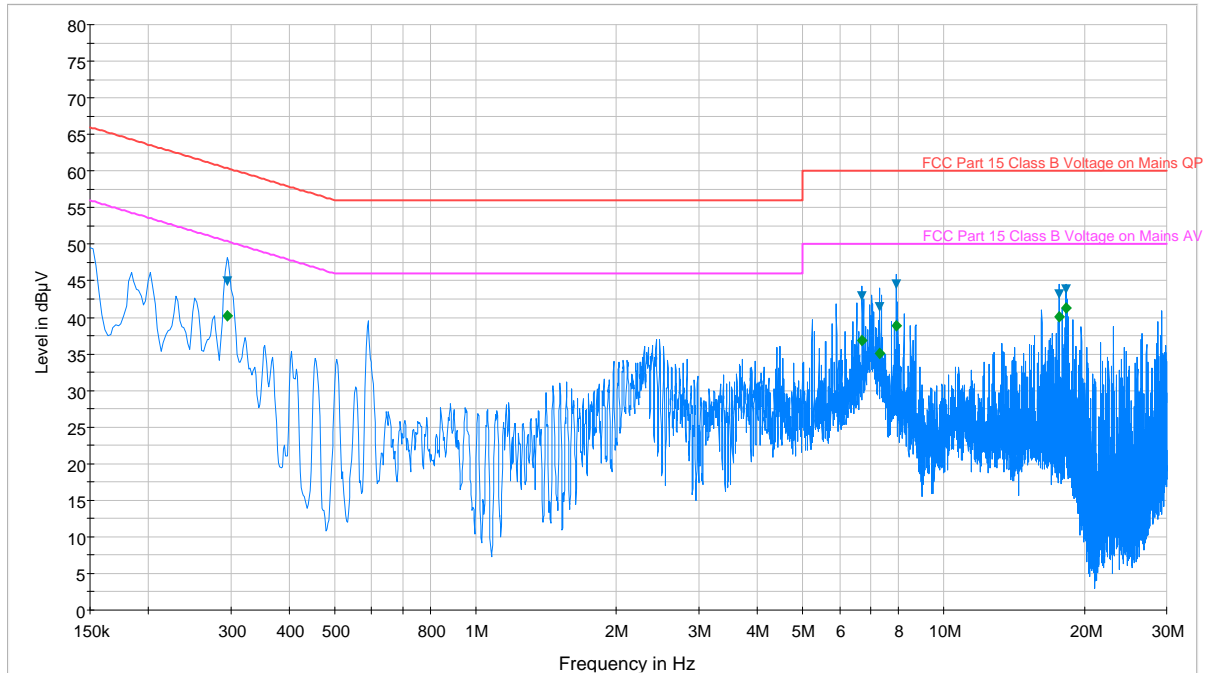
Plot 6-58. Line Conducted Plot with 802.11a UNII Band 3 (L1)
