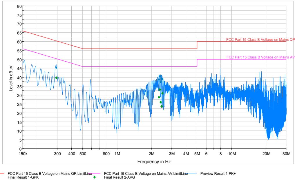
Plot 6-64. Line Conducted Plot with 802.11b (N)
