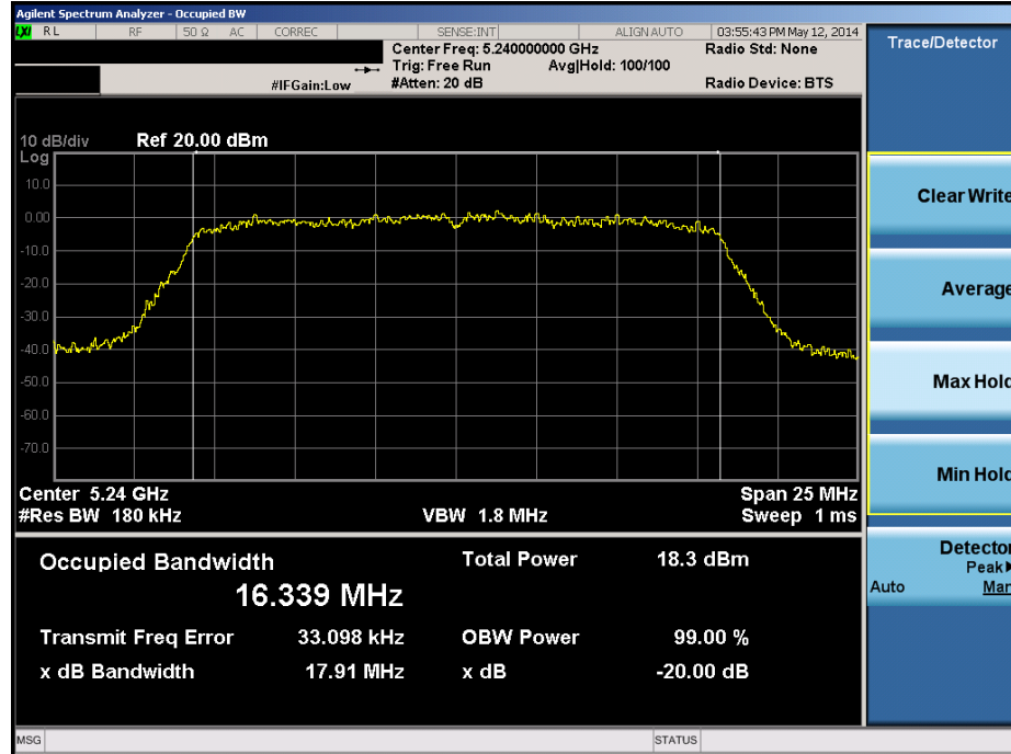
Plot 6-19. 20dB Bandwidth Plot (20MHz BW 802.11a (UNII Band 1) – Ch. 48)
