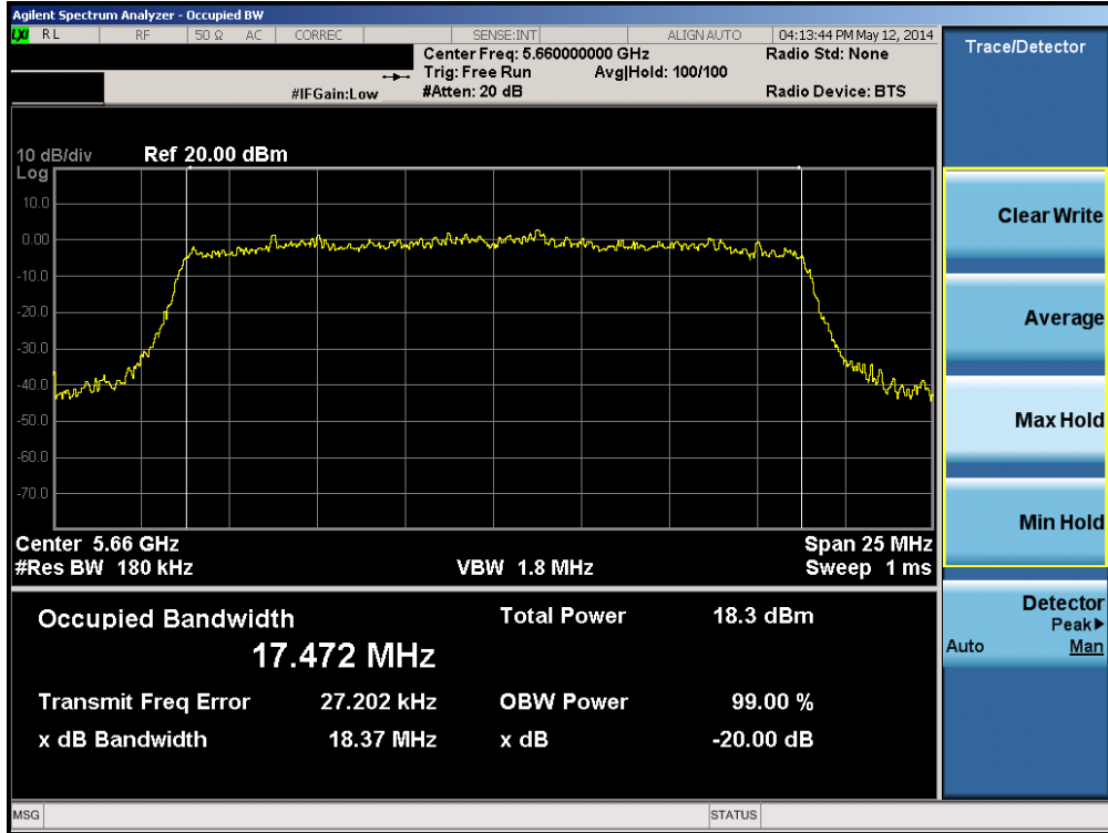
Plot 6-21. 20dB Bandwidth Plot (20MHz BW 802.11n (UNII Band 2C) – Ch. 132)
