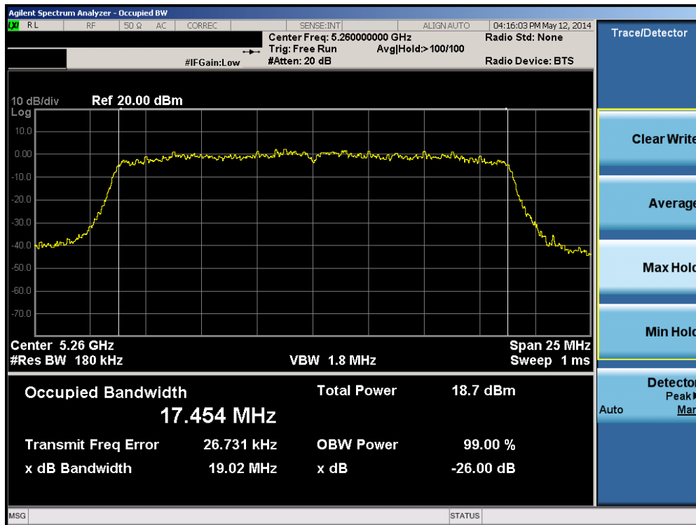
Plot 6-10. 26dB Bandwidth Plot (20MHz BW 802.11n (UNII Band 2A) – Ch. 52)
