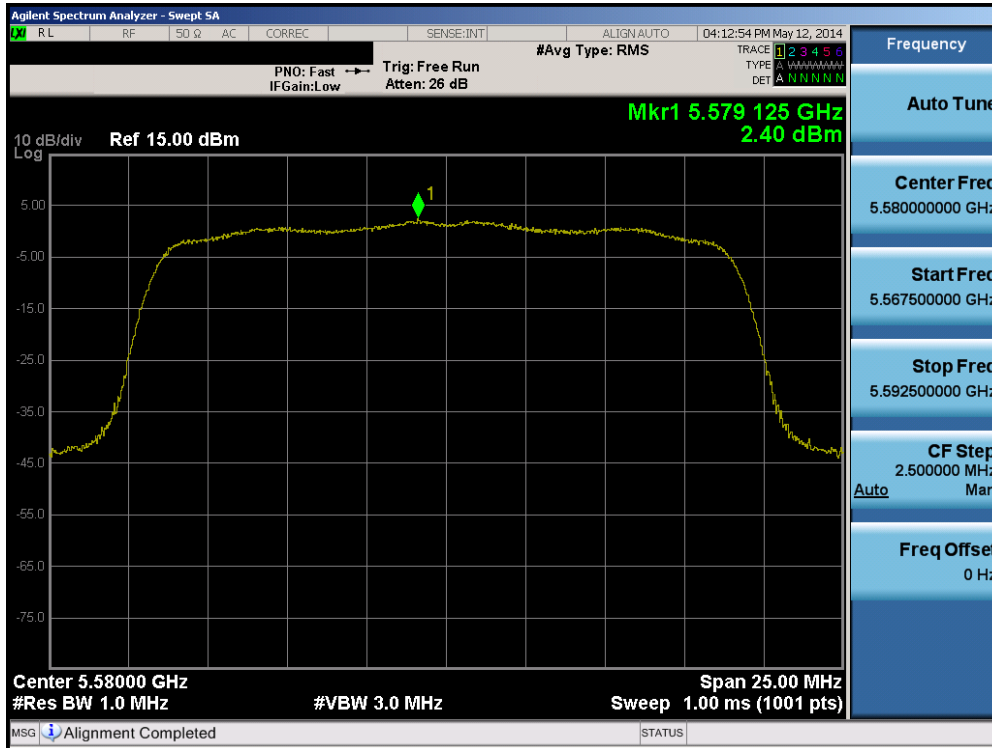
Plot 6-38. Peak Power Spectral Density Plot (20MHz BW 802.11n (UNII Band 2C) – Ch. 116)
