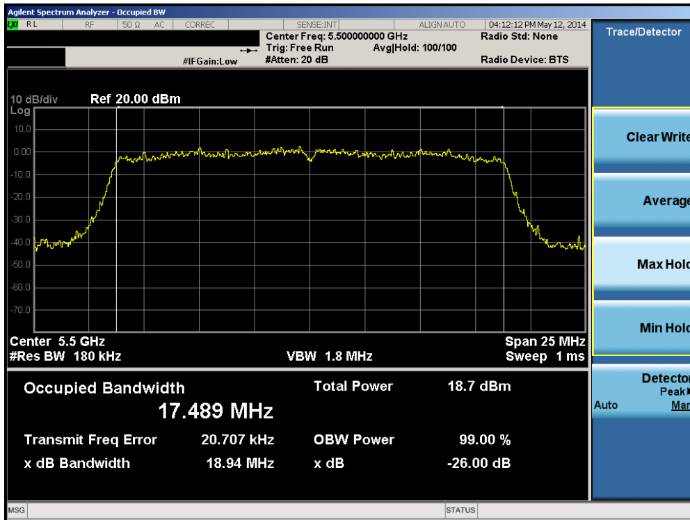
Plot 6-16. 26dB Bandwidth Plot (20MHz BW 802.11n (UNII Band 2C) – Ch. 100)
