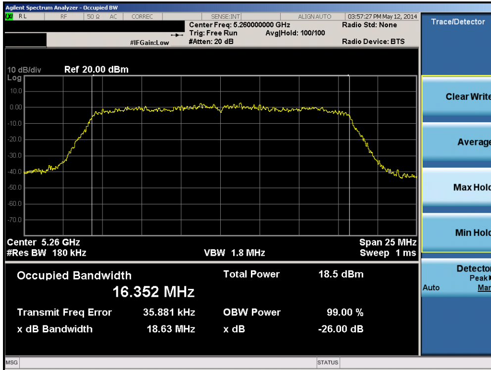
Plot 6-7. 26dB Bandwidth Plot (802.11a (UNII Band 2A) – Ch. 52)
