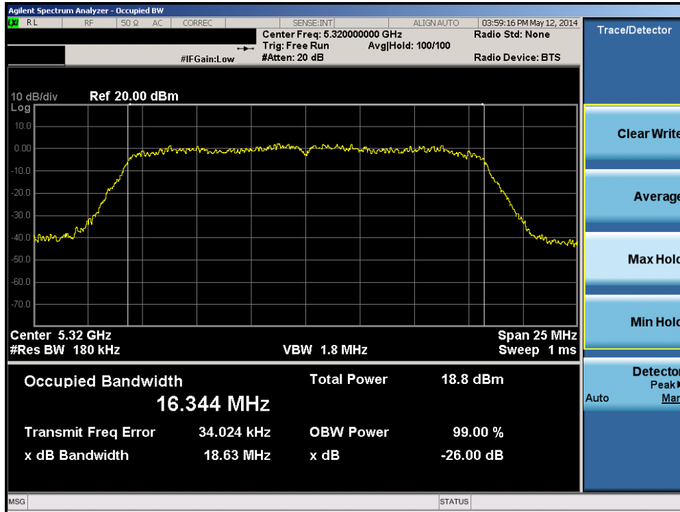
Plot 6-9. 26dB Bandwidth Plot (802.11a (UNII Band 2A) – Ch. 64)
