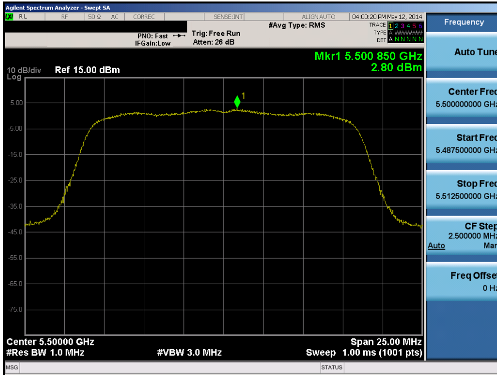
Plot 6-34. Peak Power Spectral Density Plot (802.11a (UNII Band 2C) – Ch. 100)
