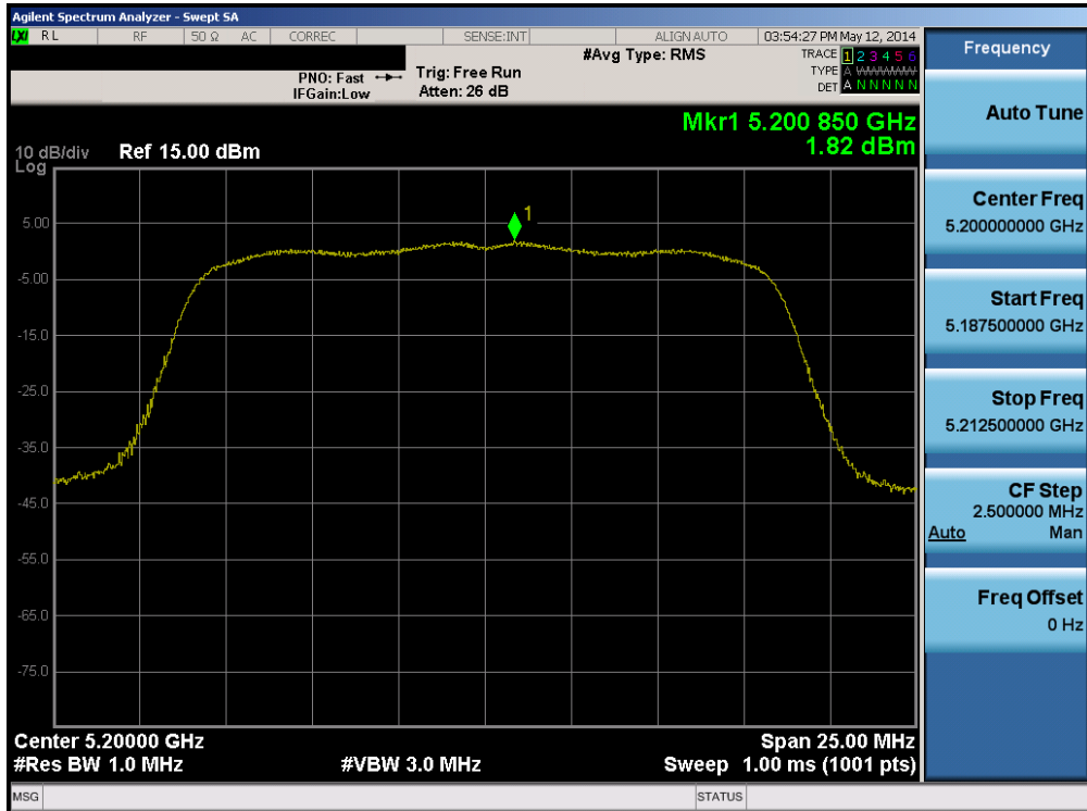
Plot 6-23. Peak Power Spectral Density Plot (802.11a (UNII Band 1) – Ch. 40)
