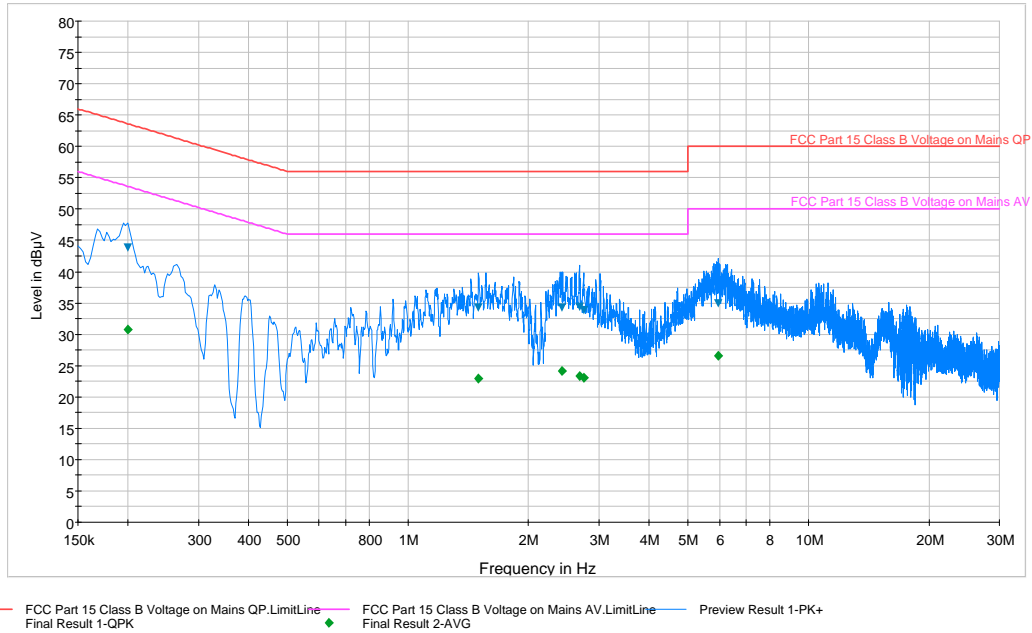
Plot 6-50. Line Conducted Plot with 802.11a UNII Band 1 (N)
