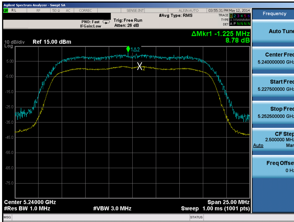
Plot 6-40. Peak Excursion Ratio Plot (802.11a (UNII Band 1) – Ch. 48)
