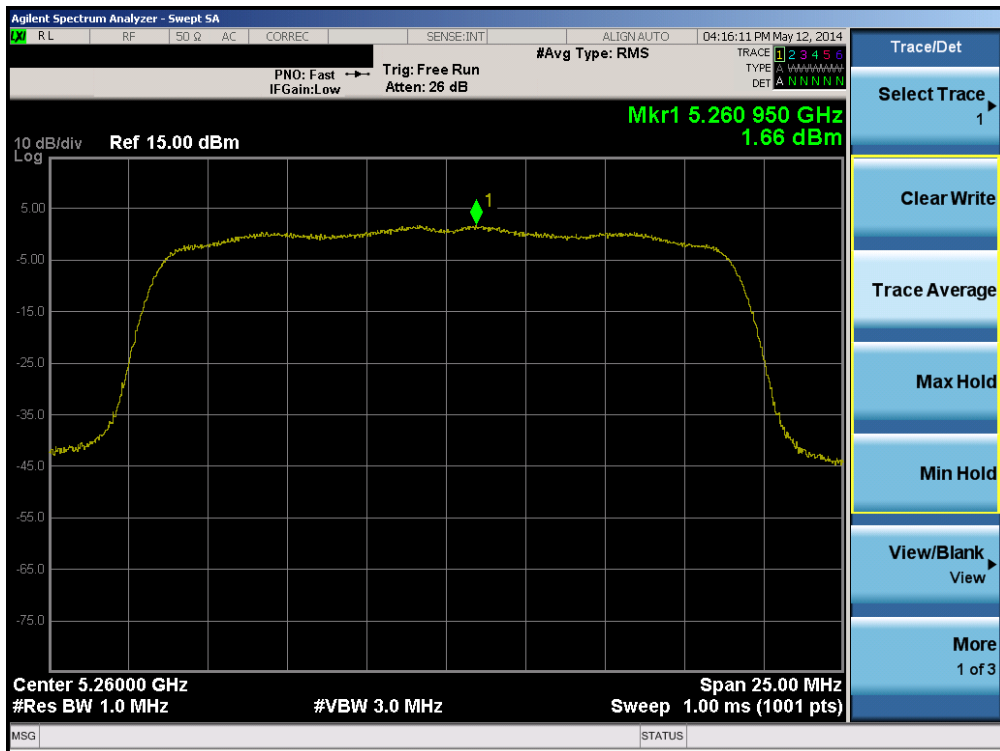
Plot 6-31. Peak Power Spectral Density Plot (20MHz BW 802.11n (UNII Band 2A) – Ch. 52)
