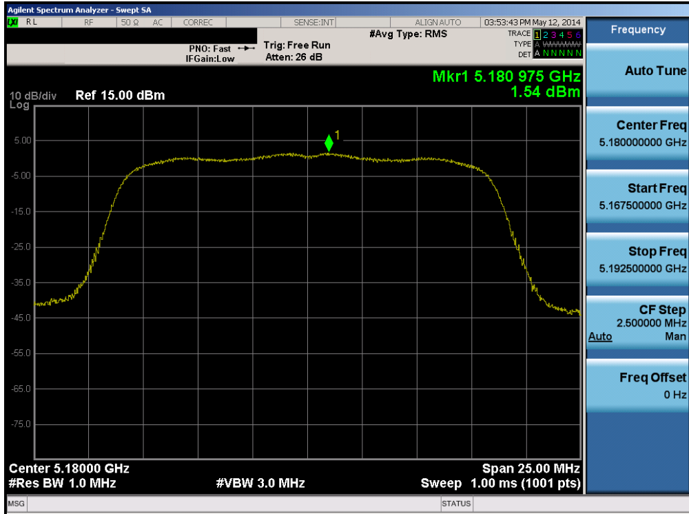
Plot 6-22. Peak Power Spectral Density Plot (802.11a (UNII Band 1) – Ch. 36)
