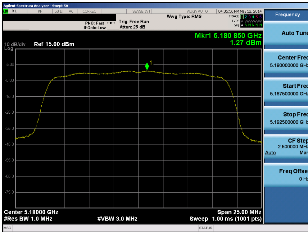
Plot 6-25. Peak Power Spectral Density Plot (20MHz BW 802.11n (UNII Band 1) – Ch. 36)
