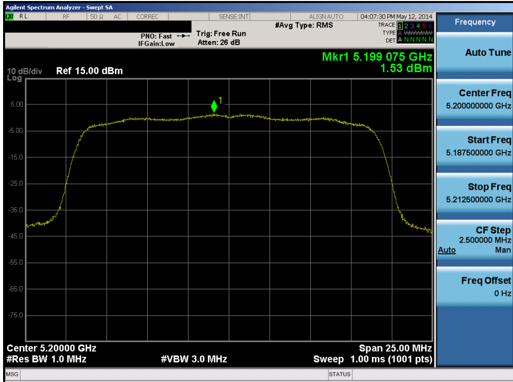
Plot 6-26. Peak Power Spectral Density Plot (20MHz BW 802.11n (UNII Band 1) – Ch. 40)
