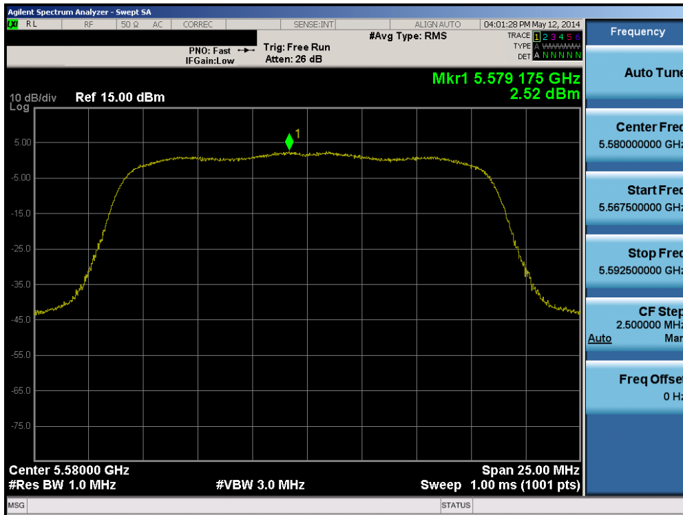
Plot 6-35. Peak Power Spectral Density Plot (802.11a (UNII Band 2C) – Ch. 116)
