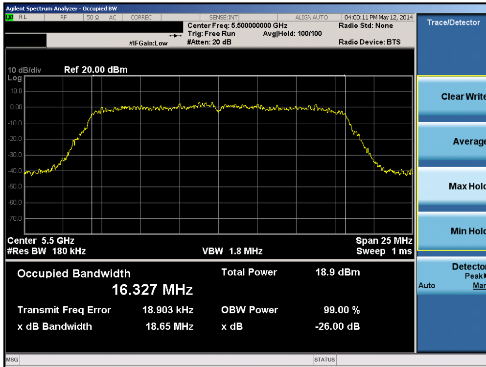
Plot 6-13. 26dB Bandwidth Plot (802.11a (UNII Band 2C) – Ch. 100)
