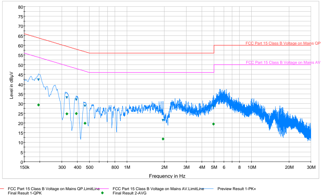
Plot 6-53. Line Conducted Plot with 802.11a UNII Band 2C (L1)
