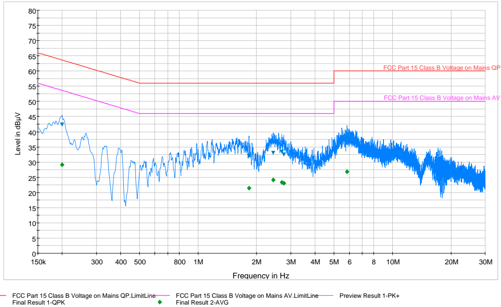
Plot 6-54. Line Conducted Plot with 802.11a UNII Band 2C (N)
