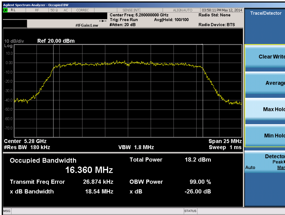
Plot 6-8. 26dB Bandwidth Plot (802.11a (UNII Band 2A) – Ch. 56)
