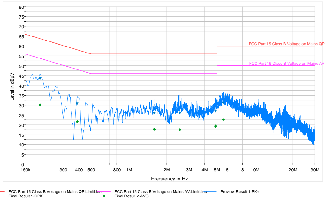
Plot 6-51. Line Conducted Plot with 802.11a UNII Band 2A (L1)
