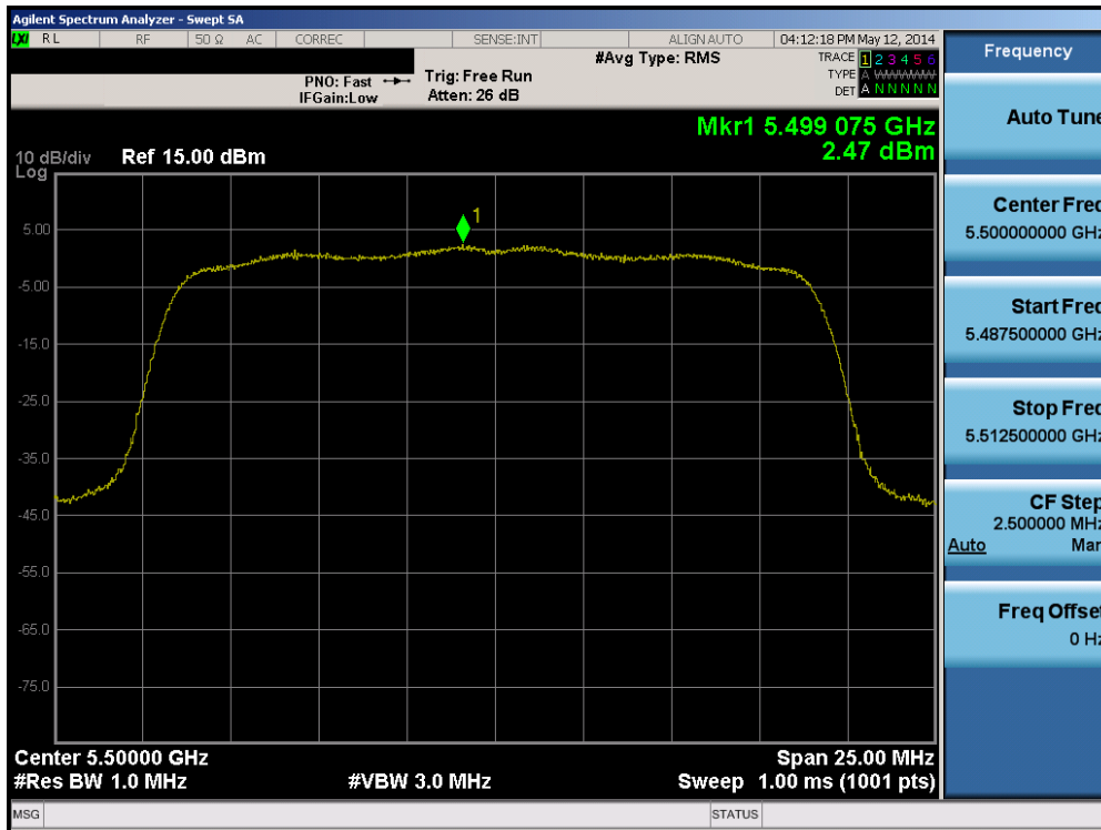
Plot 6-37. Peak Power Spectral Density Plot (20MHz BW 802.11n (UNII Band 2C) – Ch. 100)
