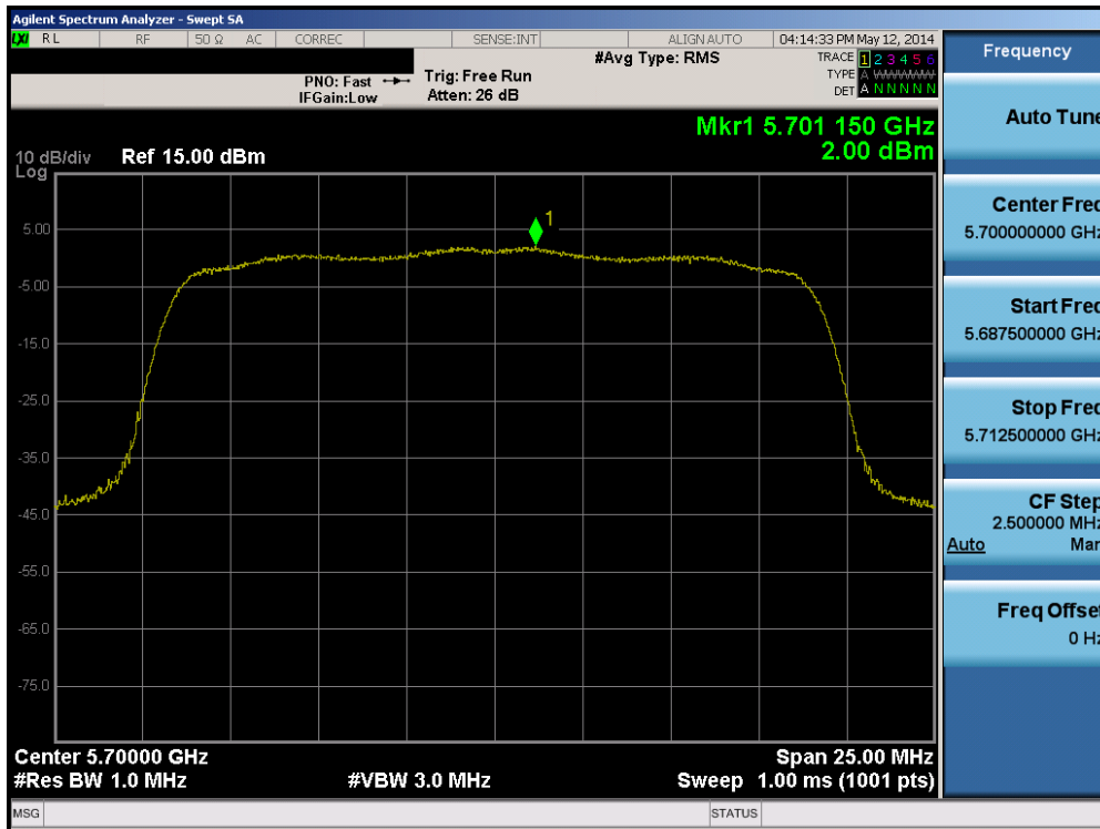
Plot 6-39. Peak Power Spectral Density Plot (20MHz BW 802.11n (UNII Band 2C) – Ch. 140)
