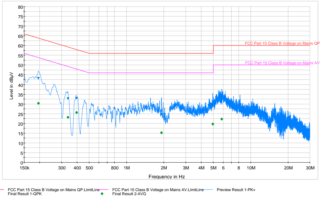
Plot 6-49. Line Conducted Plot with 802.11a UNII Band 1 (L1)
