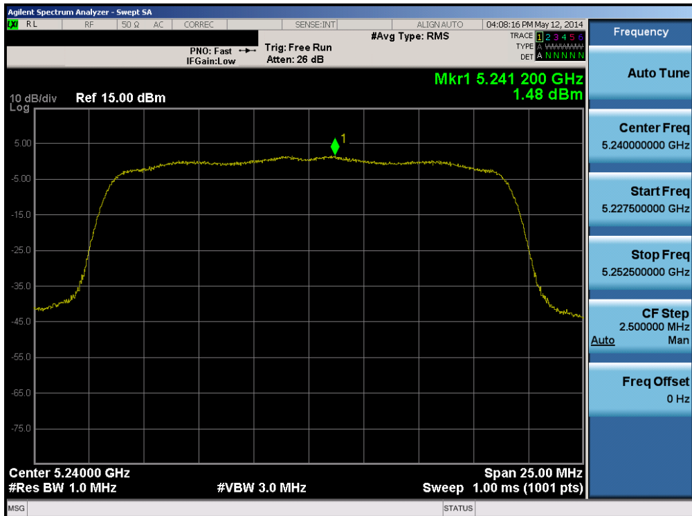
Plot 6-27. Peak Power Spectral Density Plot (20MHz BW 802.11n (UNII Band 1) – Ch. 48)
