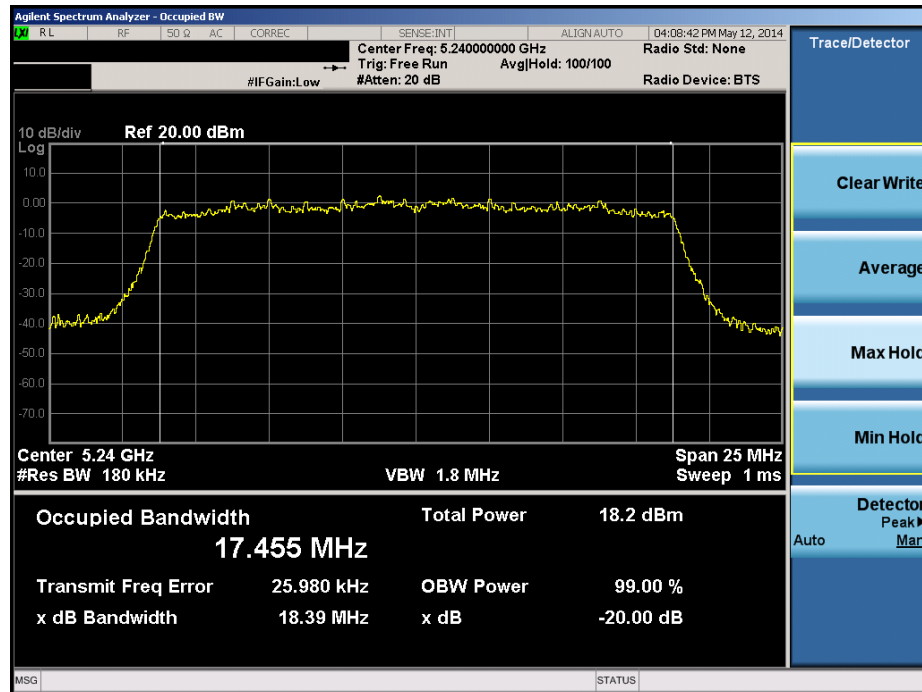
Plot 6-20. 20dB Bandwidth Plot (20MHz BW 802.11n (UNII Band 1) – Ch. 48)
