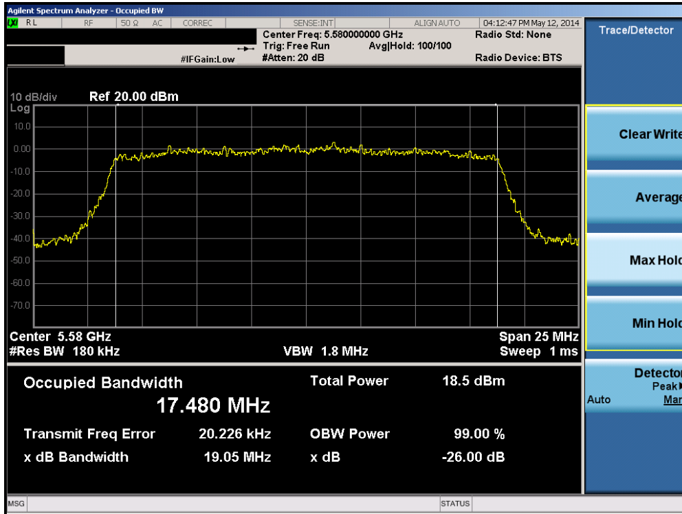
Plot 6-17. 26dB Bandwidth Plot (20MHz BW 802.11n (UNII Band 2C) – Ch. 116)
