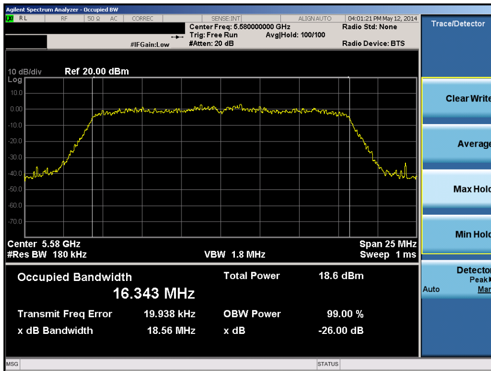
Plot 6-14. 26dB Bandwidth Plot (802.11a (UNII Band 2C) – Ch. 116)
