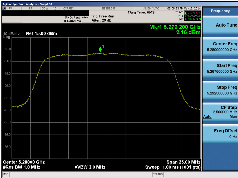
Plot 6-29. Peak Power Spectral Density Plot (802.11a (UNII Band 2A) – Ch. 56)
