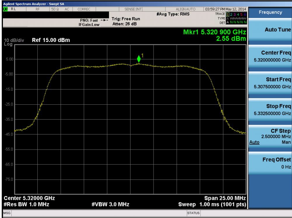
Plot 6-30. Peak Power Spectral Density Plot (802.11a (UNII Band 2A) – Ch. 64)
