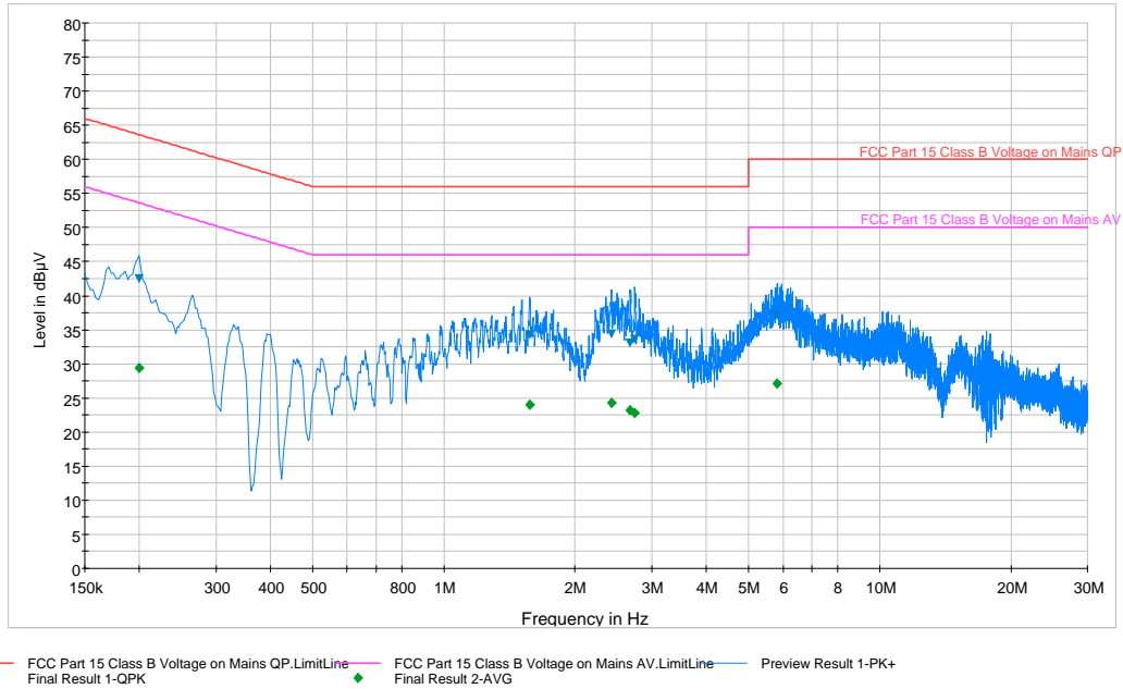
Plot 6-52. Line Conducted Plot with 802.11a UNII Band 2A (N)
