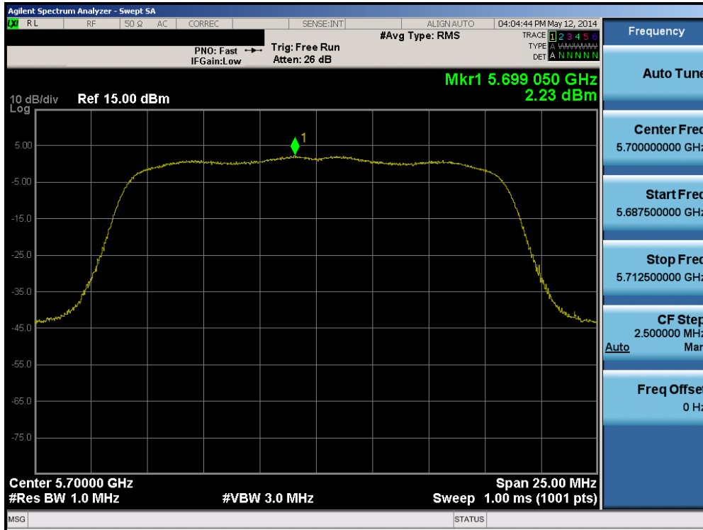
Plot 6-36. Peak Power Spectral Density Plot (802.11a (UNII Band 2C) – Ch. 140)
