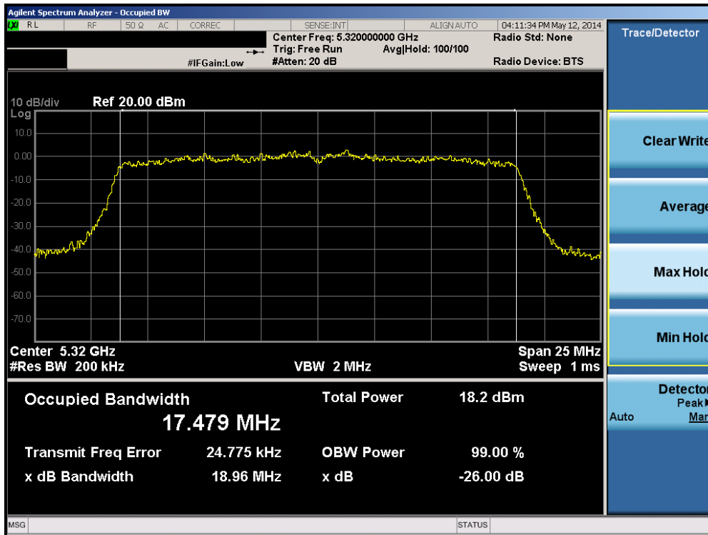
Plot 6-12. 26dB Bandwidth Plot (20MHz BW 802.11n (UNII Band 2A) – Ch. 64)
