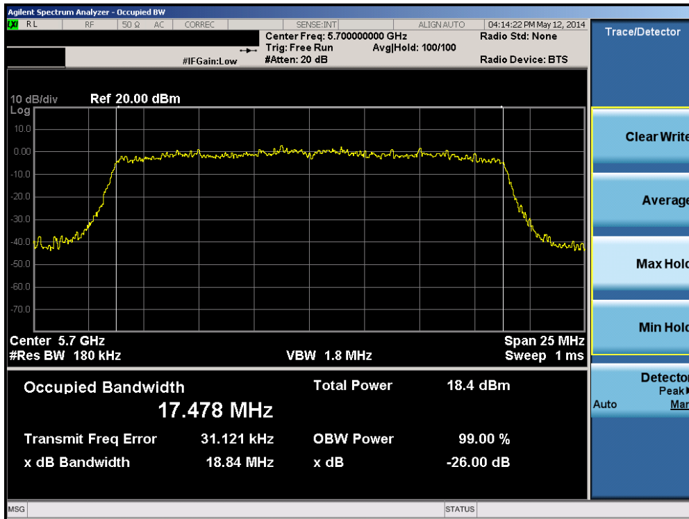
Plot 6-18. 26dB Bandwidth Plot (20MHz BW 802.11n (UNII Band 2C) – Ch. 140)
