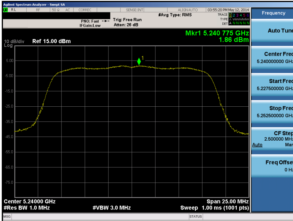
Plot 6-24. Peak Power Spectral Density Plot (802.11a (UNII Band 1) – Ch. 48)
