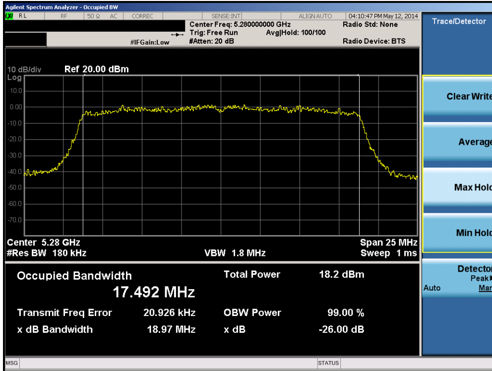
Plot 6-11. 26dB Bandwidth Plot (20MHz BW 802.11n (UNII Band 2A) – Ch. 56)
