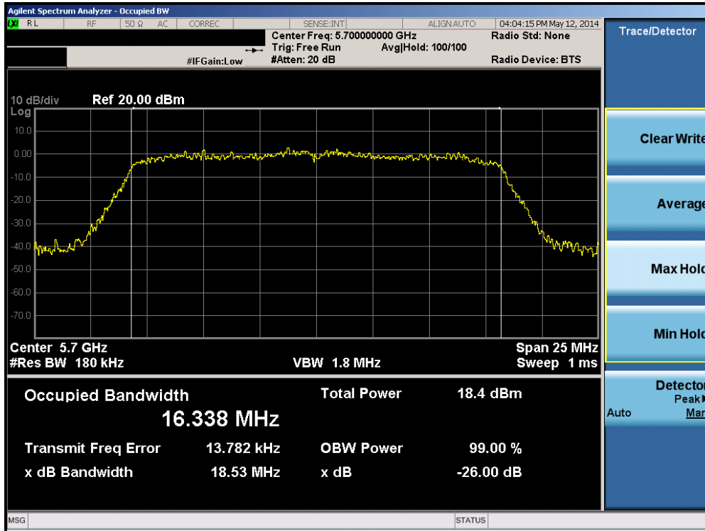
Plot 6-15. 26dB Bandwidth Plot (802.11a (UNII Band 2C) – Ch. 140)
