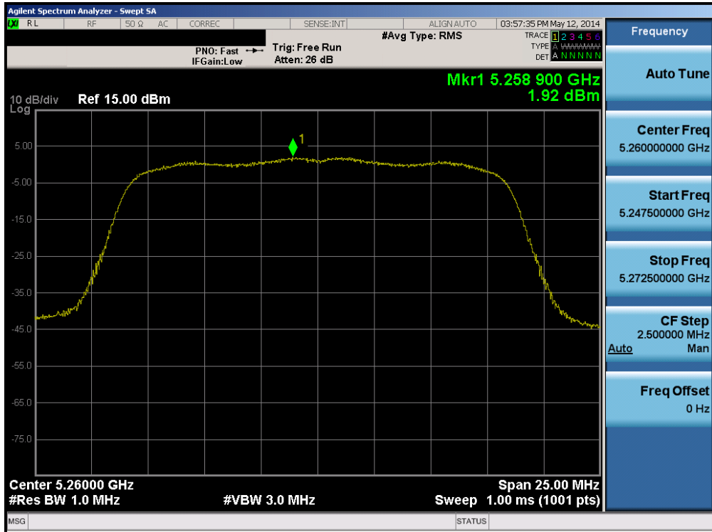
Plot 6-28. Peak Power Spectral Density Plot (802.11a (UNII Band 2A) – Ch. 52)
