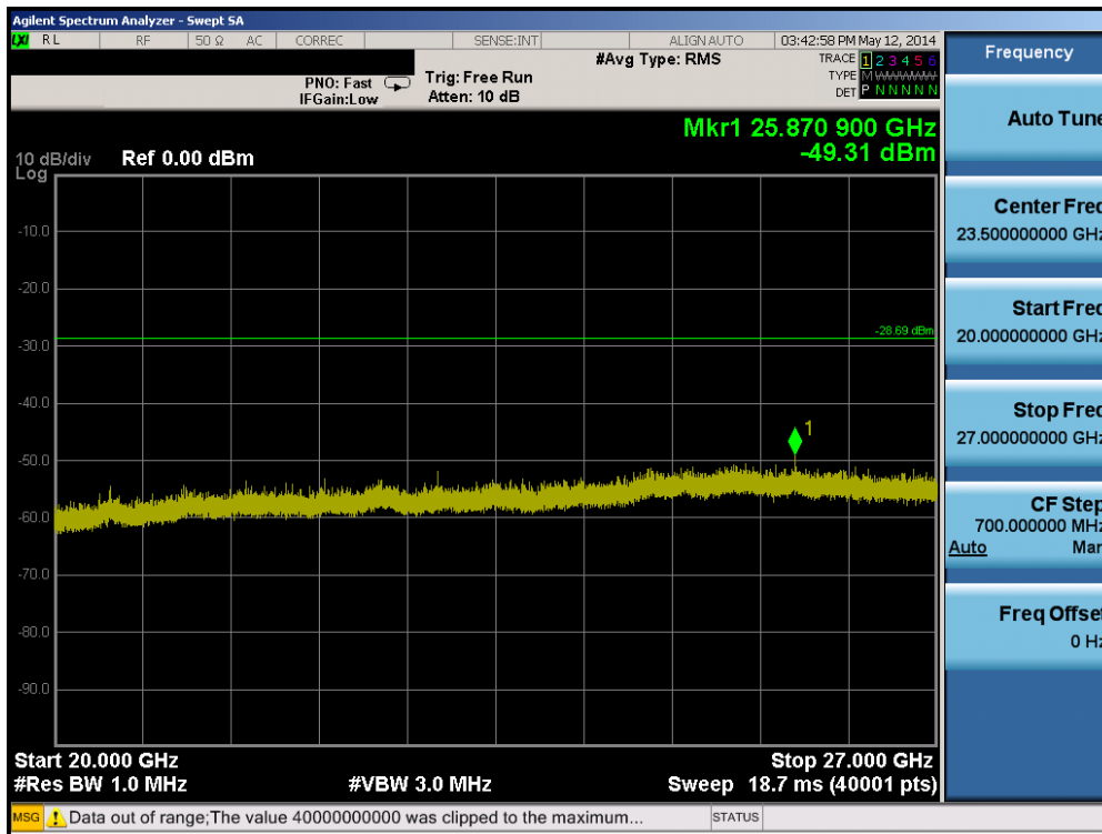
Plot 6-50. Conducted Spurious Plot (802.11a – Ch. 157)
