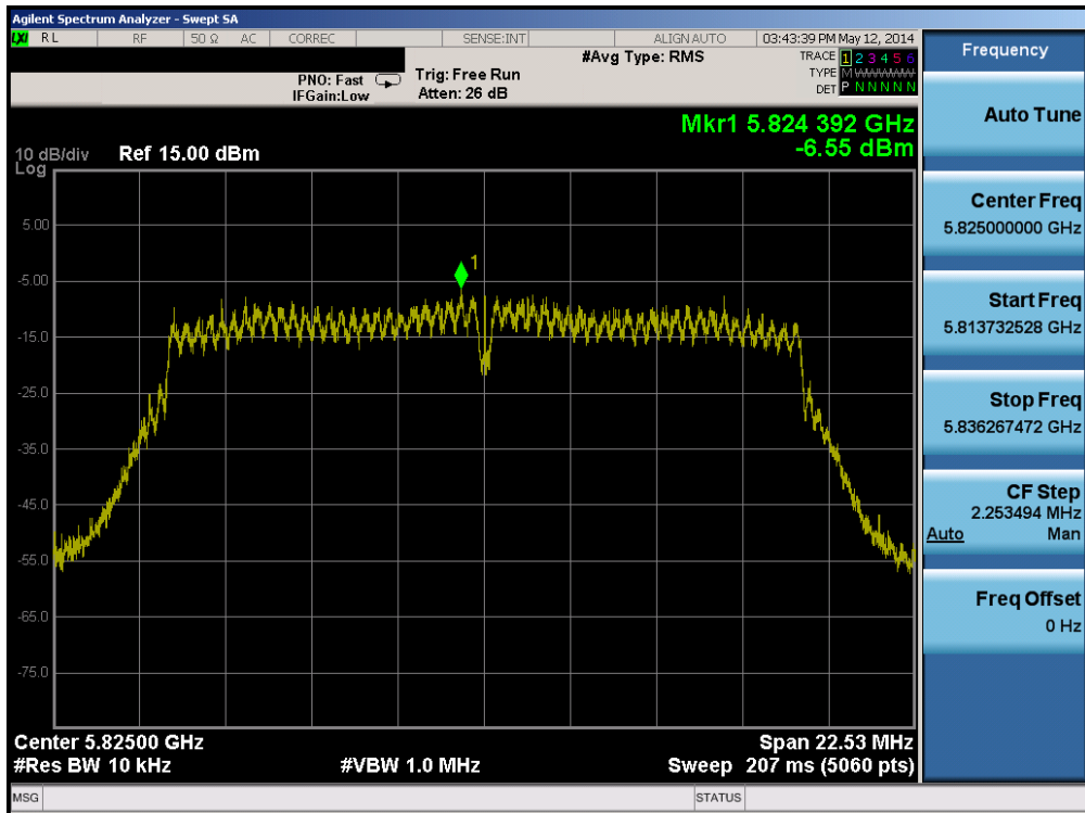
Plot 6-27. Power Spectral Density Plot (802.11a – Ch. 165)
