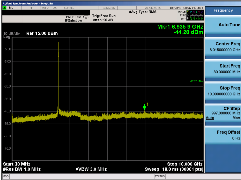
Plot 6-45. Conducted Spurious Plot (802.11b – Ch. 11)
