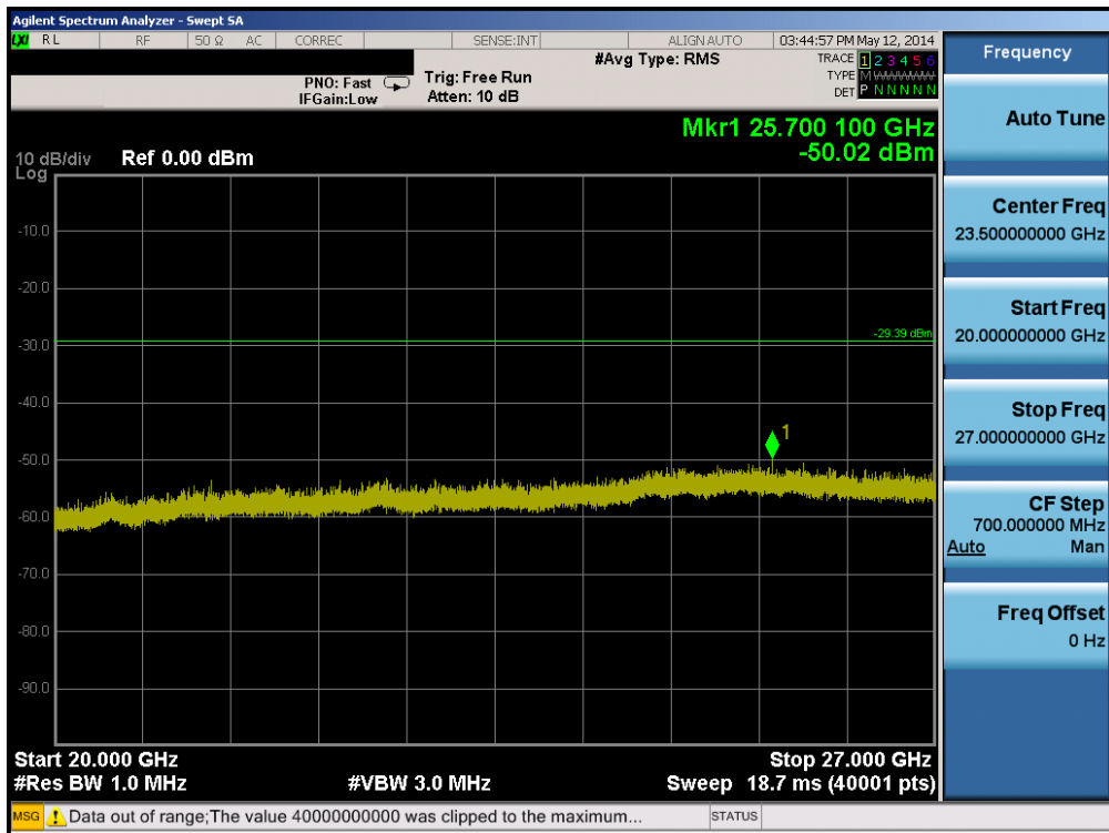
Plot 6-52. Conducted Spurious Plot (802.11a – Ch. 165)
