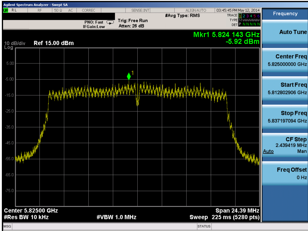
Plot 6-30. Power Spectral Density Plot (20MHz BW 802.11n (5.8GHz) – Ch. 165)
