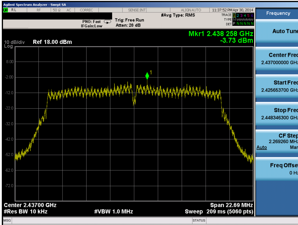
Plot 6-20. Power Spectral Density Plot (802.11g – Ch. 6)
