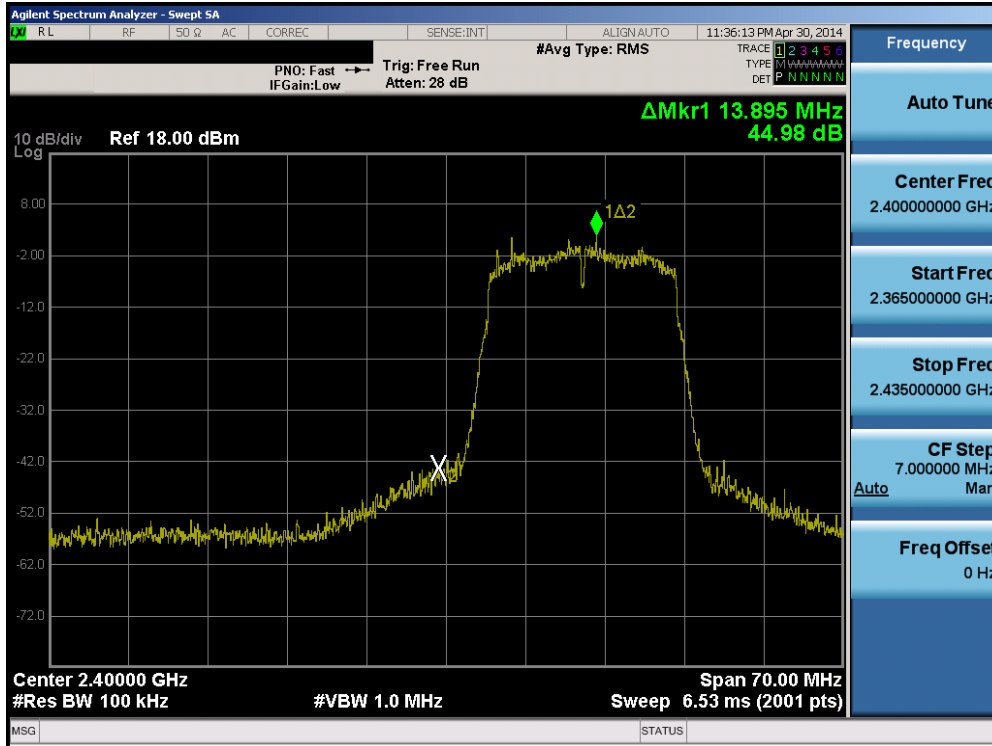
Plot 6-33. Band Edge Plot (802.11g– Ch. 1)
