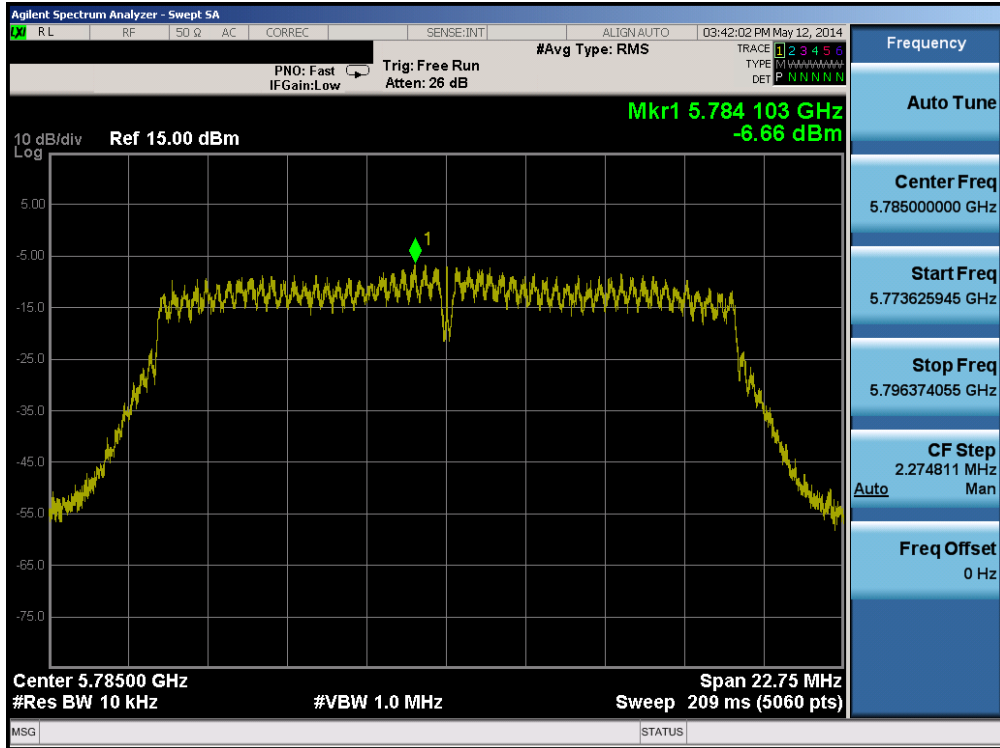
Plot 6-26. Power Spectral Density Plot (802.11a – Ch. 157)
