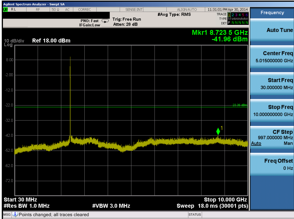
Plot 6-41. Conducted Spurious Plot (802.11b – Ch. 1)
