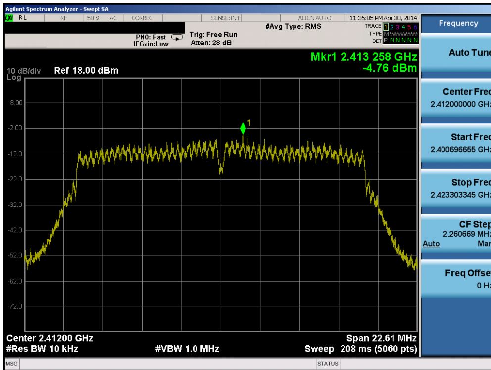
Plot 6-19. Power Spectral Density Plot (802.11g – Ch. 1)
