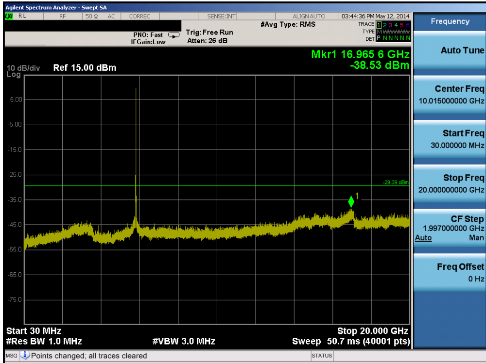
Plot 6-51. Conducted Spurious Plot (802.11a – Ch. 165)
