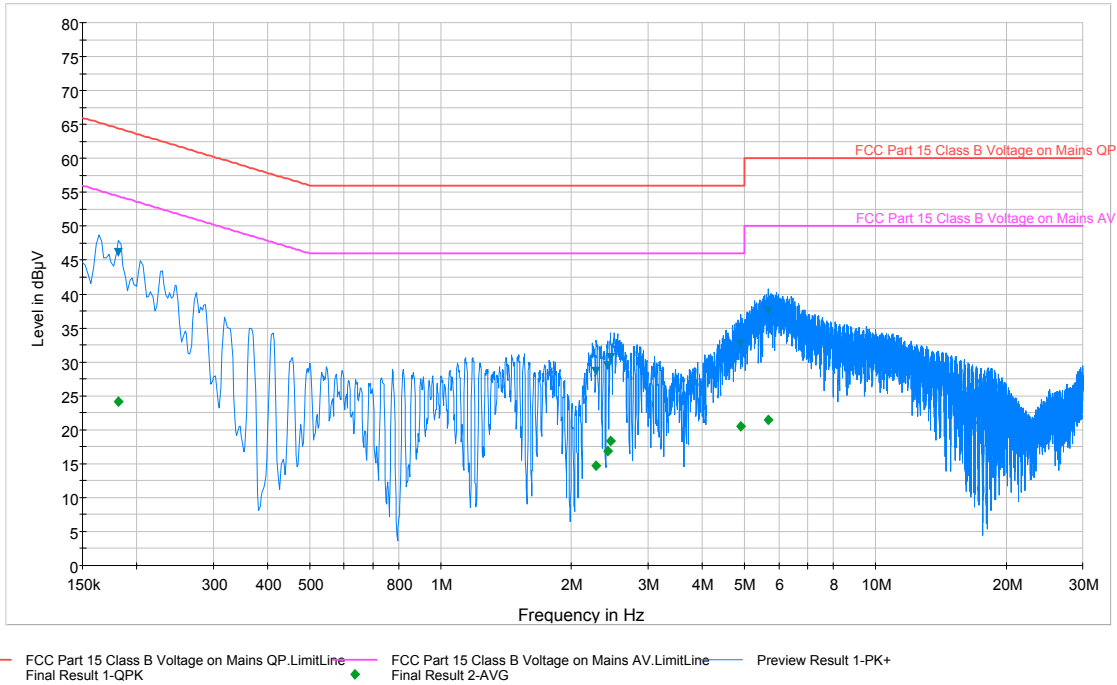
Plot 6-59. Line Conducted Plot with 802.11a (L1)
