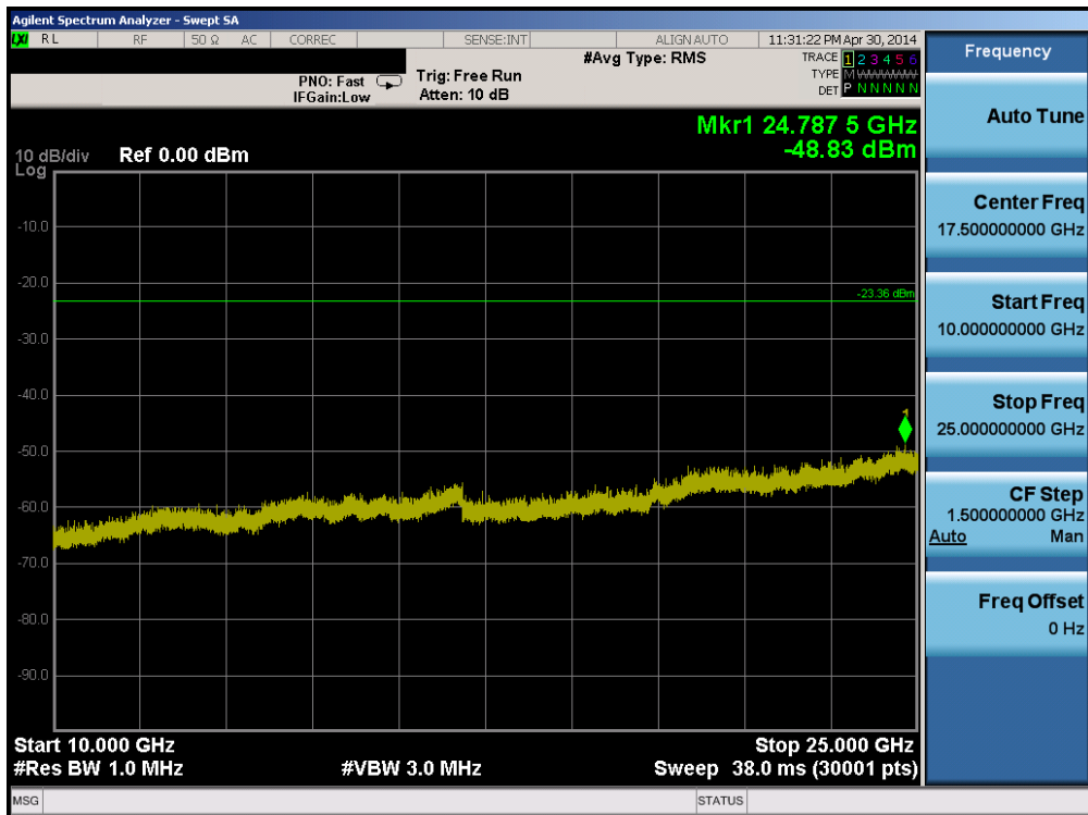
Plot 6-42. Conducted Spurious Plot (802.11b – Ch. 1)
