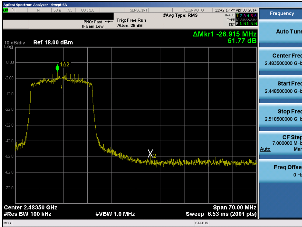
Plot 6-36. Band Edge Plot (802.11n (2.4GHz) – Ch. 11)
