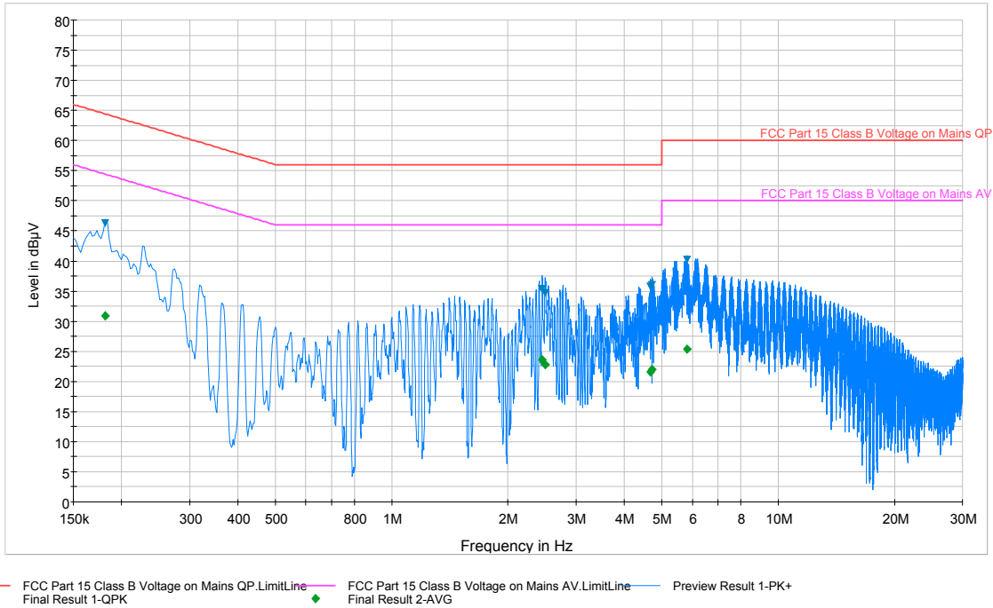
Plot 6-58. Line Conducted Plot with 802.11b (N)
