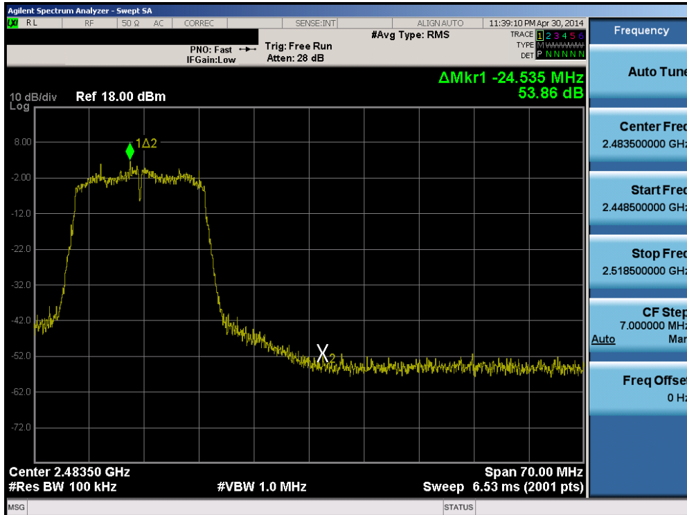
Plot 6-34. Band Edge Plot (802.11g – Ch. 11)
