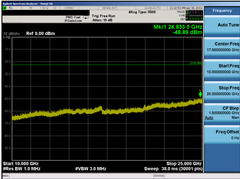
Plot 6-44. Conducted Spurious Plot (802.11b – Ch. 6)
