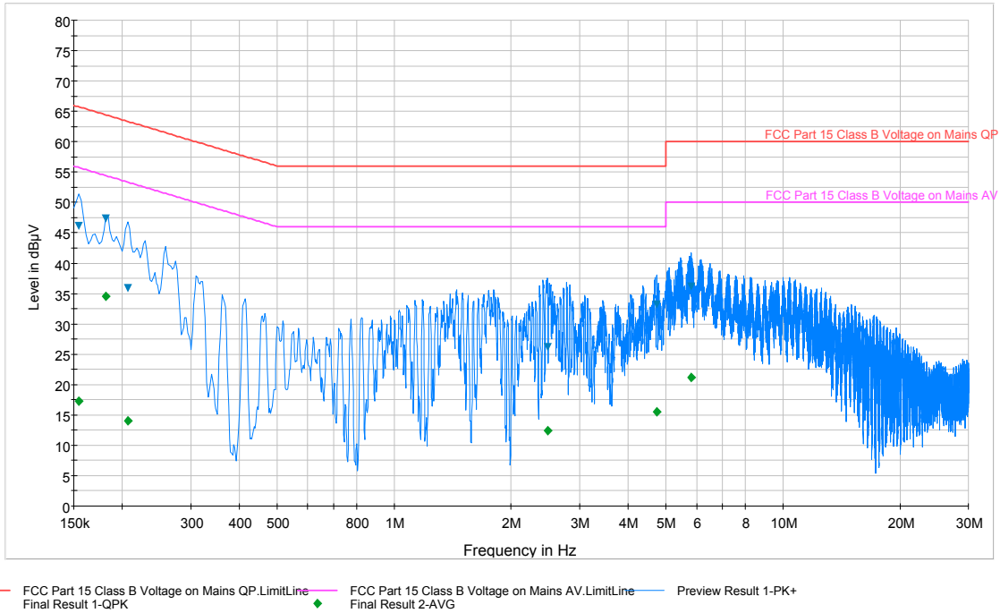
Plot 6-60. Line Conducted Plot with 802.11a (N)
