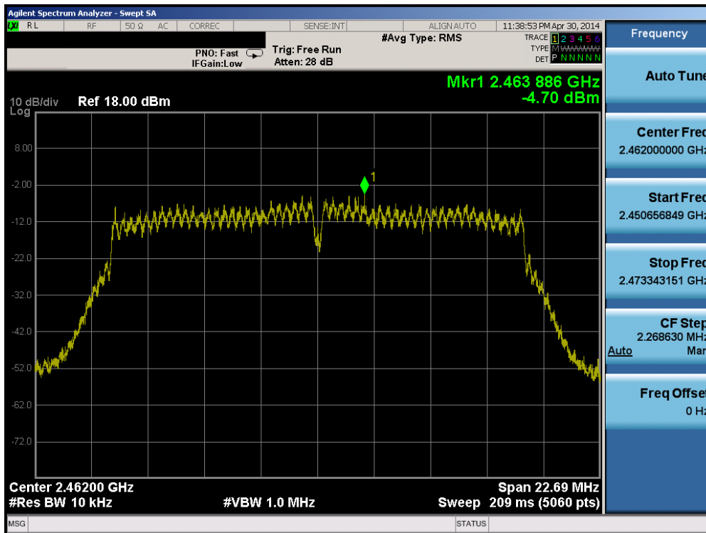
Plot 6-21. Power Spectral Density Plot (802.11g – Ch. 11)
