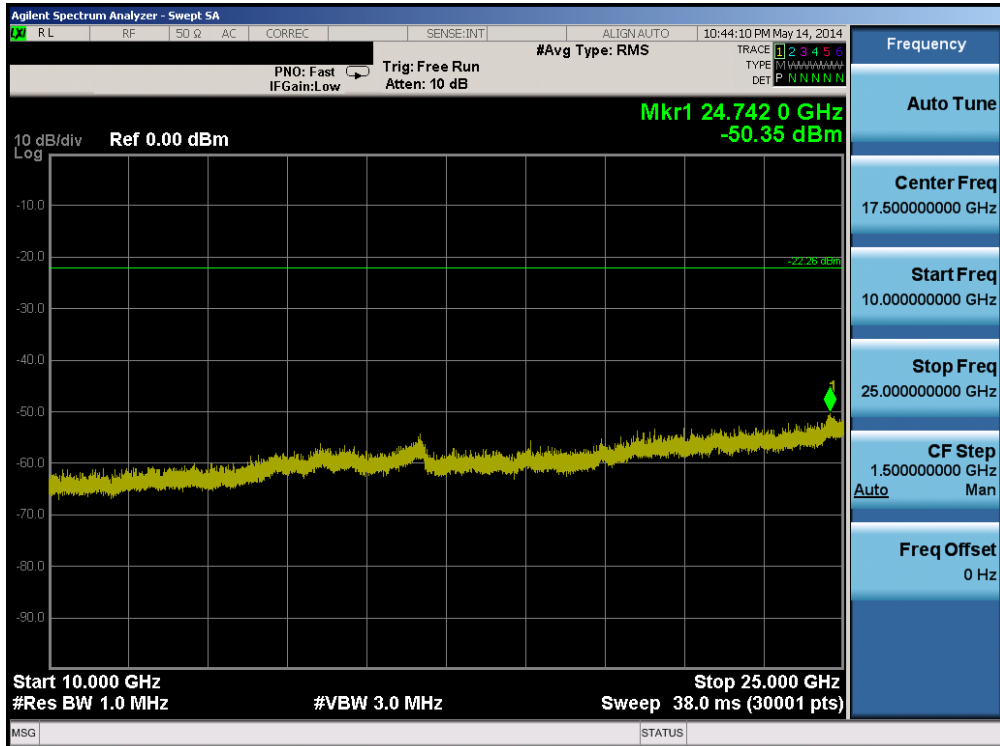
Plot 6-46. Conducted Spurious Plot (802.11b – Ch. 11)
