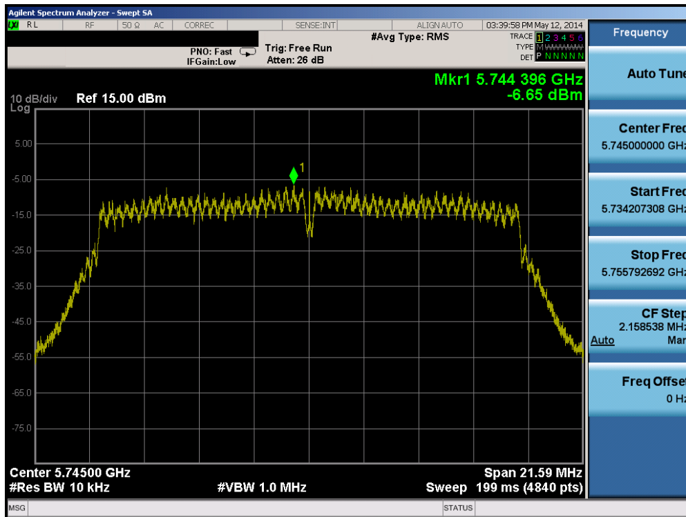
Plot 6-25. Power Spectral Density Plot (802.11a – Ch. 149)
