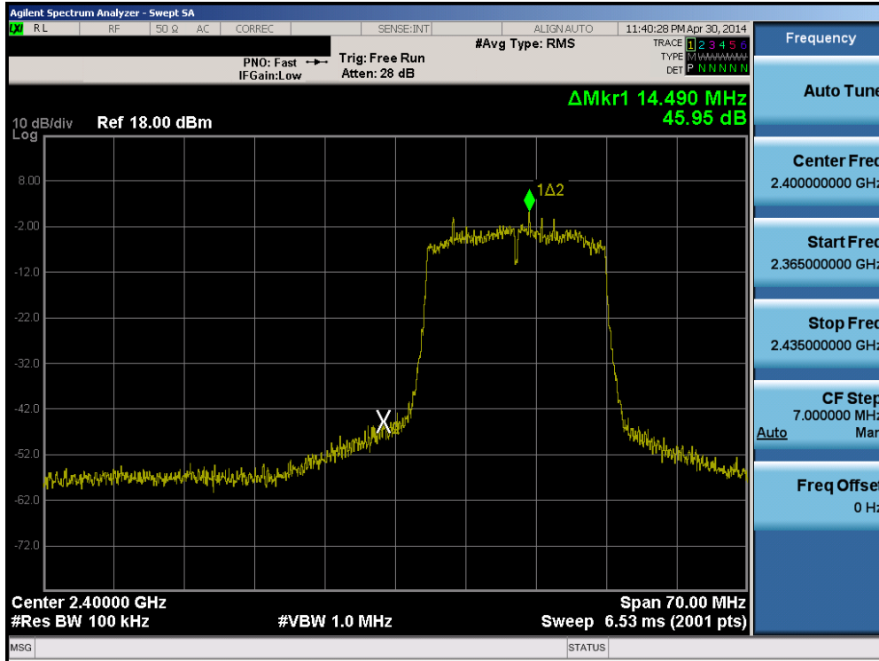
Plot 6-35. Band Edge Plot (802.11n (2.4GHz) – Ch. 1)
