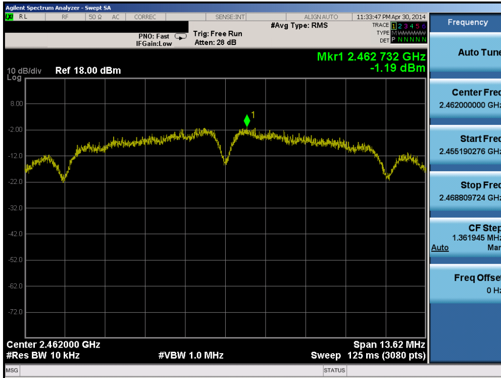
Plot 6-18. Power Spectral Density Plot (802.11b – Ch. 11)
