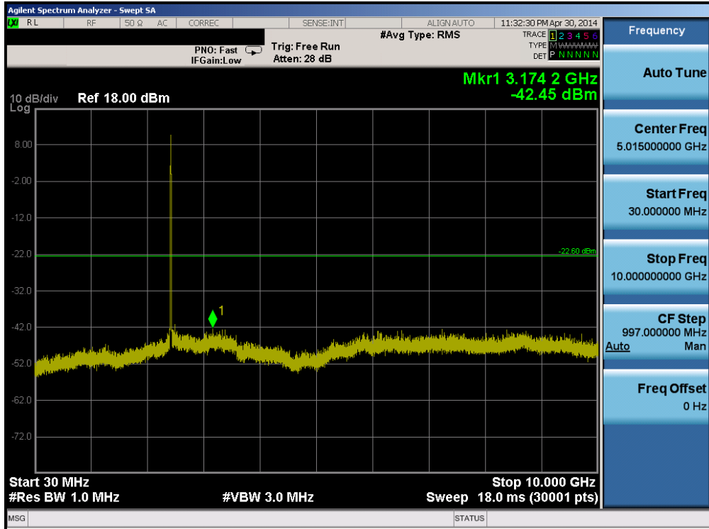
Plot 6-43. Conducted Spurious Plot (802.11b – Ch. 6)
