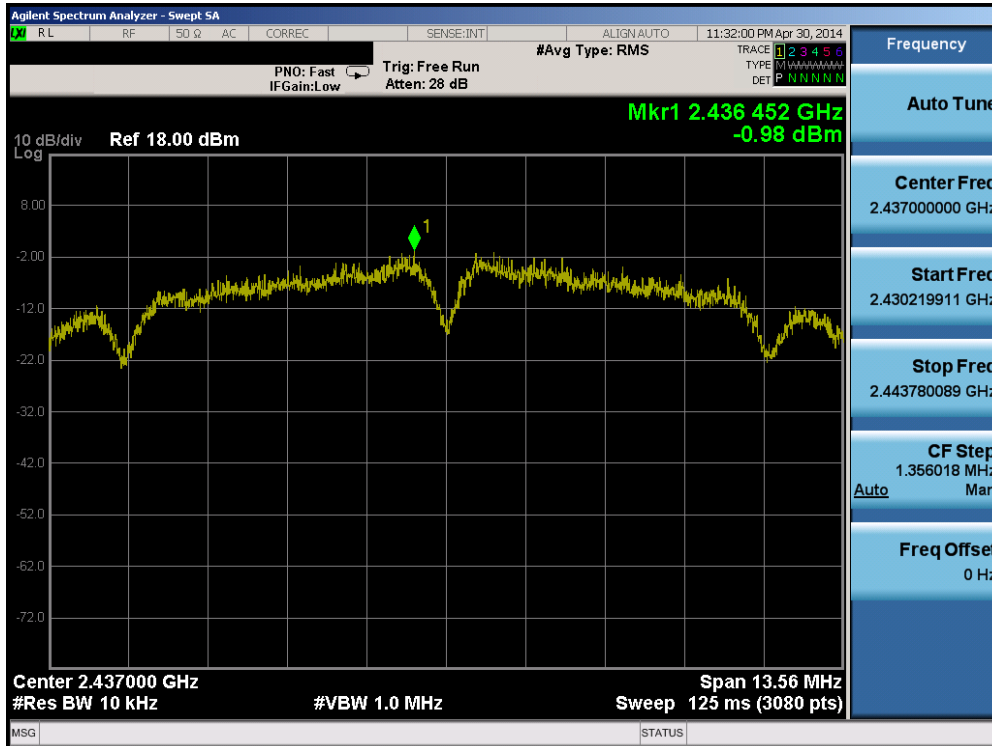
Plot 6-17. Power Spectral Density Plot (802.11b – Ch. 6)
