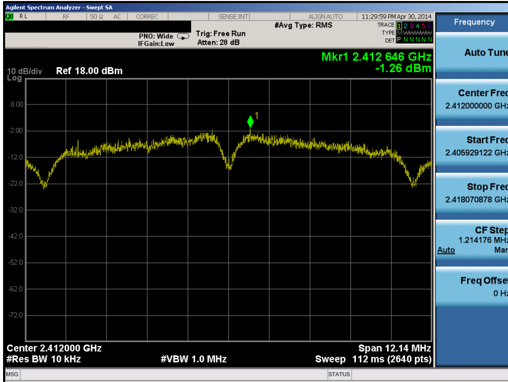
Plot 6-16. Power Spectral Density Plot (802.11b – Ch. 1)
