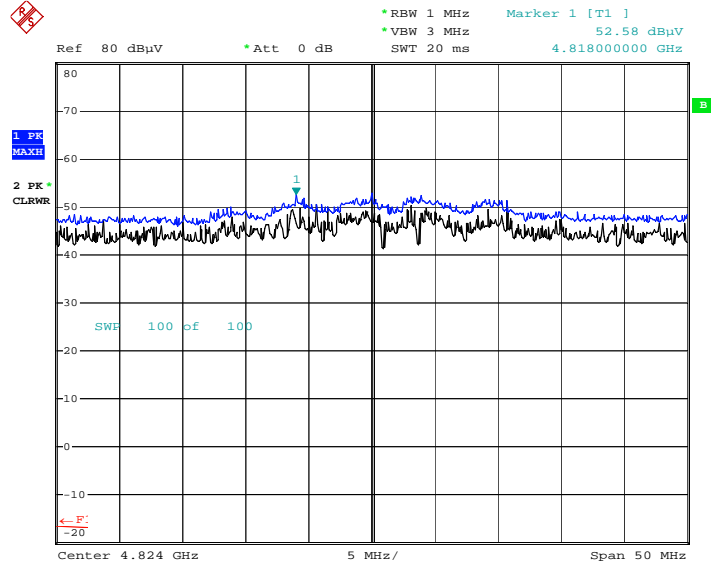
Radiated Spurious Emissions plot – Peak Reading (802.11g, Ch.1 2nd Harmonic, H)
