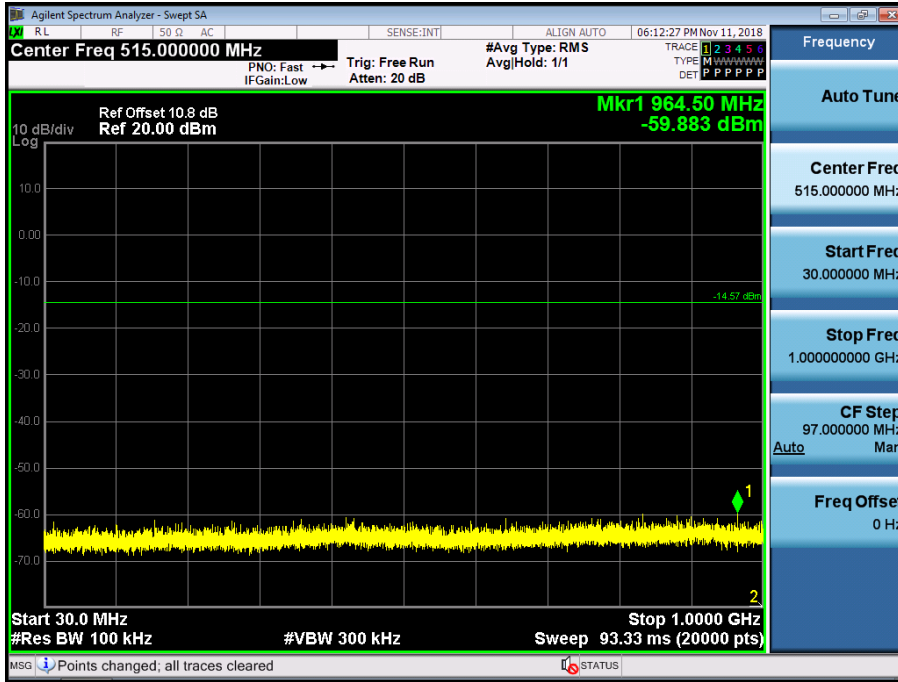
Conducted Spurious Emission (802.11g_Ch.11)
