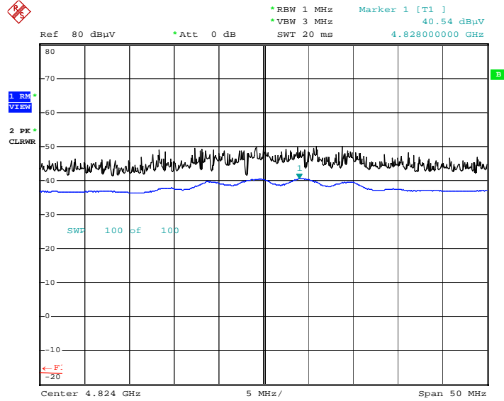
Radiated Spurious Emissions plot – Average Reading (802.11g, Ch.1 2nd Harmonic, H)
