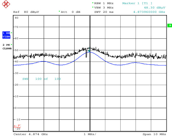
Radiated Spurious Emissions plot – Average Reading (802.11b, Ch.6 2nd Harmonic, H)
