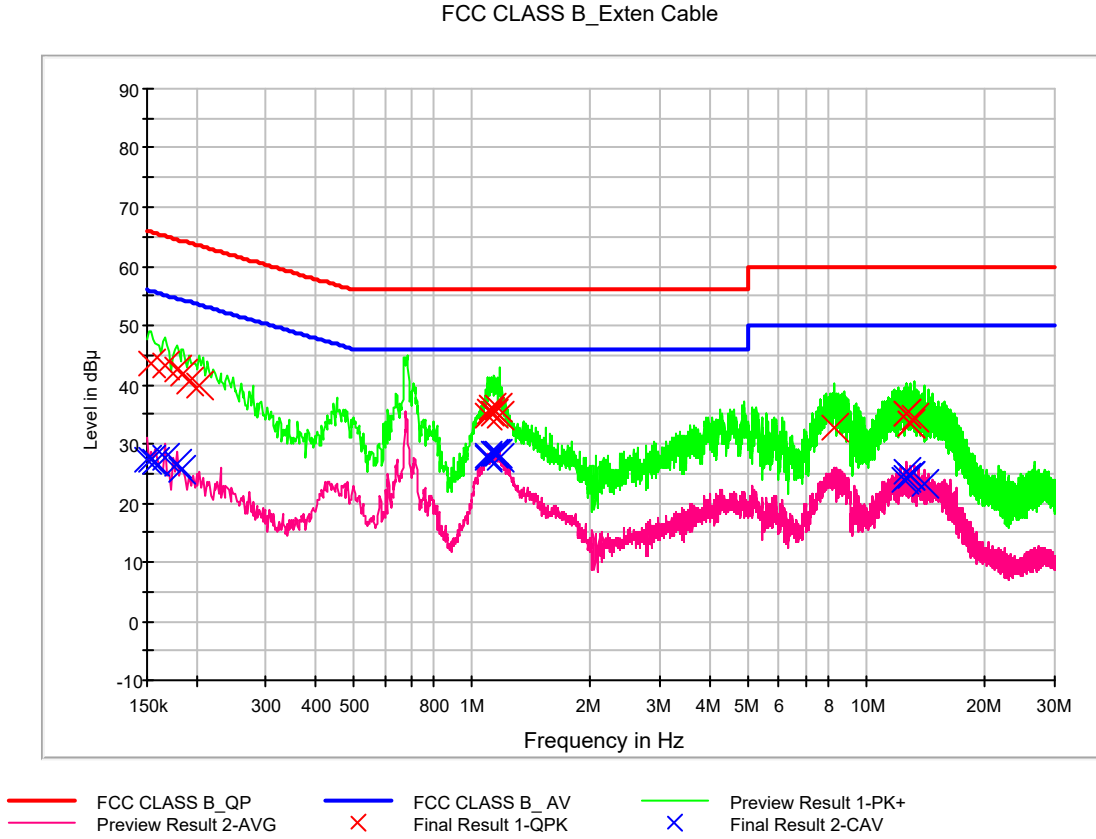
Figure 5: Conducted Emission, SD Card Write & FM Radio (Middle CH) Mode, Line (L1)
