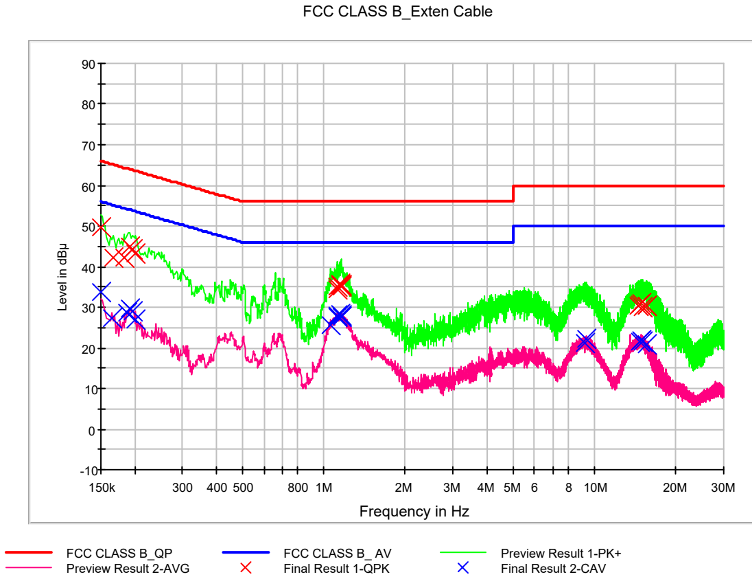
Figure 8: Conducted Emission, Receiver Mode at LTE B17 (Middle CH Idle), Line (L1)
