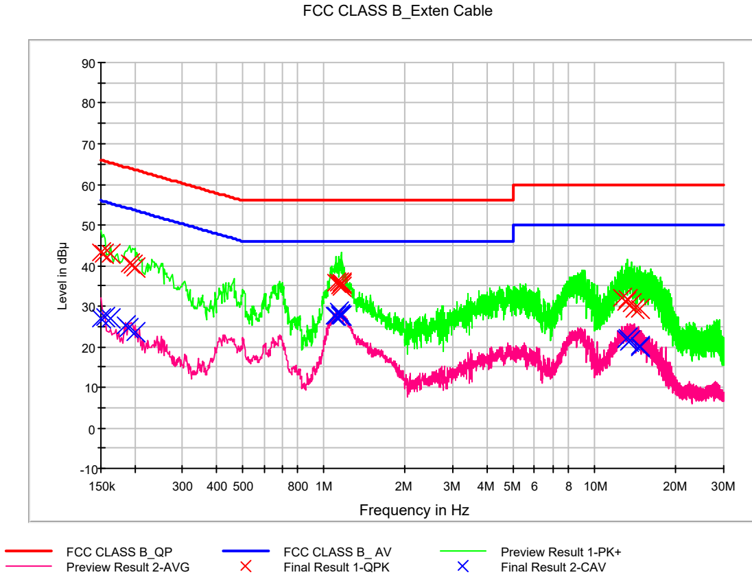
Figure 6: Conducted Emission, SD Card Write & FM Radio (Middle CH) Mode, Line (N)
