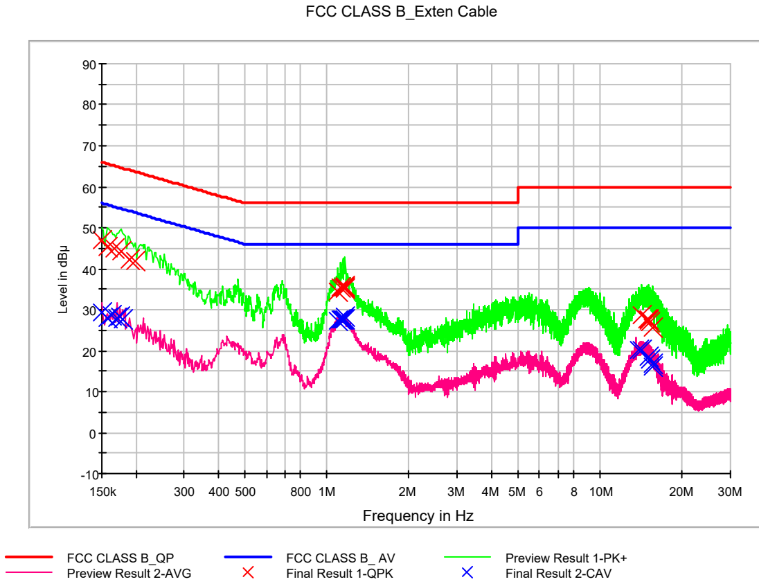
Figure 10: Conducted Emission, Receiver Mode at WCDMA 850, LTE B5/B26 (Middle CH Idle), Line (L1)
