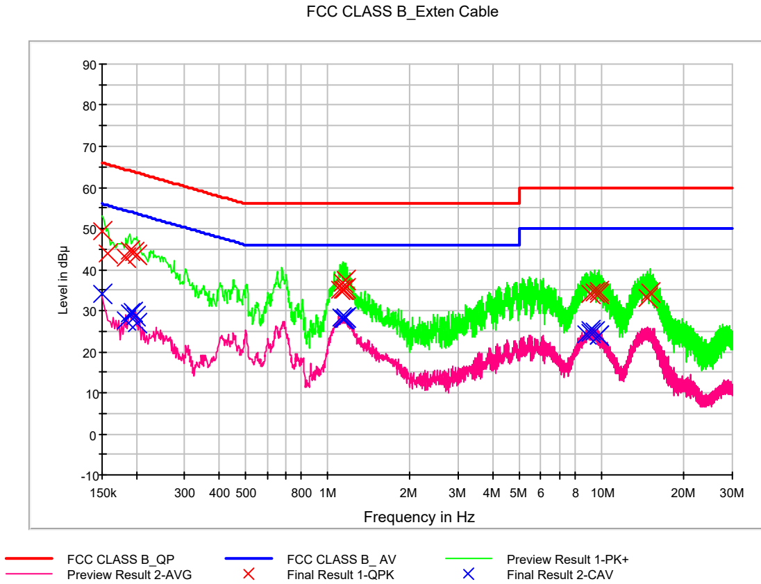
Figure 9: Conducted Emission, Receiver Mode at WCDMA 850, LTE B5/B26 (Middle CH Idle), Line (L1)
