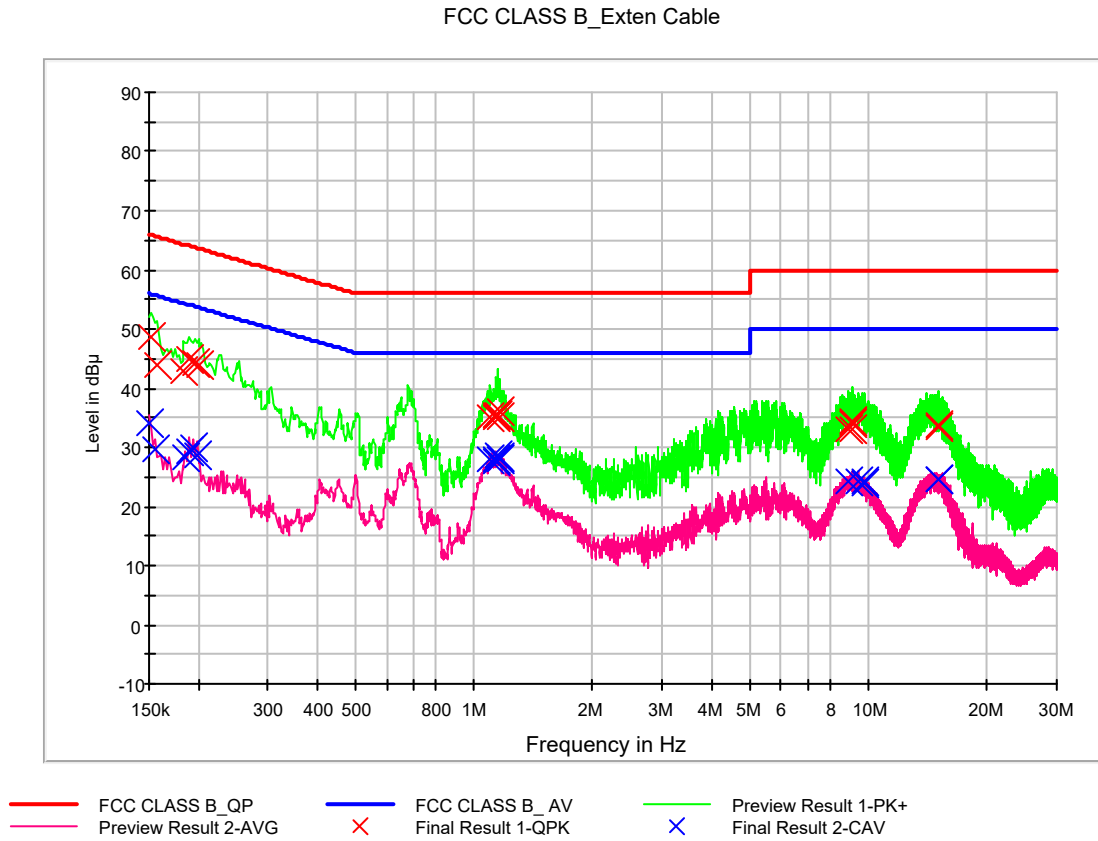
Figure 7: Conducted Emission, Receiver Mode at LTE B17 (Middle CH Idle), Line (L1)
