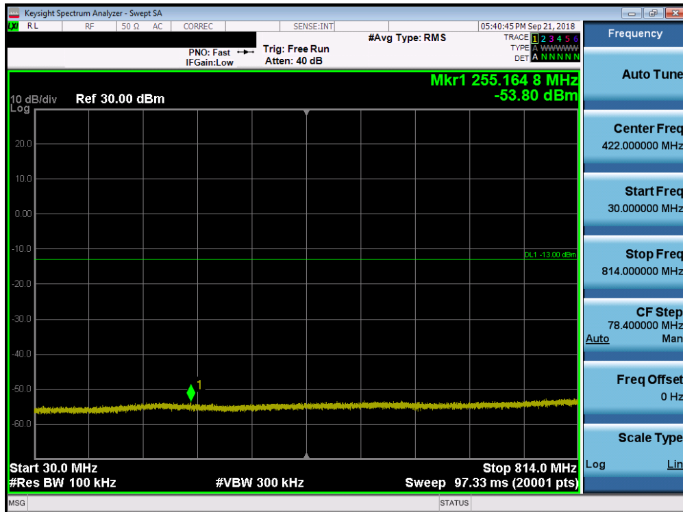
Plot 7-19. Conducted Spurious Plot (LTE Band 26, 1.4MHz QPSK – RB Size 1, RB Offset 0 – High Channel)
