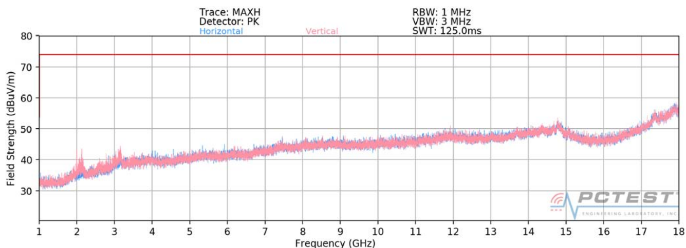
Plot 7-2. Radiated Spurious Plot above 1GHz
