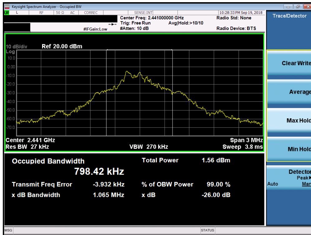
Plot 7-1. Occupied Bandwidth Plot (ANT+ – Ch. 39)
