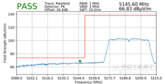
Plot 7-228. Radiated Lower Band Edge Plot MIMO (Peak – UNII Band 1)
