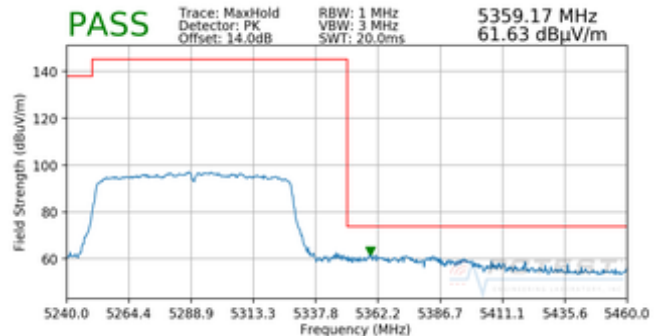
Plot 7-210. Radiated Upper Band Edge Plot SISO ANT2 (Peak – UNII Band 2A)
