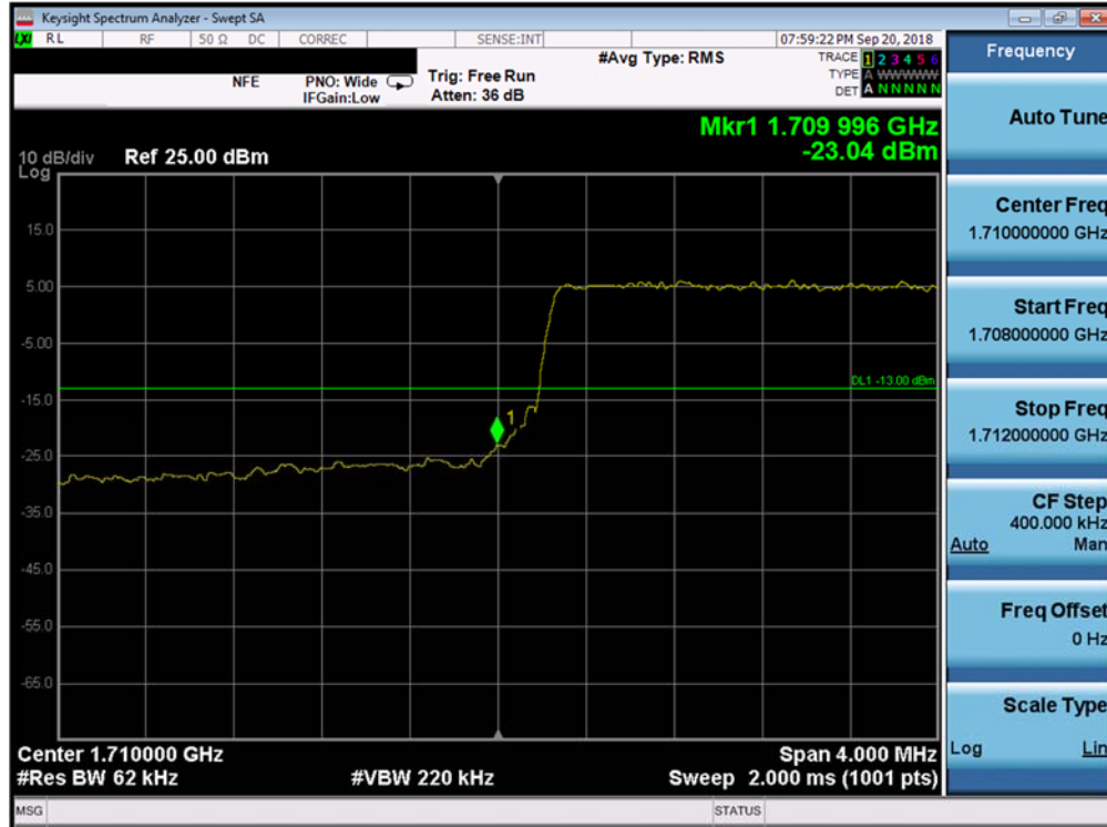
Plot 7-117. Lower Band Edge Plot (Band 4 - 5.0MHz QPSK - Full RB Configuration)
