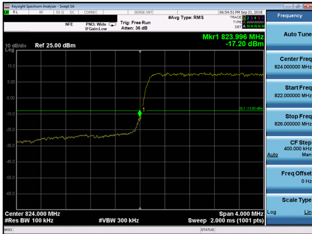
Plot 7-103. Lower Band Edge Plot (Band 5 - 3.0MHz QPSK - Full RB Configuration)
