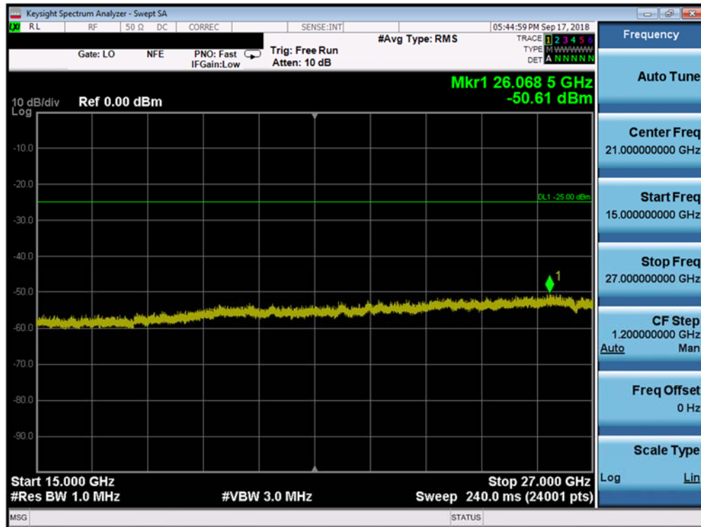
Plot 7-90. Conducted Spurious Plot (Band 41 - 20.0MHz QPSK - RB Size 1, RB Offset 0 - High Channel)
