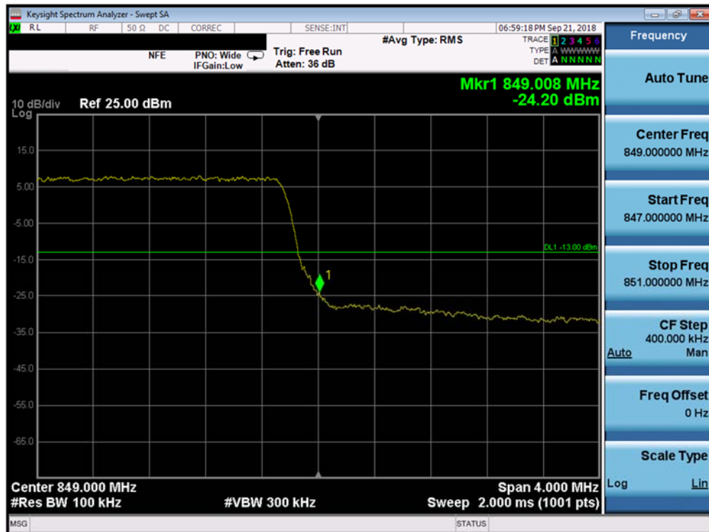
Plot 7-106. Upper Band Edge Plot (Band 5 - 5.0MHz QPSK - Full RB Configuration)
