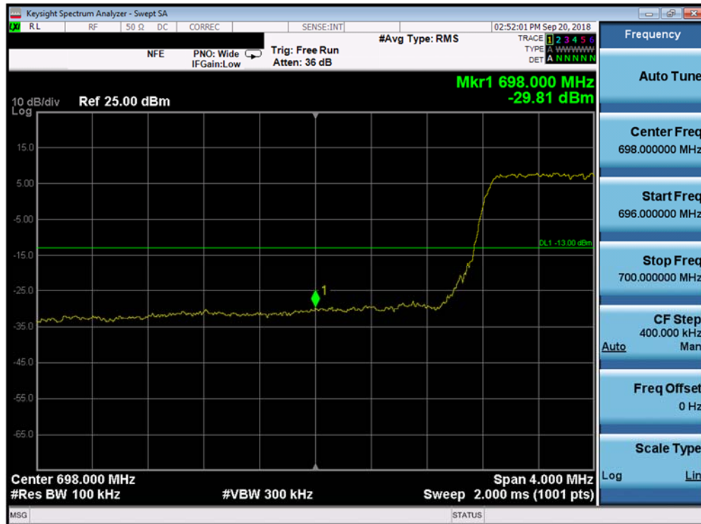
Plot 7-95. Lower Band Edge Plot (Band 12 - 5.0MHz QPSK - Full RB Configuration)
