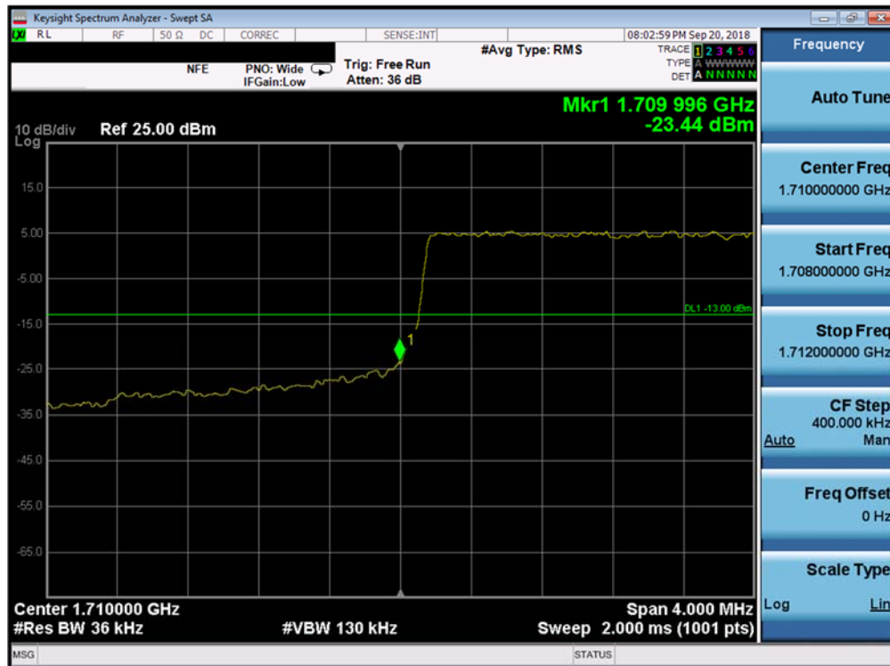
Plot 7-113. Lower Band Edge Plot (Band 4 - 3.0MHz QPSK - Full RB Configuration)
