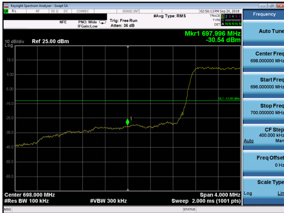
Plot 7-93. Lower Band Edge Plot (Band 12 - 3.0MHz QPSK - Full RB Configuration)
