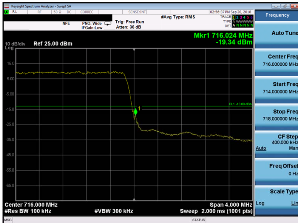
Plot 7-94. Upper Band Edge Plot (Band 12 - 3.0MHz QPSK - Full RB Configuration)
