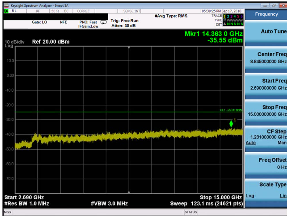
Plot 7-86. Conducted Spurious Plot (Band 41 - 20.0MHz QPSK - RB Size 1, RB Offset 0 - Mid Channel)
