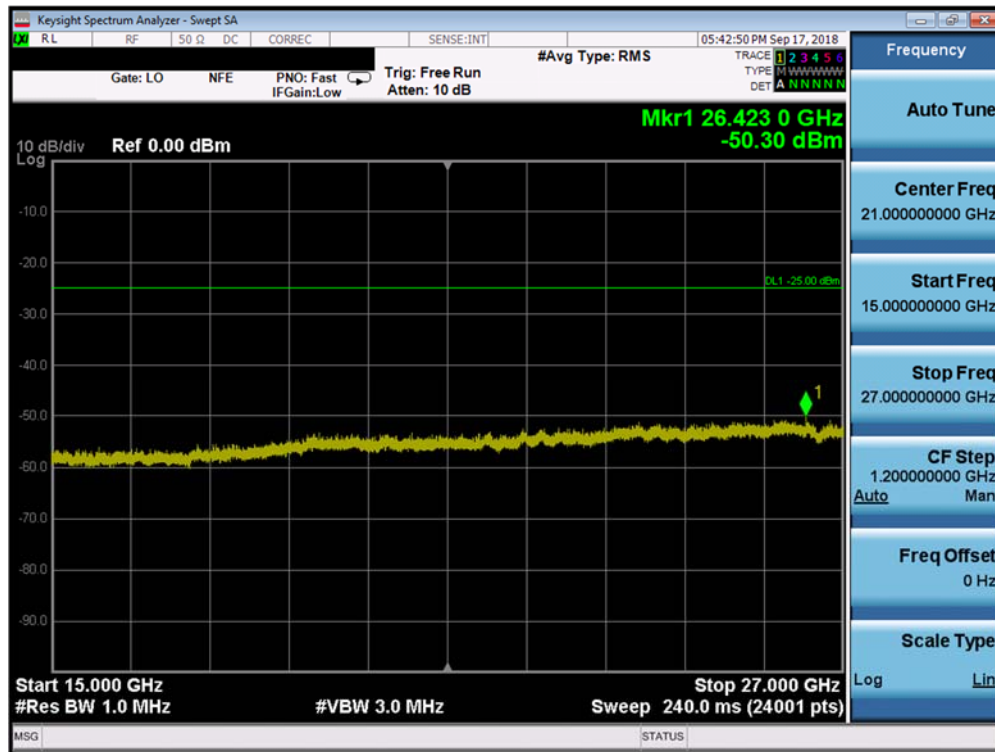
Plot 7-84. Conducted Spurious Plot (Band 41 - 20.0MHz QPSK - RB Size 1, RB Offset 0 - Low Channel)
