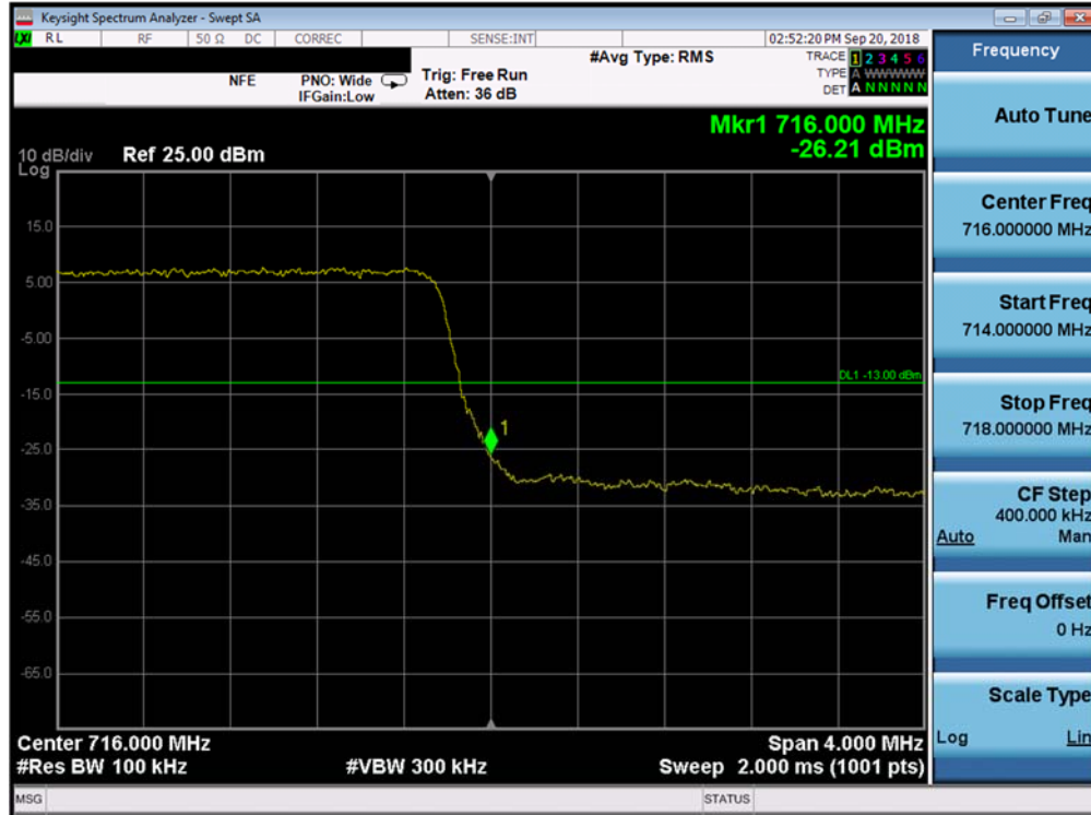
Plot 7-97. Upper Band Edge Plot (Band 12/17 - 5.0MHz QPSK - Full RB Configuration)
