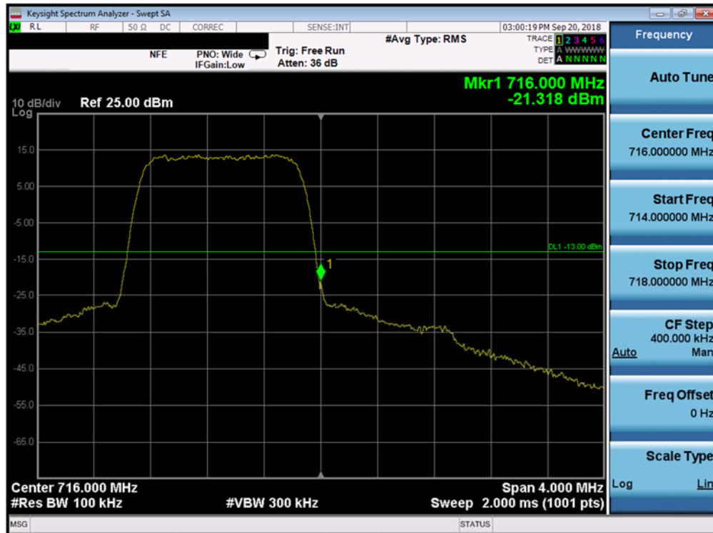
Plot 7-92. Upper Band Edge Plot (Band 12 - 1.4MHz QPSK - Full RB Configuration)
