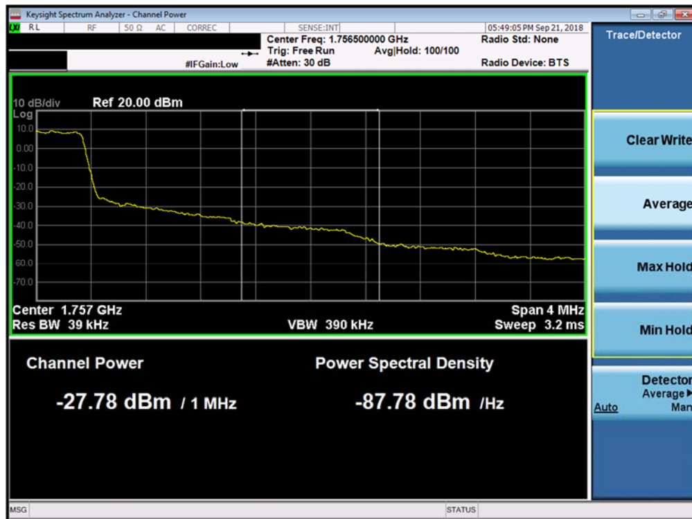
Plot 7-112. Upper Extended Band Edge Plot (Band 4 - 1.4MHz QPSK - Full RB Configuration)
