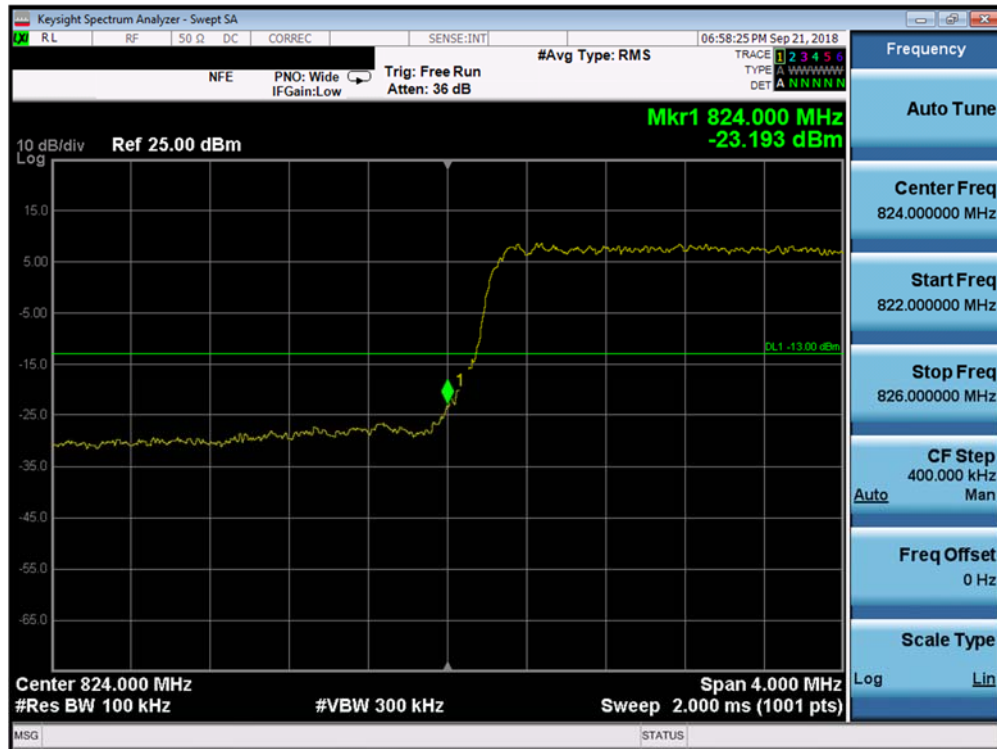
Plot 7-105. Lower Band Edge Plot (Band 5 - 5.0MHz QPSK - Full RB Configuration)
