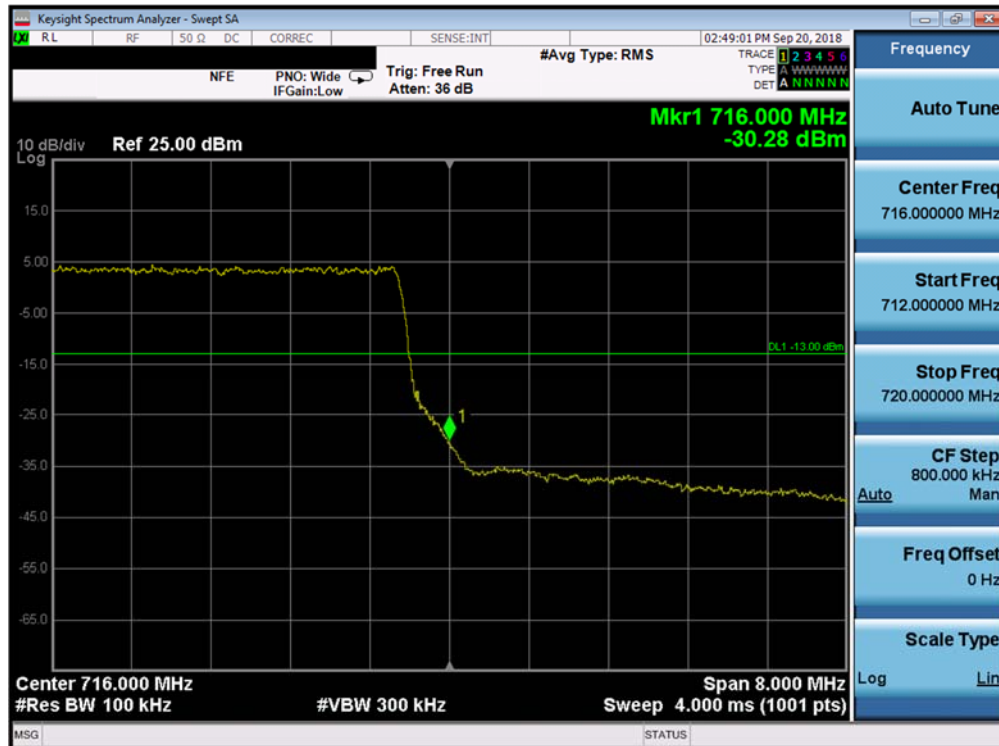
Plot 7-100. Upper Band Edge Plot (Band 12/17 - 10.0MHz QPSK - Full RB Configuration)
