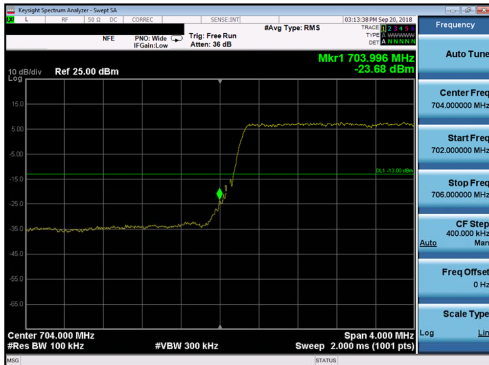
Plot 7-96. Lower Band Edge Plot (Band 17 - 5.0MHz QPSK - Full RB Configuration)
