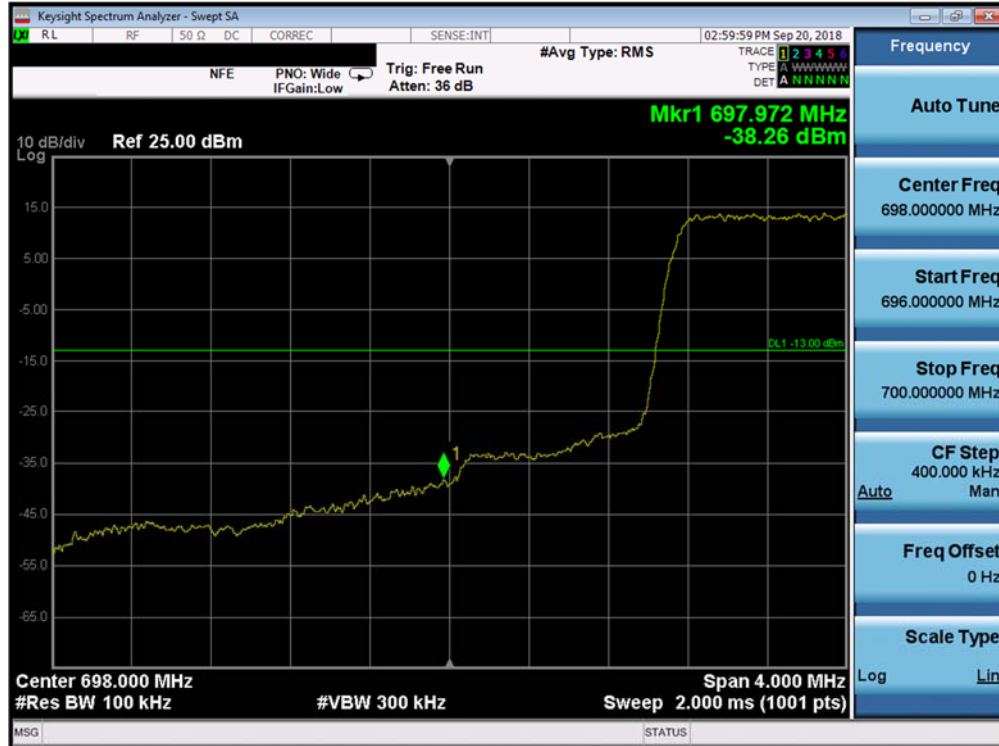
Plot 7-91. Lower Band Edge Plot (Band 12 - 1.4MHz QPSK - Full RB Configuration)
