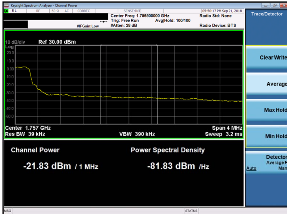
Plot 7-120. Upper Extended Band Edge Plot (Band 4 - 5.0MHz QPSK - Full RB Configuration)
