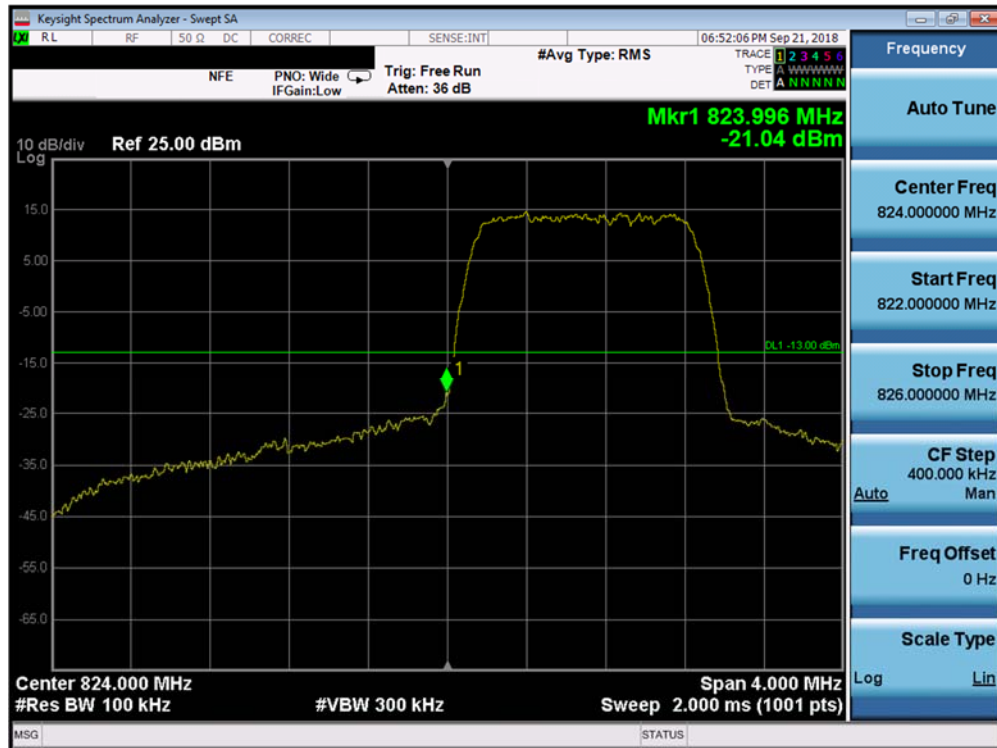
Plot 7-101. Lower Band Edge Plot (Band 5 - 1.4MHz QPSK - Full RB Configuration)
