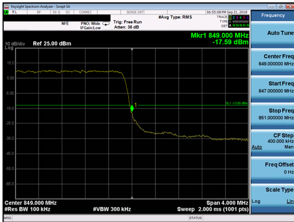
Plot 7-104. Upper Band Edge Plot (Band 5 - 3.0MHz QPSK - Full RB Configuration)
