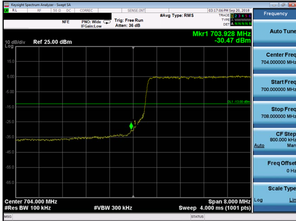
Plot 7-99. Lower Band Edge Plot (Band 17 - 10.0MHz QPSK - Full RB Configuration)
