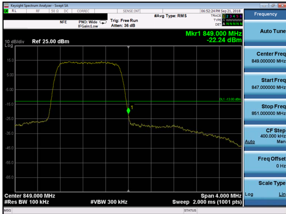
Plot 7-102. Upper Band Edge Plot (Band 5 - 1.4MHz QPSK - Full RB Configuration)
