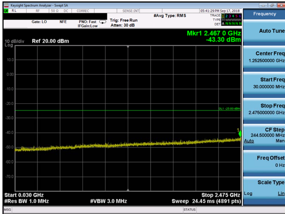
Plot 7-82. Conducted Spurious Plot (Band 41 - 20.0MHz QPSK - RB Size 1, RB Offset 0 - Low Channel)
