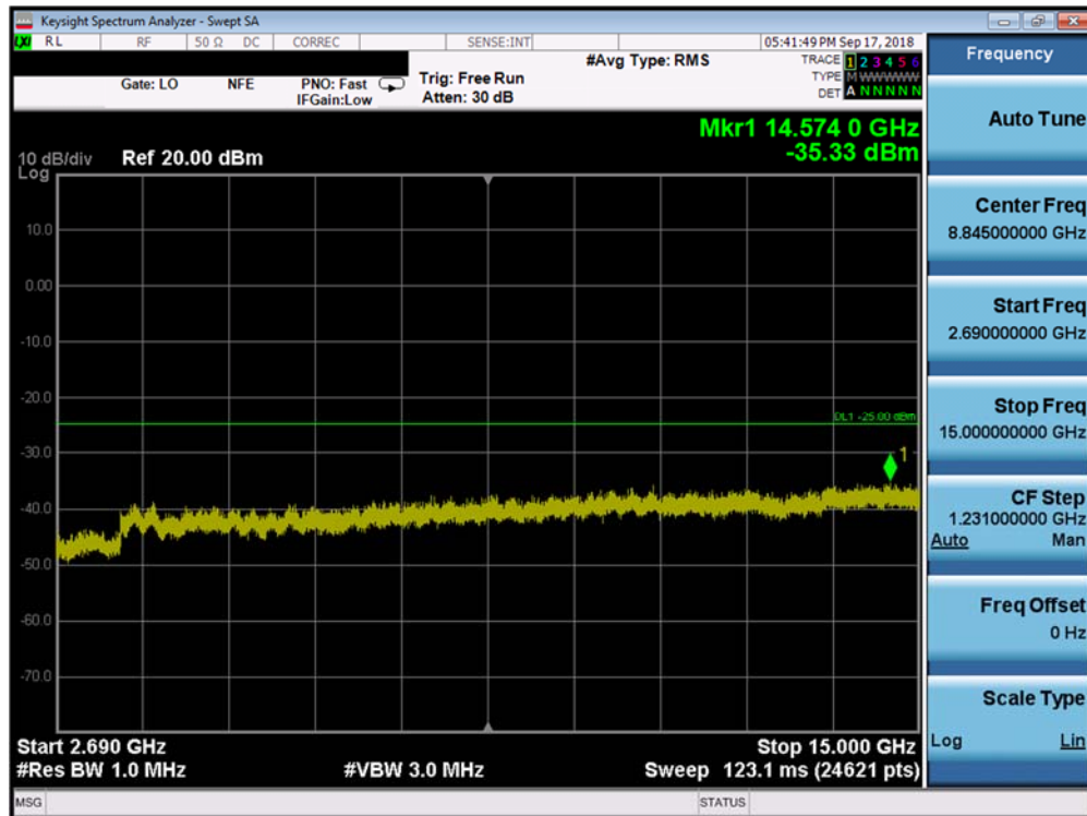
Plot 7-83. Conducted Spurious Plot (Band 41 - 20.0MHz QPSK - RB Size 1, RB Offset 0 - Low Channel)
