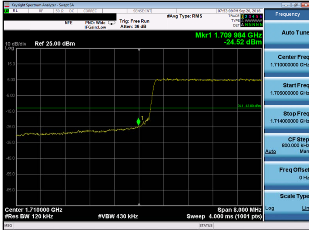
Plot 7-121. Lower Band Edge Plot (Band 4 - 10.0MHz QPSK - Full RB Configuration)
