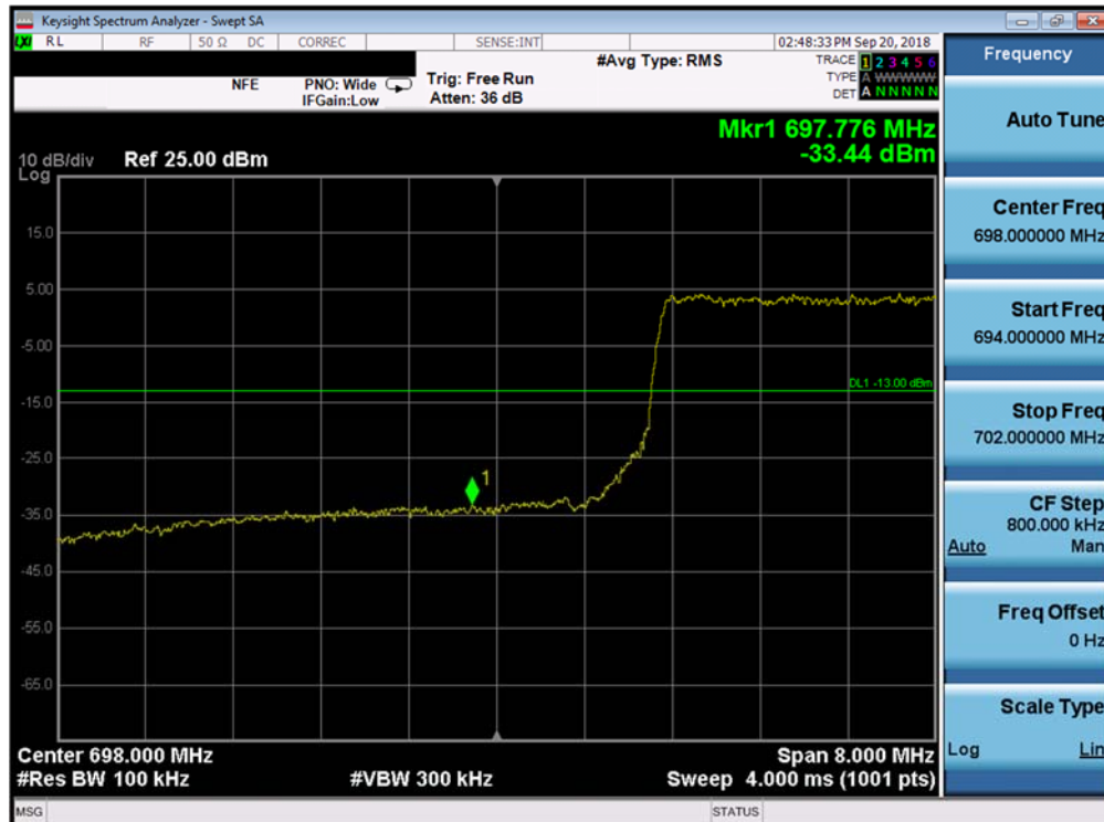
Plot 7-98. Lower Band Edge Plot (Band 12 - 10.0MHz QPSK - Full RB Configuration)
