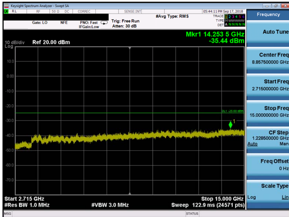
Plot 7-89. Conducted Spurious Plot (Band 41 - 20.0MHz QPSK - RB Size 1, RB Offset 0 - High Channel)
