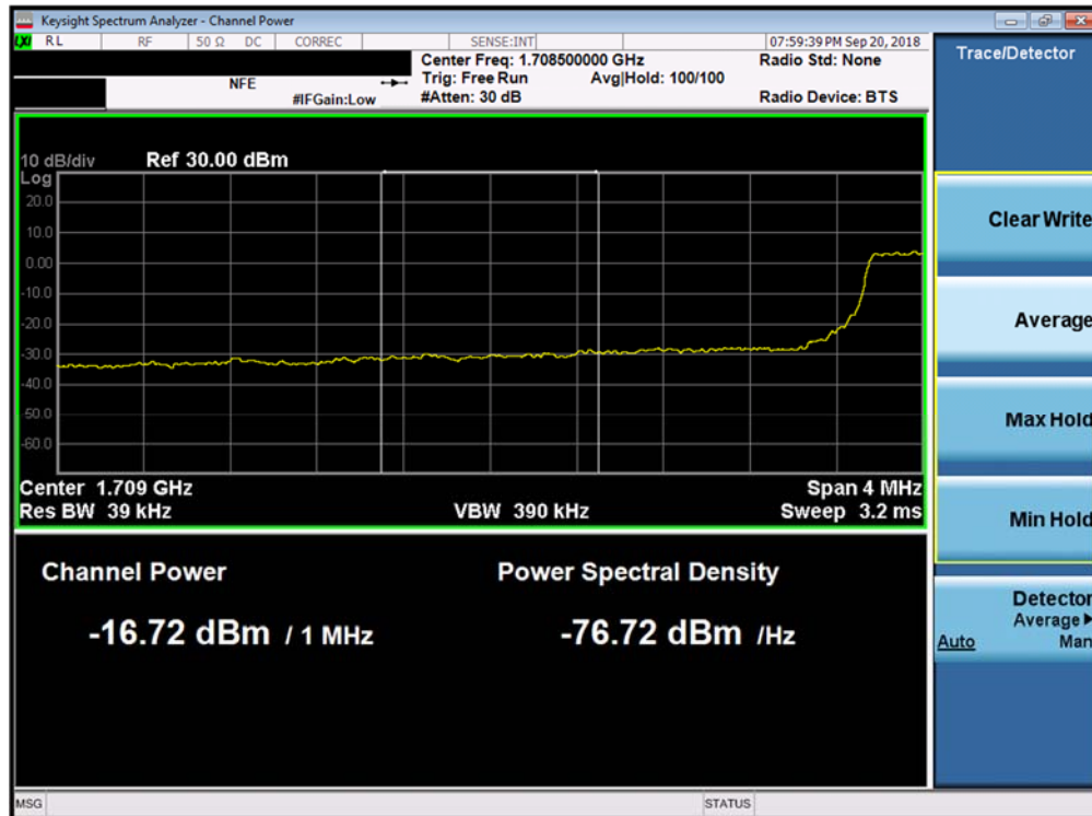
Plot 7-118. Lower Extended Band Edge Plot (Band 4 - 5.0MHz QPSK - Full RB Configuration)
