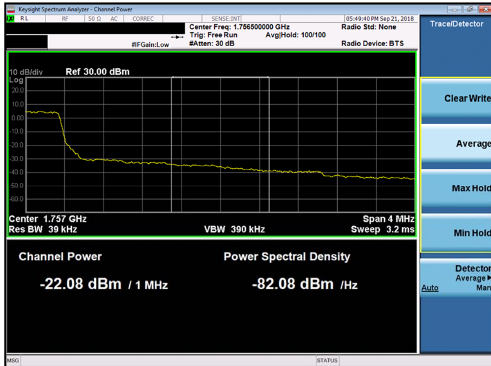
Plot 7-116. Upper Extended Band Edge Plot (Band 4 - 3.0MHz QPSK - Full RB Configuration)
