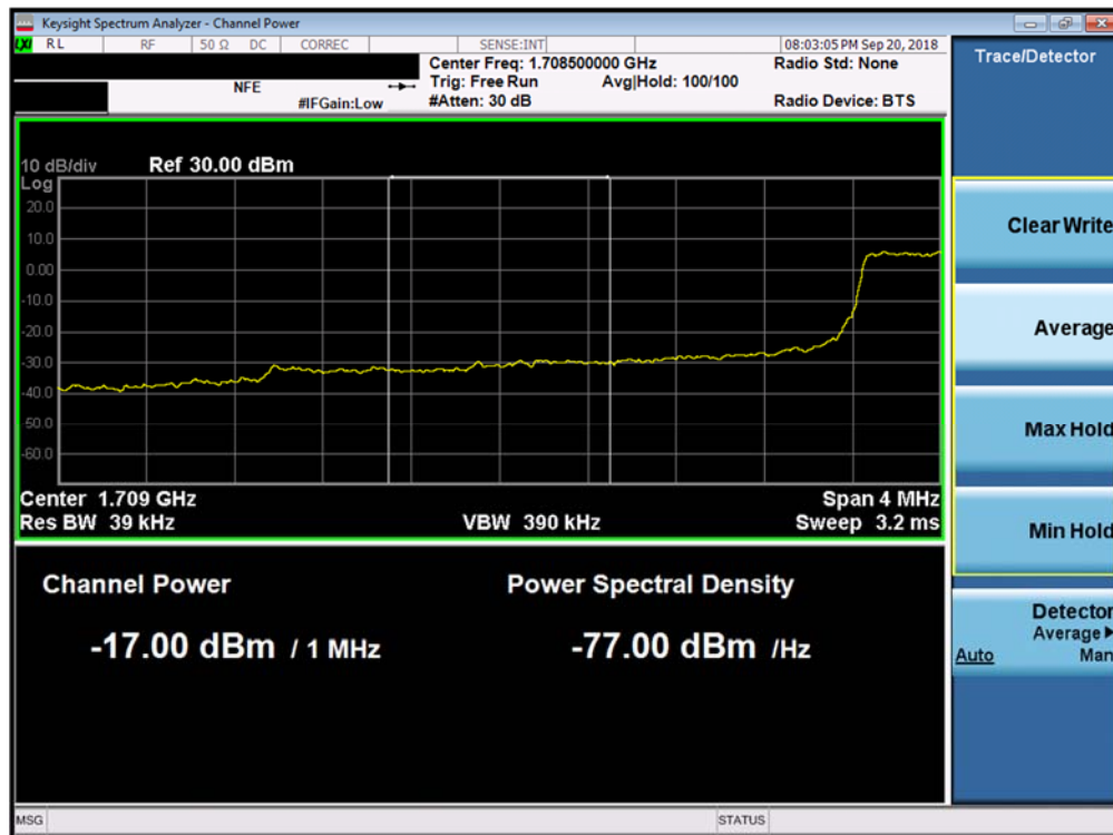
Plot 7-114. Lower Extended Band Edge Plot (Band 4 - 3.0MHz QPSK - Full RB Configuration)
