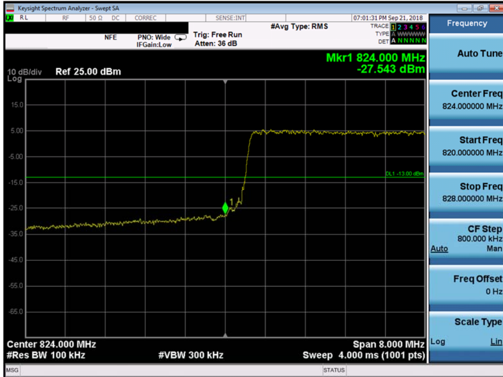
Plot 7-107. Lower Band Edge Plot (Band 5 - 10.0MHz QPSK - Full RB Configuration)
