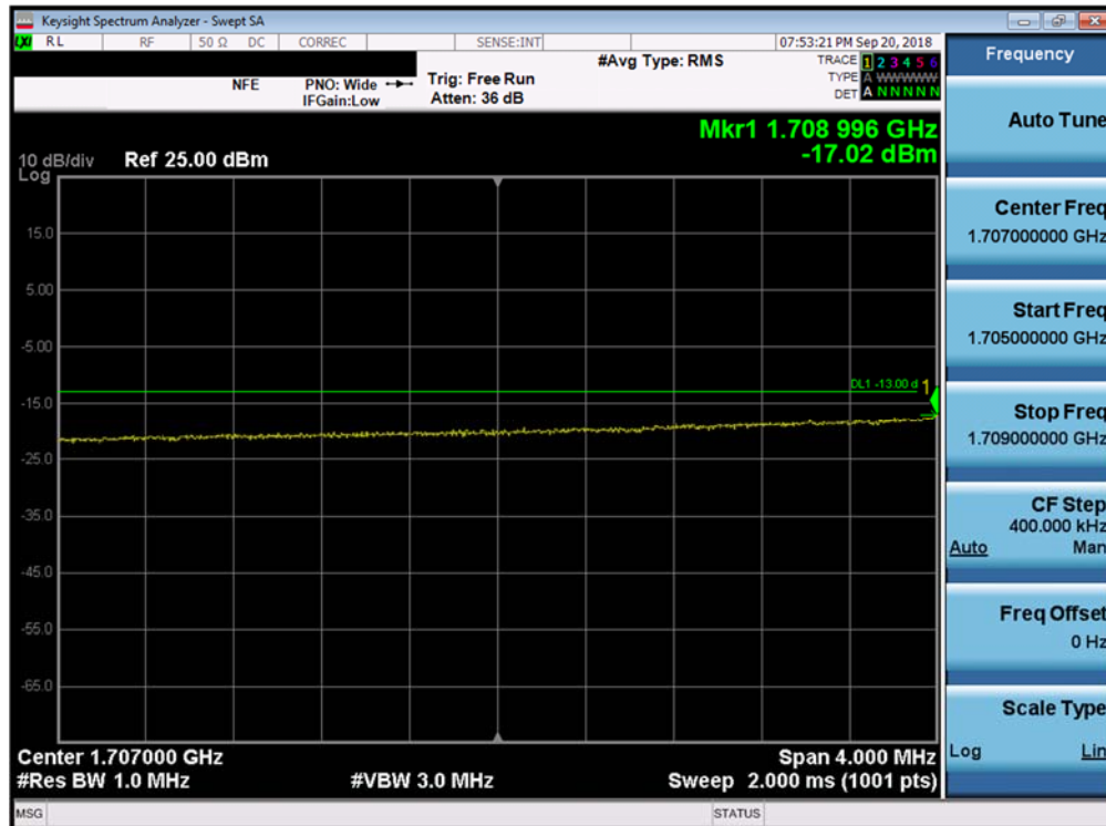
Plot 7-122. Lower Extended Band Edge Plot (Band 4 - 10.0MHz QPSK - Full RB Configuration)
