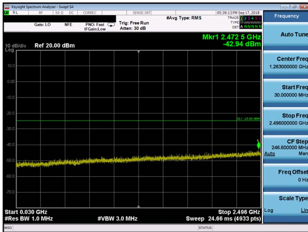
Plot 7-85. Conducted Spurious Plot (Band 41 - 20.0MHz QPSK - RB Size 1, RB Offset 0 - Mid Channel)
