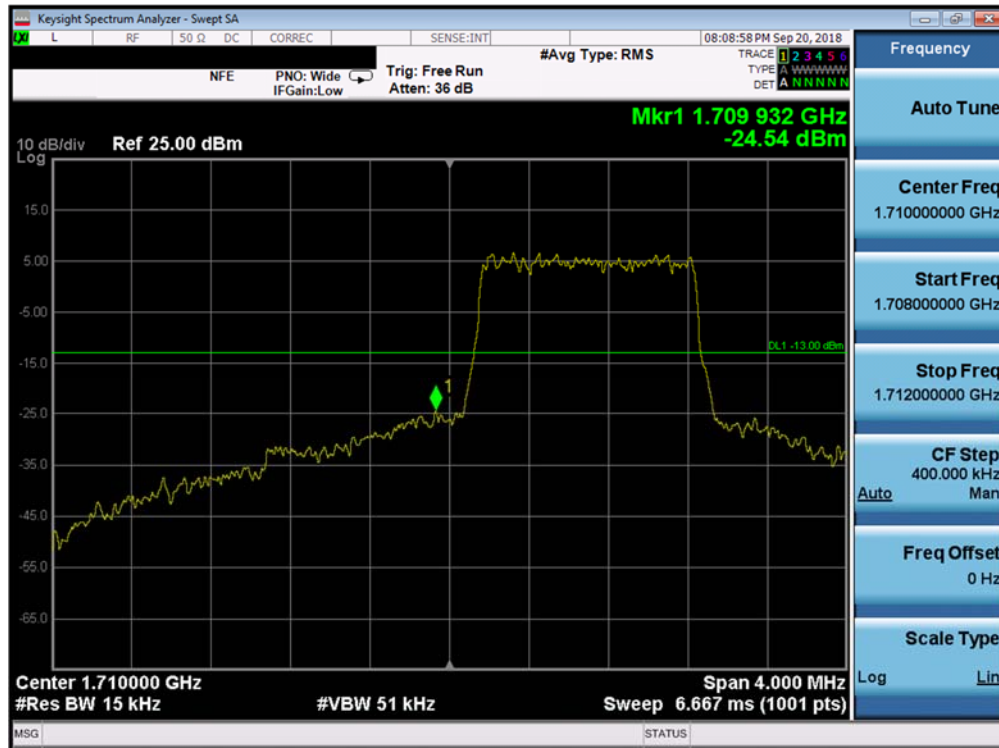
Plot 7-109. Lower Band Edge Plot (Band 4 - 1.4MHz QPSK - Full RB Configuration)
