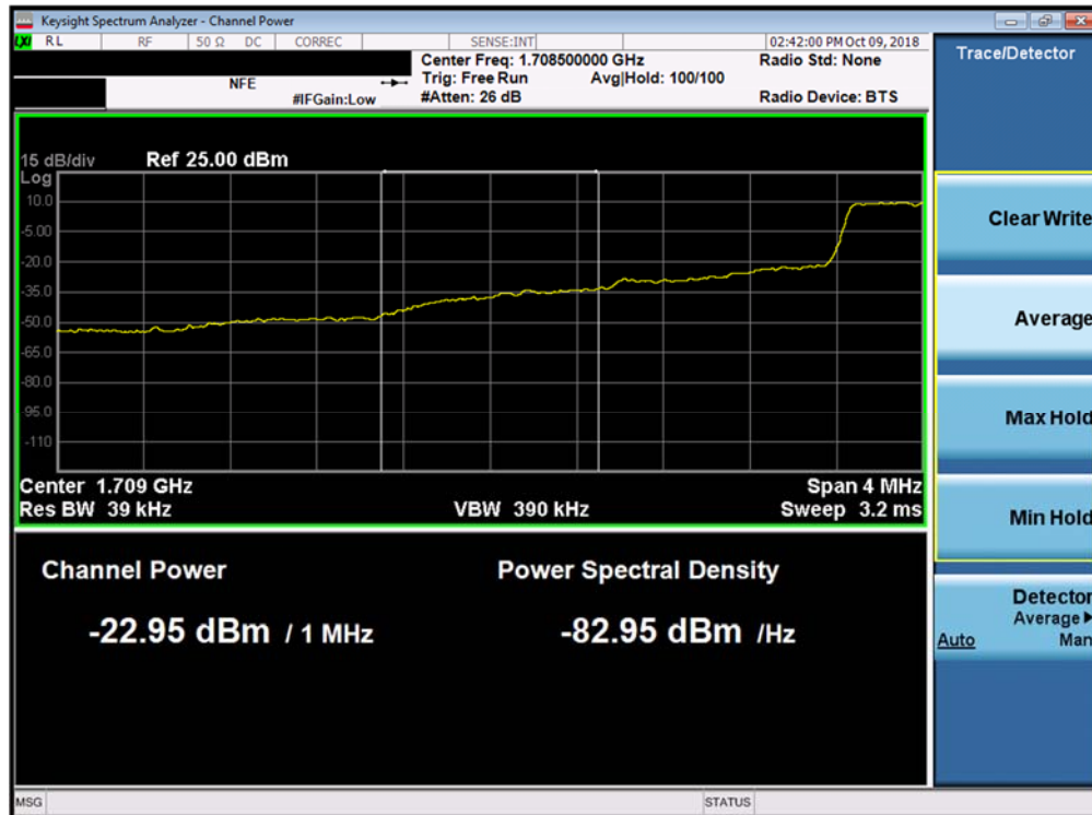
Plot 7-110. Lower Extended Band Edge Plot (Band 4 - 1.4MHz QPSK - Full RB Configuration)
