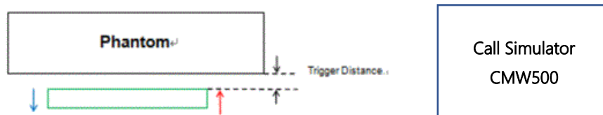
Proximity Sensor Trigger Distance Assessment KDB 616217 D04 §6.2, front side
