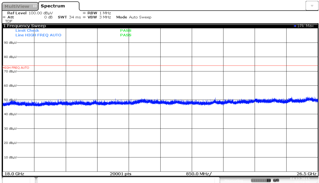
Plot 7-37. Radiated Spurious Plot above 18GHz (Pol. H)
