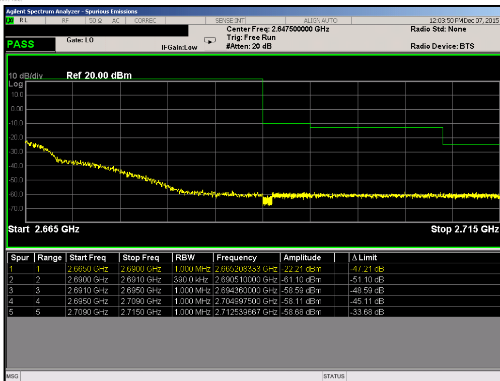
Plot 7-54. Upper ACP Plot (Band 41 – 15.0MHz QPSK – RB Size 75)
