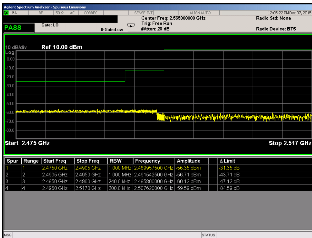
Plot 7-55. Lower ACP Plot (Band 41 – 20.0MHz QPSK – RB Size 100)
