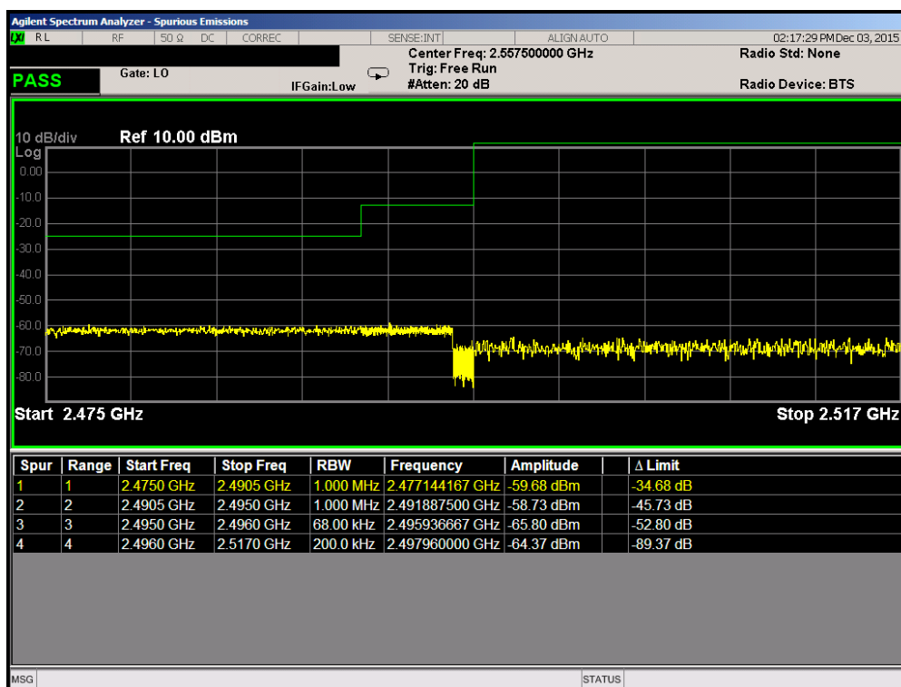
Plot 7-49. Lower ACP Plot (Band 41 – 5.0MHz QPSK – RB Size 25)
