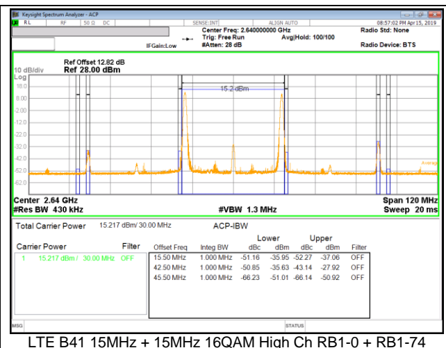
LTE B41 15MHz + 15MHz 16QAM High Ch RB1-0 + RB1-74
