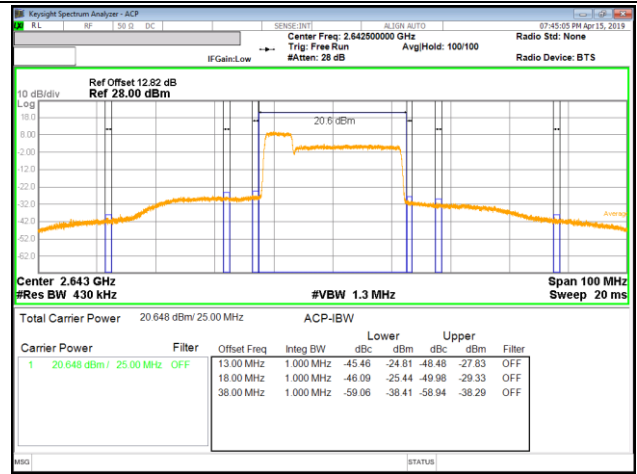
LTE B41 5MHz + 20MHz 16QAM High Ch RB25-0 + RB100-0
