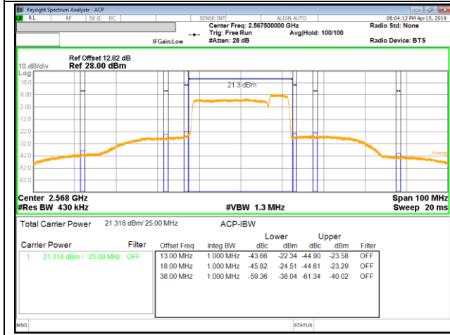
LTE B41 20MHz + 5MHz QPSK Low Ch RB100-0 + RB25-0
