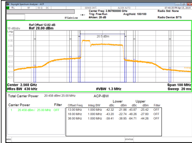
LTE B41 5MHz + 20MHz 16QAM Low Ch RB25-0 + RB100-0
