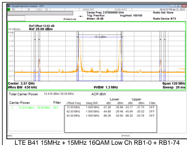
LTE B41 15MHz + 15MHz 16QAM Low Ch RB1-0 + RB1-74
