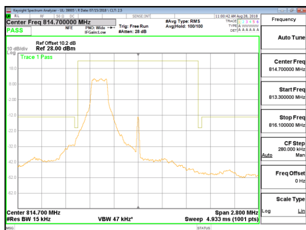
LTE B26 1.4MHz 16QAM Low Channel RB1-00
