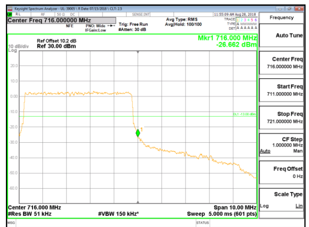
LTE B17 5MHz QPSK High Channel RB25-0
