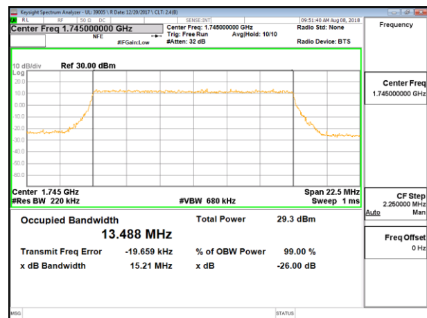
LTE B66 15MHz 16QAM Mid Channel RB75-0
