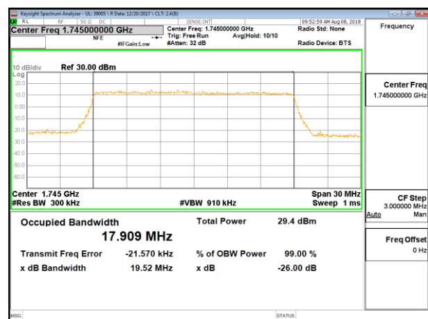
LTE B66 20MHz 16QAM Mid Channel RB100-0
