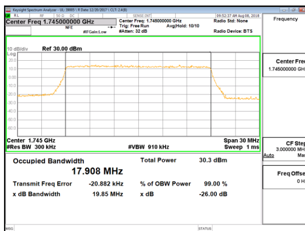
LTE B66 20MHz QPSK Mid Channel RB100-0
