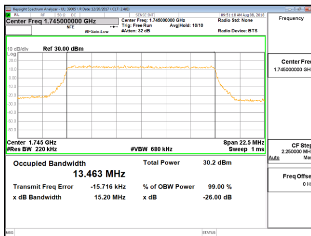
LTE B66 15MHz QPSK Mid Channel RB75-0
