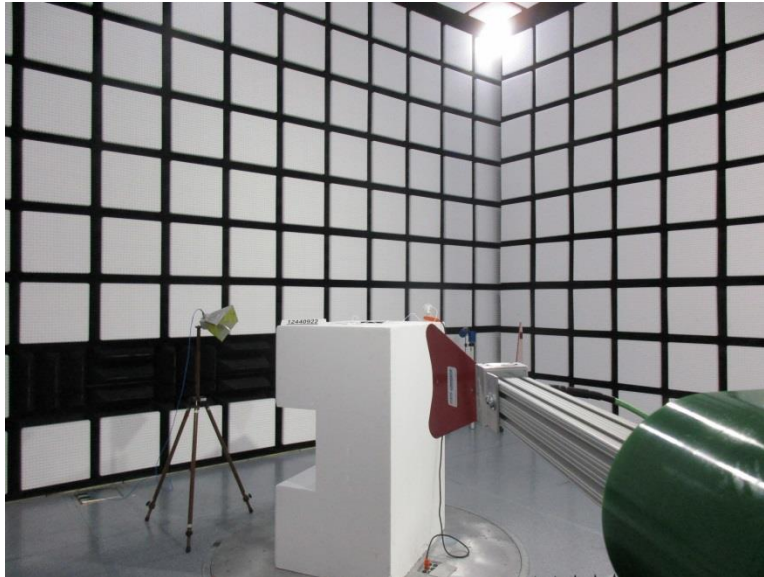
RADIATED EMISSIONS MEASUREMENT SETUP
