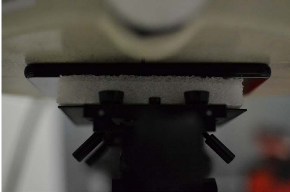
SAR Test Setup Photo 7: Front at 0.0 cm
