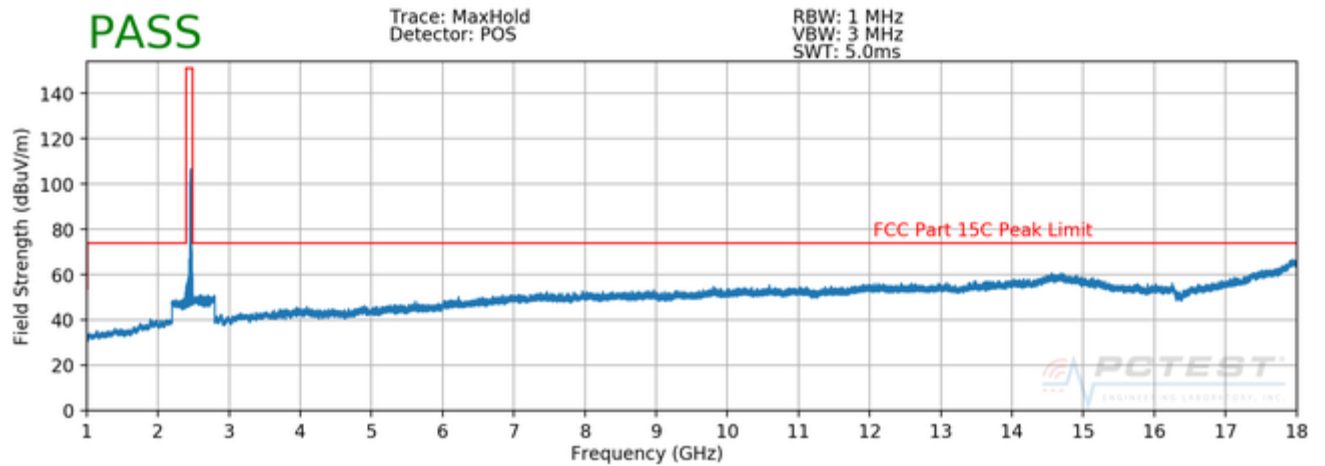
Plot 7-41. Radiated Spurious Plot above 1GHz (802.11b – Ch. 11, Ant. Pol. H)
