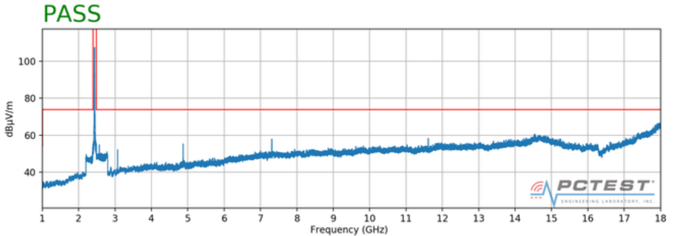
Plot 7-40. Radiated Spurious Plot above 1GHz (802.11b – Ch. 6, Ant. Pol. V)
