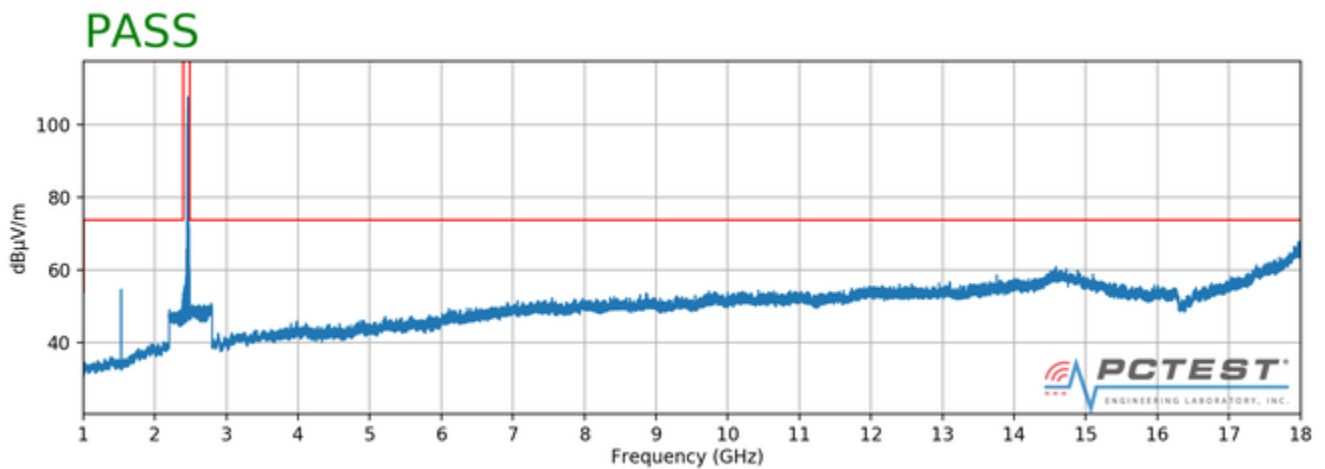
Plot 7-42. Radiated Spurious Plot above 1GHz (802.11b – Ch. 11, Ant. Pol. V)
