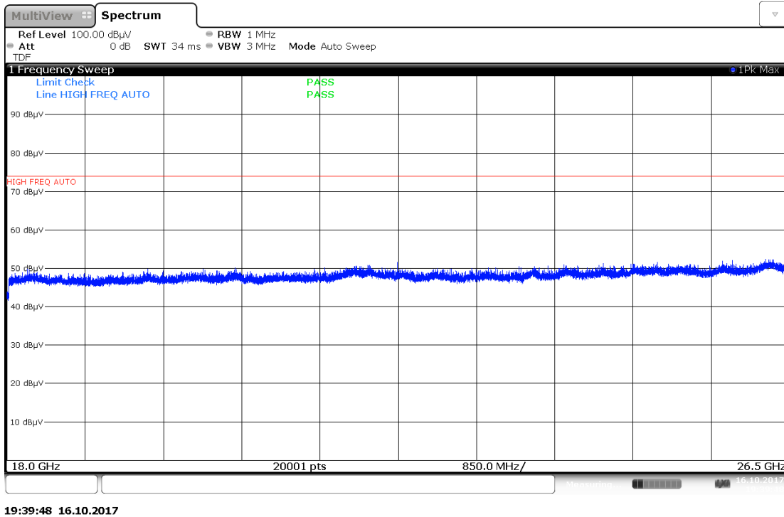
Plot 7-43. Radiated Spurious Plot above 18GHz (Pol. H)
