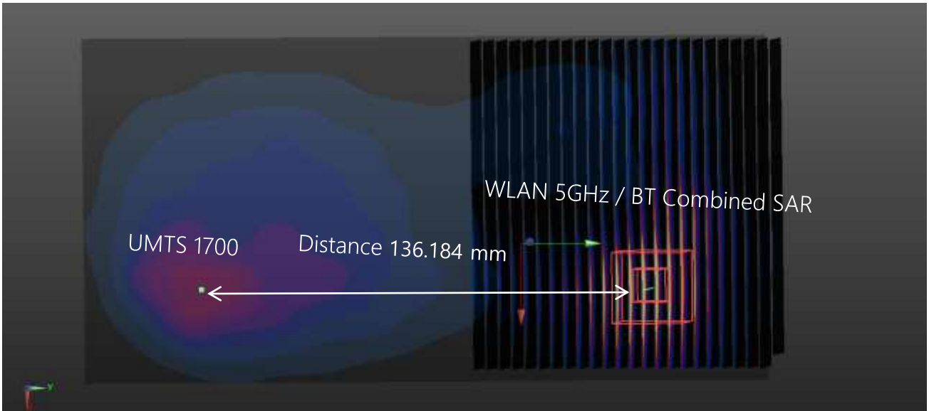
Plot #8 UMTS 1700 + WLAN 5GHz / Bluetooth Combined SAR (Hotspot Mode)
