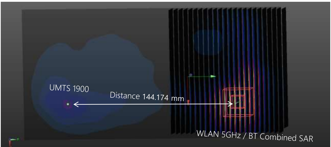
Plot #9 UMTS 1900 + WLAN 5GHz / Bluetooth Combined SAR (Hotspot Mode)
