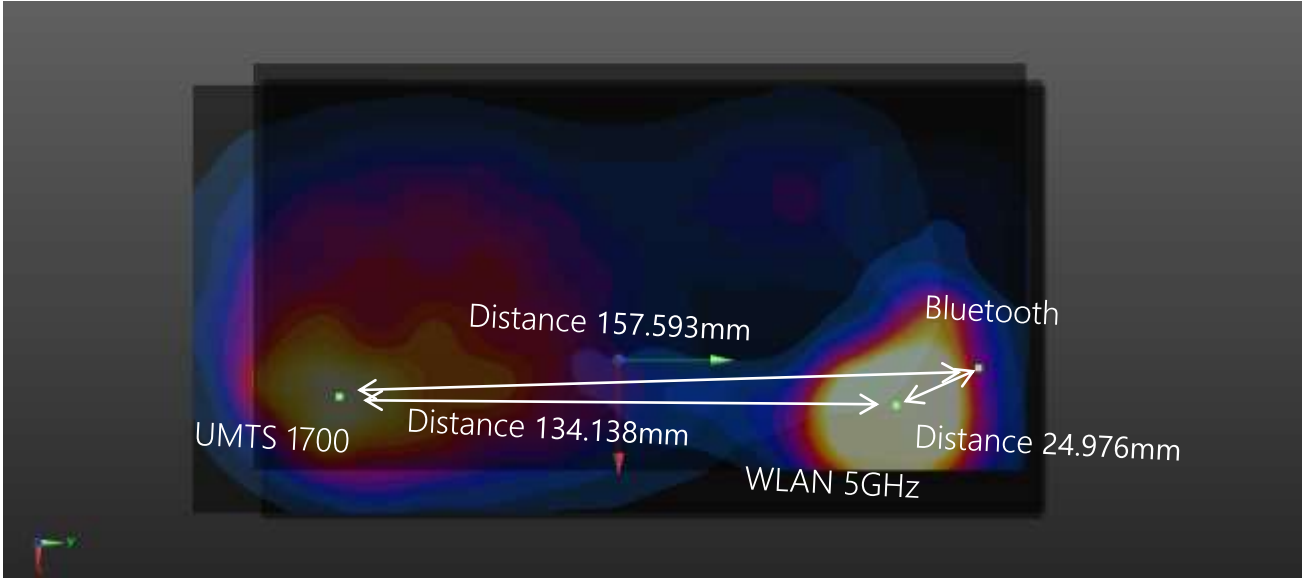
Plot #2 UMTS 1700 + WLAN 5GHz + Bluetooth (Hotspot Mode)
