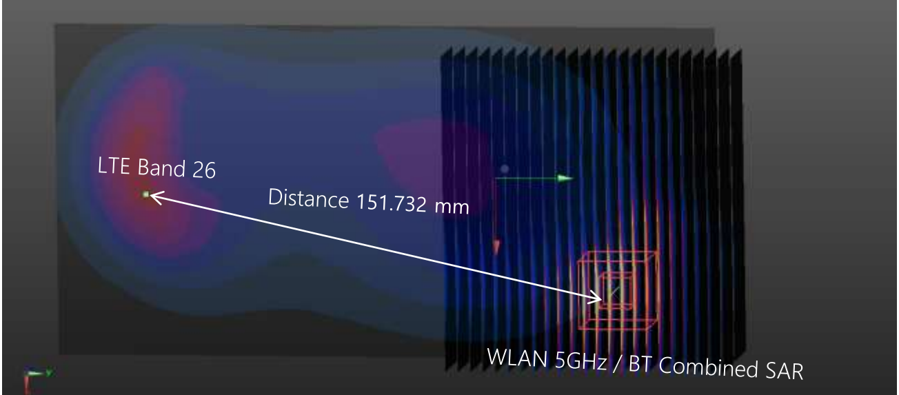
Plot #12 LTE Band 26 + WLAN 5GHz / Bluetooth Combined SAR (Hotspot Mode)
