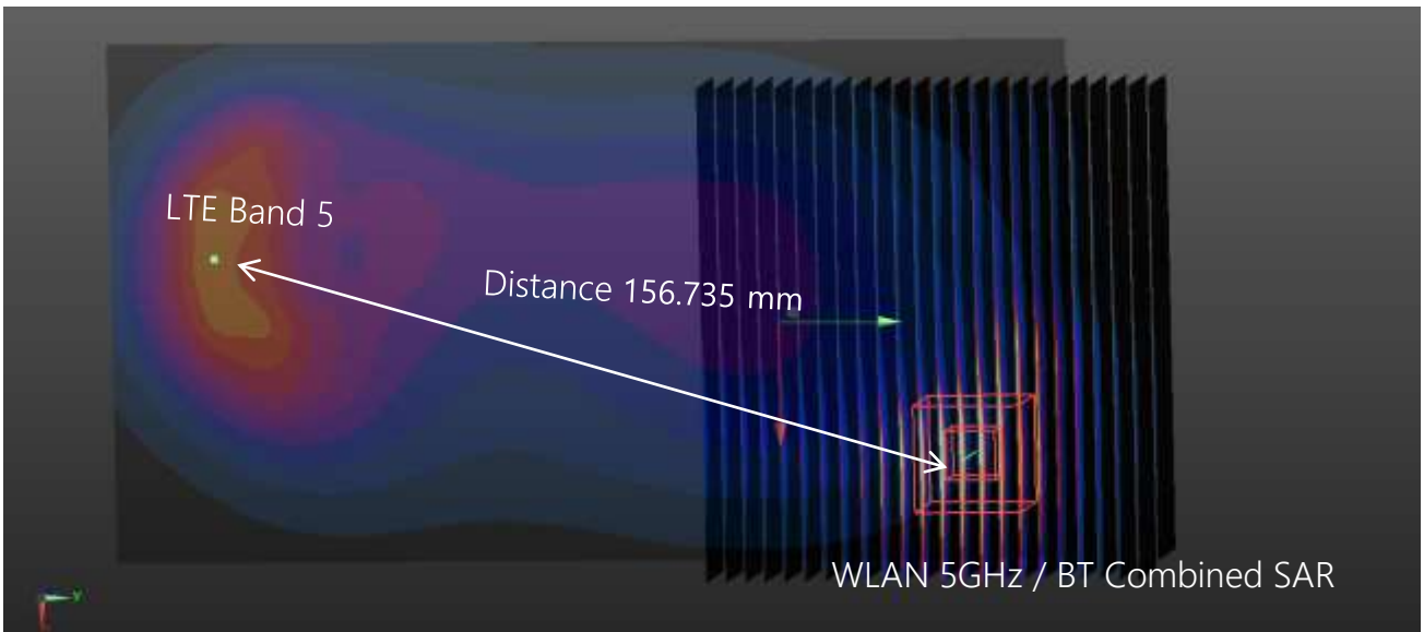
Plot #11 LTE Band 5 + WLAN 5GHz / Bluetooth Combined SAR (Hotspot Mode)
