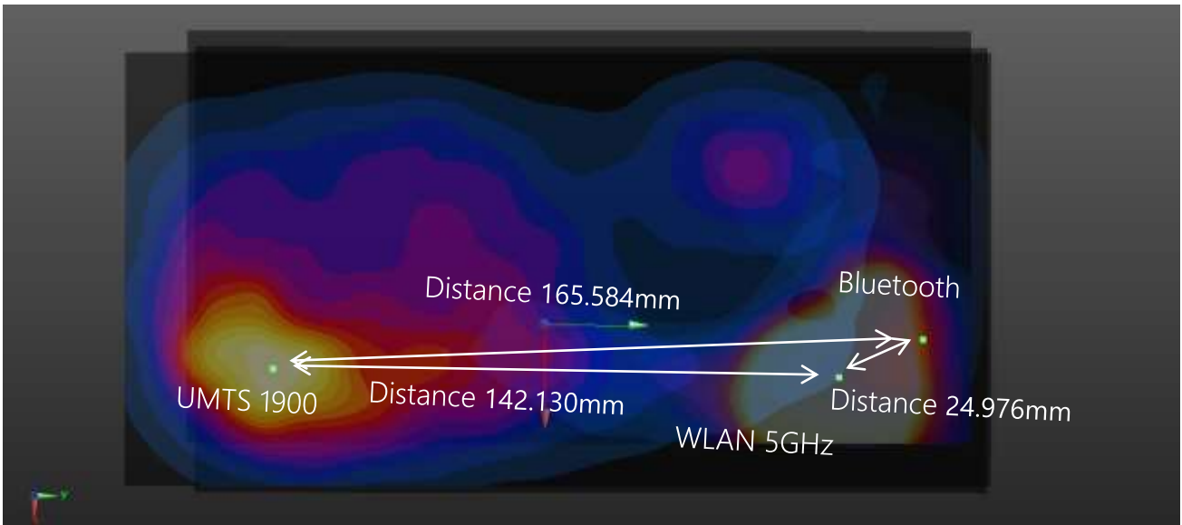
Plot #3 UMTS 1900 + WLAN 5GHz + Bluetooth (Hotspot Mode)
