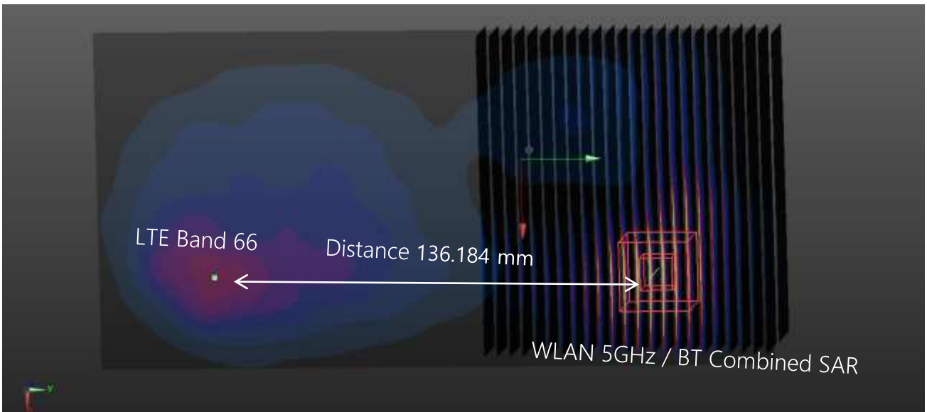
Plot #13 LTE Band 66 + WLAN 5GHz / Bluetooth Combined SAR (Hotspot Mode)
