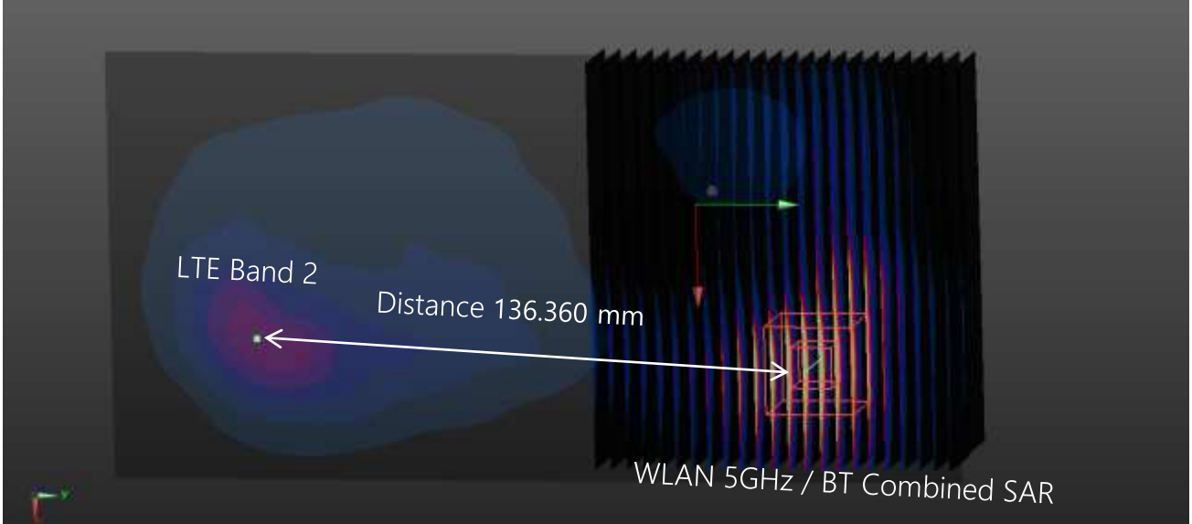
Plot #10 LTE Band 2 + WLAN 5GHz / Bluetooth Combined SAR (Hotspot Mode)
