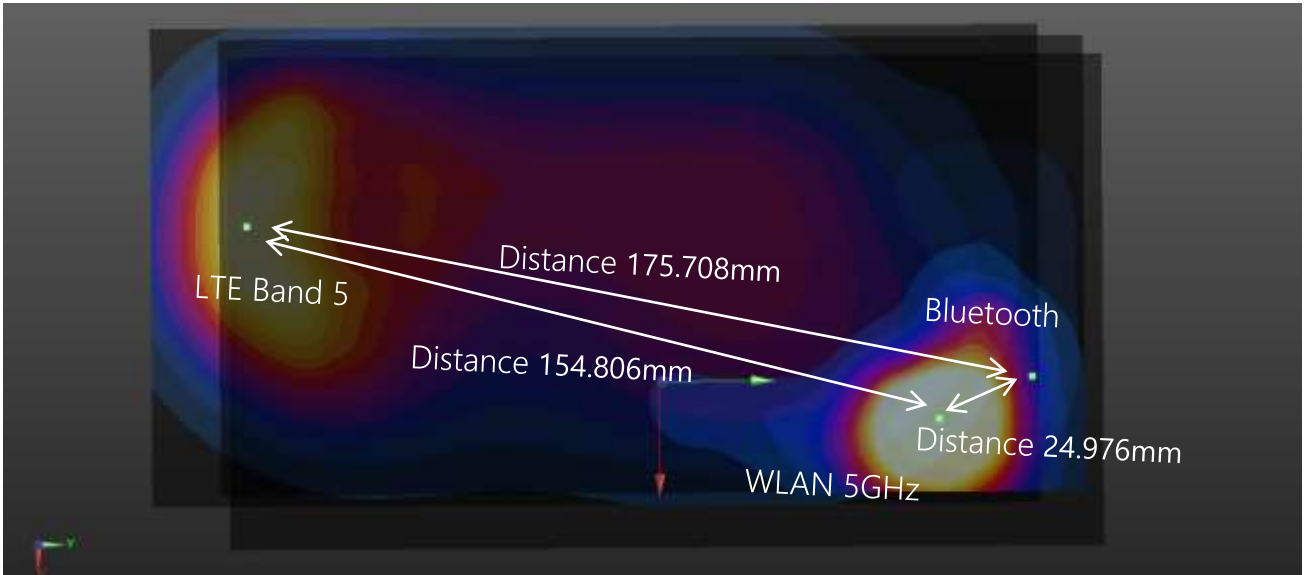
Plot #5 LTE Band 5 + WLAN 5GHz + Bluetooth (Hotspot Mode)
