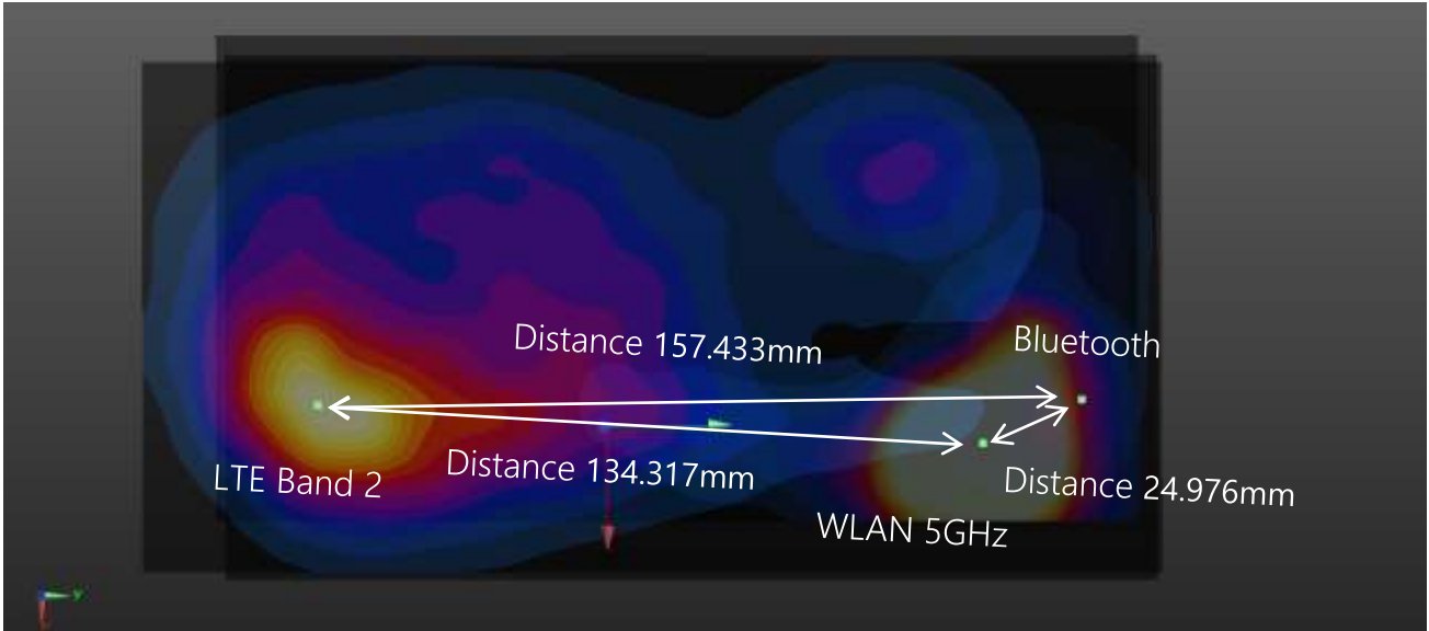
Plot #4 LTE Band 2 + WLAN 5GHz + Bluetooth (Hotspot Mode)
