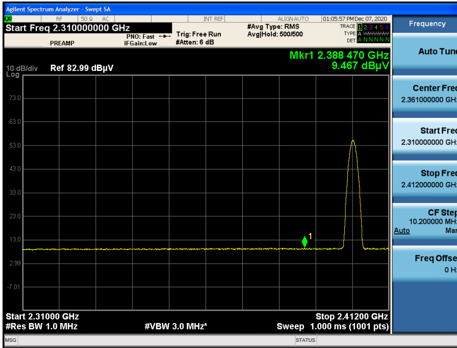
Radiated Restricted Band Edges plot – Peak Reading (Ch.0, X-H)
