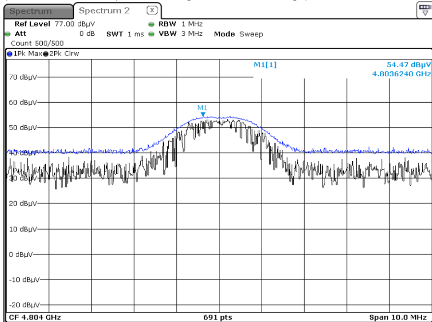
Radiated Spurious Emissions plot – Average & Peak Reading (GFSK, Ch.0 2nd Harmonic, X-H)
