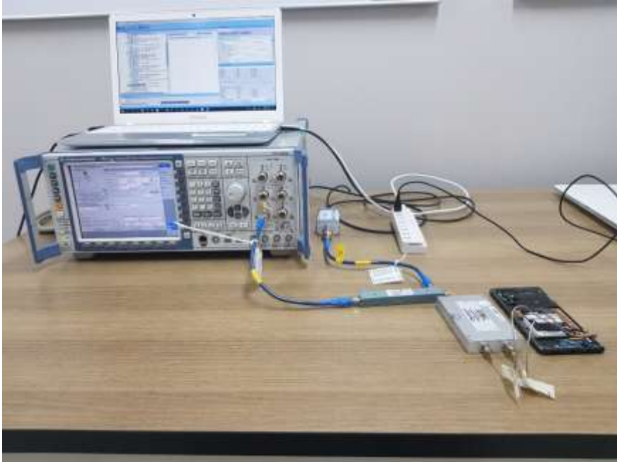
Test setup photo-2 (8-1(b) Antenna Switch)
