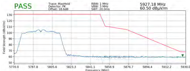
Plot 7-98. Radiated Upper Band Edge Plot (Peak – UNII Band 3)
