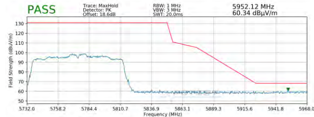
Plot 7-105. Radiated Upper Band Edge Plot (Peak – UNII Band 3)
