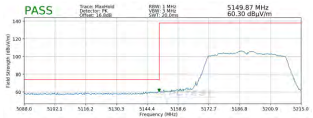
Plot 7-93. Radiated Lower Band Edge Plot (Peak – UNII Band 1)
