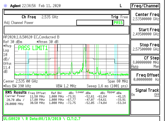
LTE B7 20MHz 16QAM Middle Channel RB1-99
