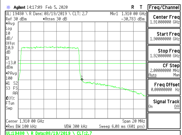
LTE B2 10MHz 16QAM High Channel RB50-0
