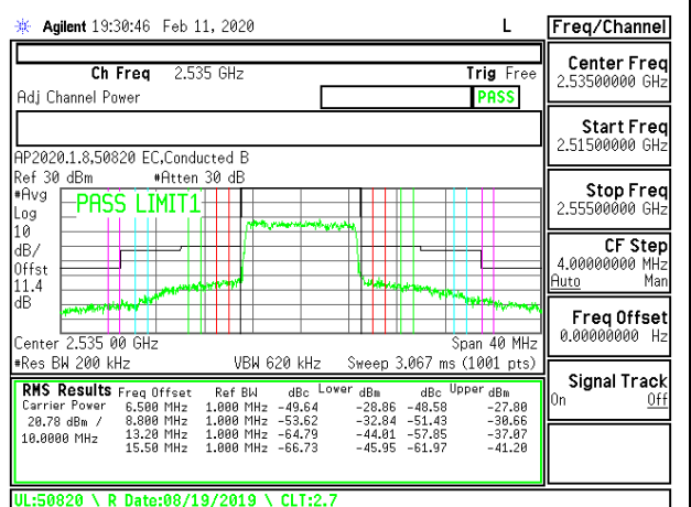
LTE B7 10MHz 16QAM Middle Channel RB50-0
