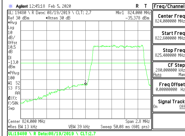
LTE B5 1.4MHz 16QAM Low Channel RB6-0
