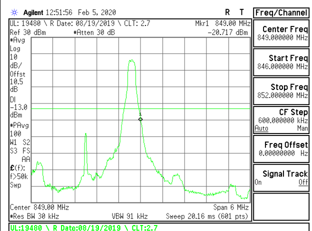
LTE B5 3MHz 16QAM High Channel RB1-14
