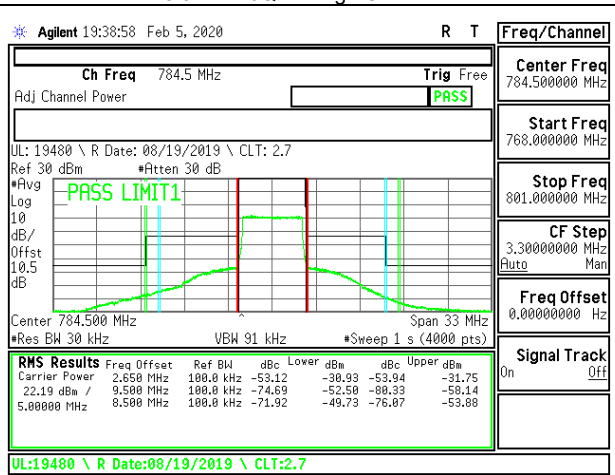
LTE B13 5MHz 16QAM High Channel RB25-0
