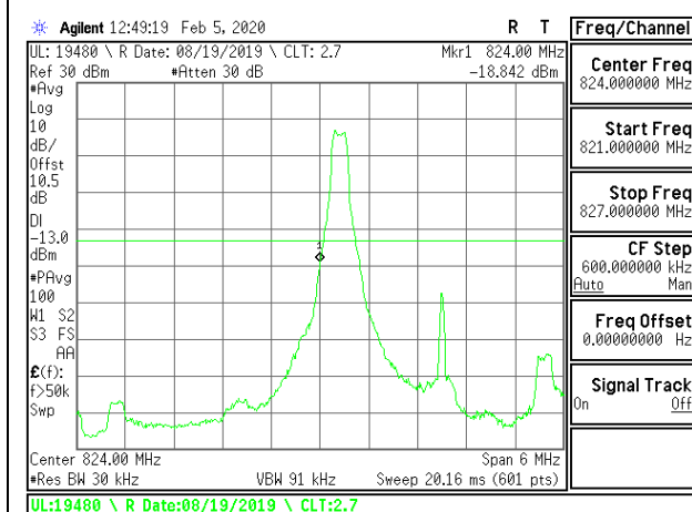
LTE B5 3MHz 16QAM Low Channel RB1-0
