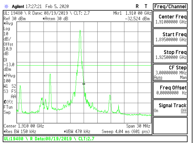
LTE B2 15MHz 16QAM High Channel RB1-74
