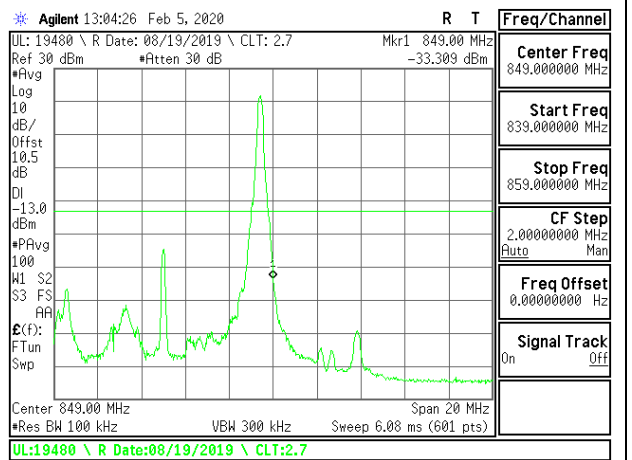
LTE B5 10MHz QPSK High Channel RB1-49
