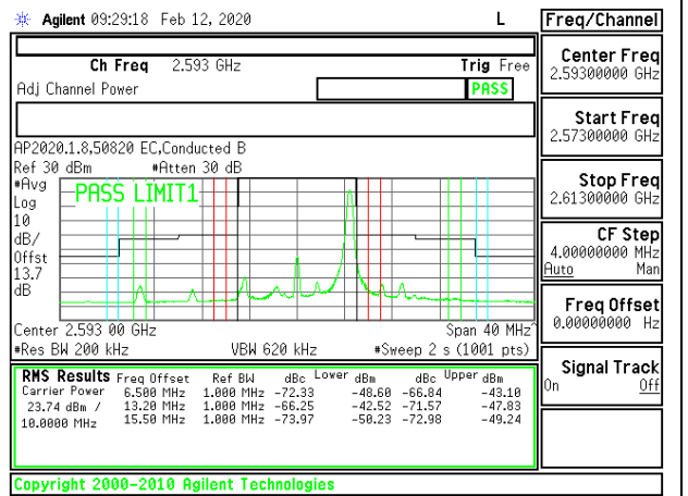
LTE B41 10MHz 16QAM Middle Channel RB1-49
