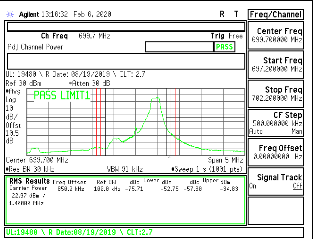
LTE B12 1.4MHz 16QAM Low Channel RB1-5
