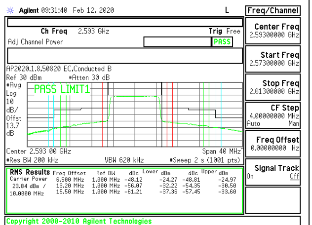
LTE B41 10MHz 16QAM Middle Channel RB50-0
