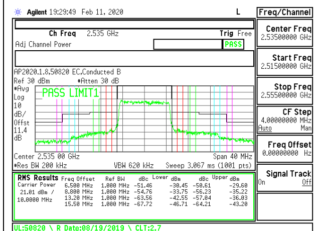
LTE B7 10MHz QPSK Middle Channel RB50-0
