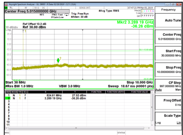
CDMA BC0 1xEV-DO Rev A Low Channel
