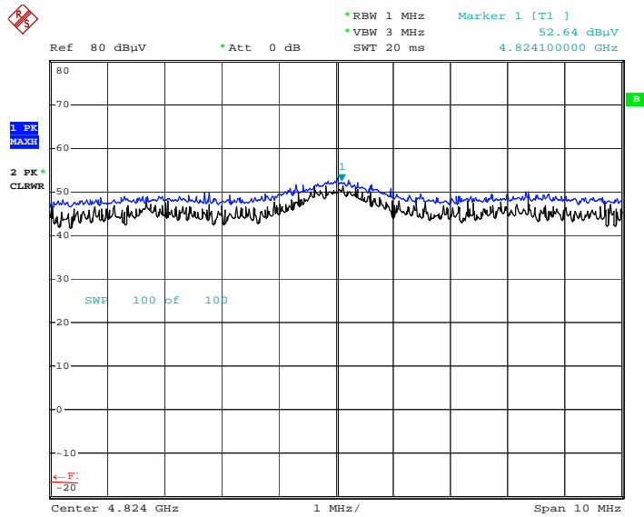
Radiated Spurious Emissions plot – Peak Reading (802.11b, Ch.1 2nd Harmonic, Y-H)
