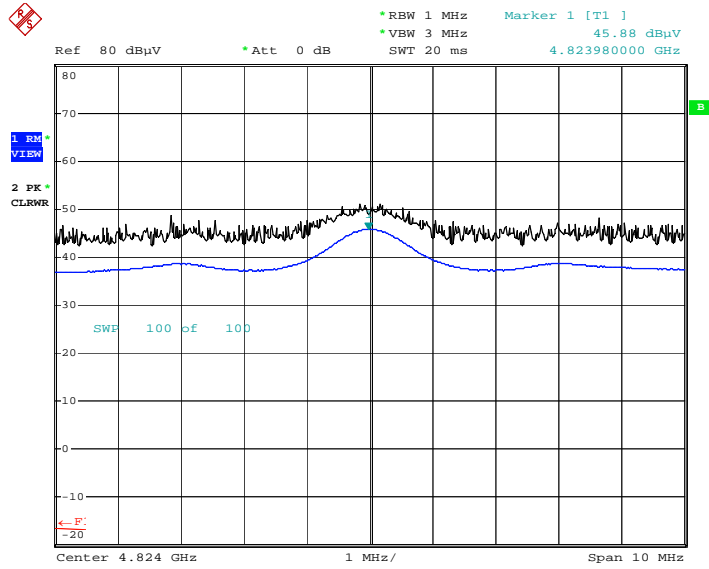
Radiated Spurious Emissions plot – Average Reading (802.11b, Ch.1 2nd Harmonic, Y-H)
