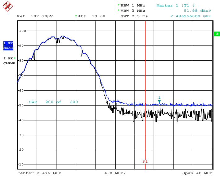
Radiated Restricted Band Edges plot – Peak Reading (802.11b Ch.11)
