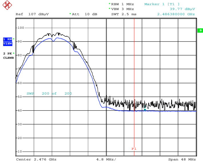
Radiated Restricted Band Edges plot – Average Reading (802.11b Ch.11)
