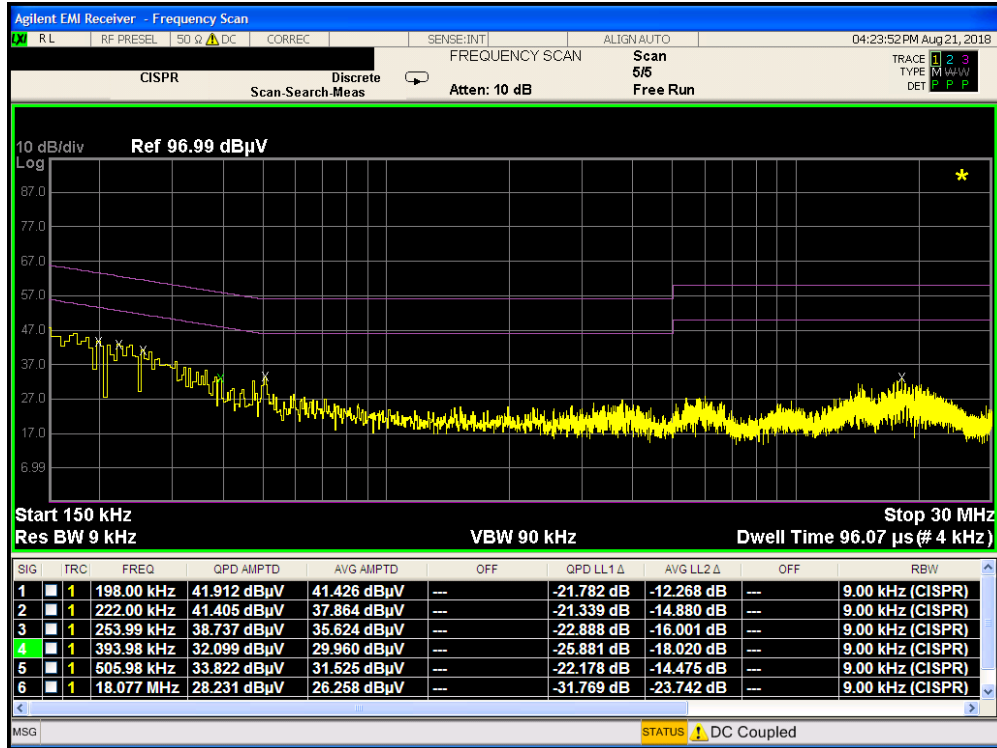
Plot 7-35. Line Conducted Plot with Bluetooth LE (L1)
