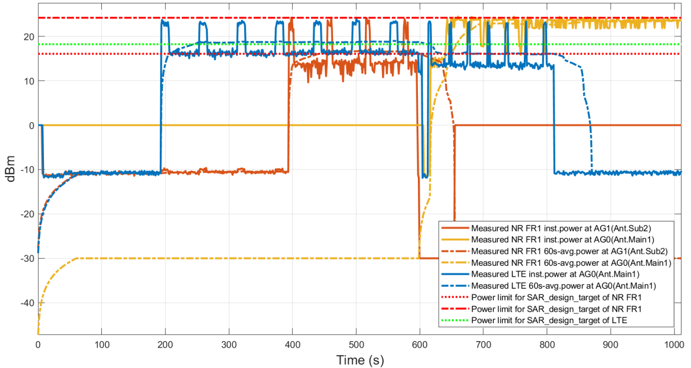
Plot.1 : Conducted Tx power for LTE and NR :
