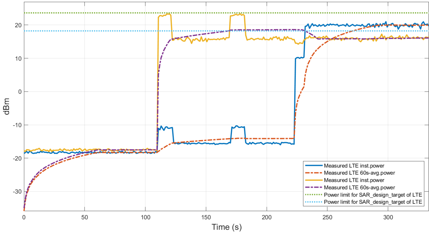
Plot.1 : Time average SAR of LTE ULCA case:
