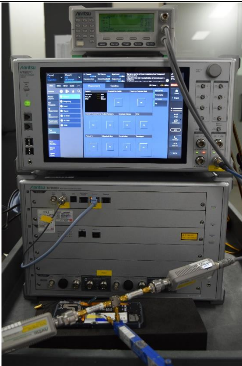
A.3 F_TC 15 Conducted test in MT8821C callbox
