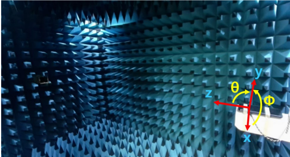
Figure 1: Geometry for SM-A556E/DS for Radiation patterns.
