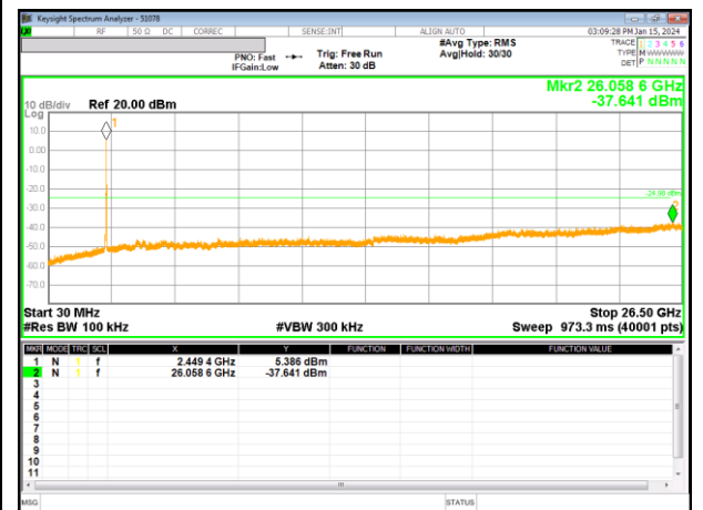
Out-Of-Band 10 Channel
