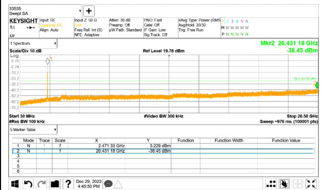
Out-Of-Band 11 Channel(8RU)
