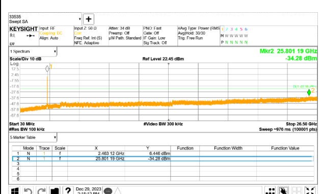
Out-Of-Band 11 Channel
