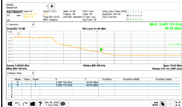
10 Channel Band-edge
