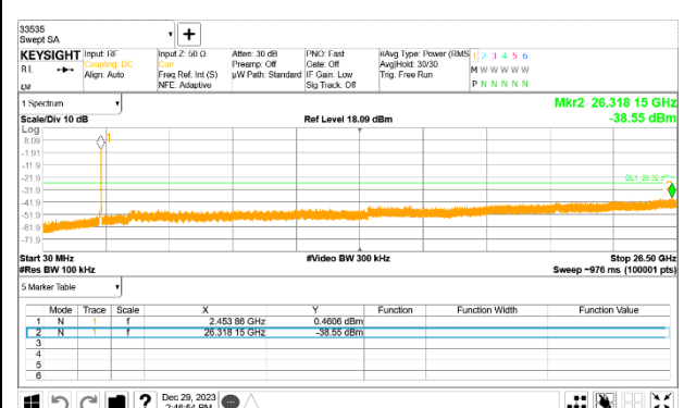
Out-Of-Band 9 Channel
