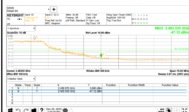
9 Channel Band-edge
