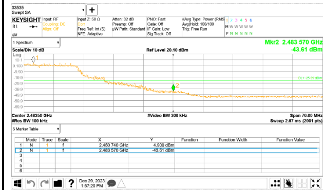
9 Channel Band-edge
