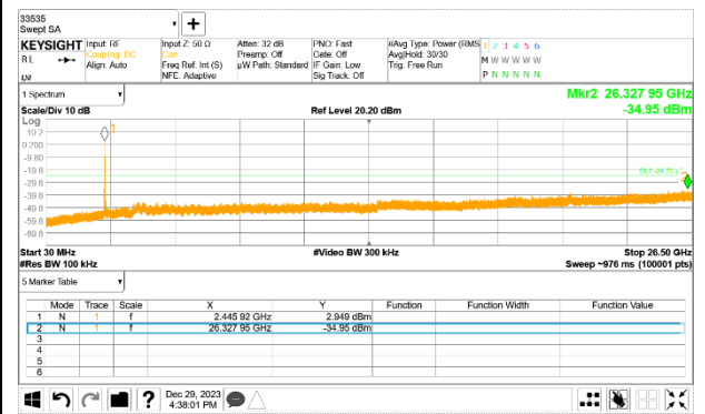
Out-Of-Band 6 Channel(8RU)
