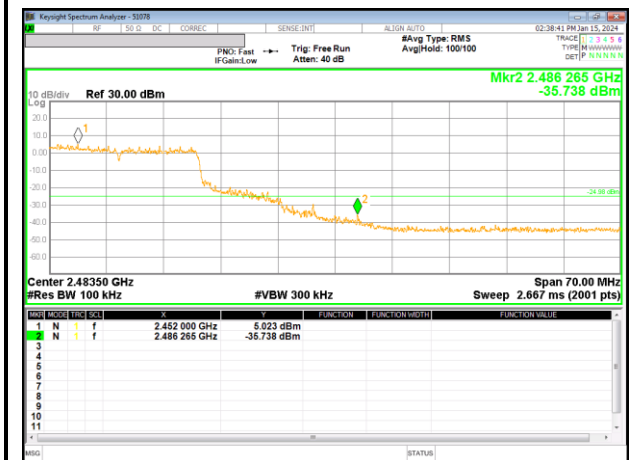
10 Channel Band-edge
