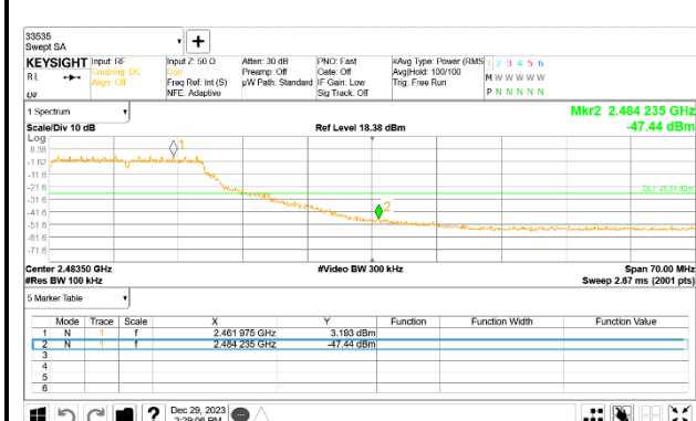
10 Channel Band-edge
