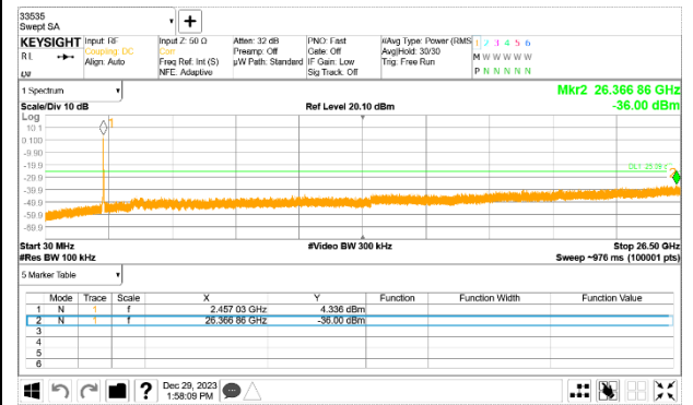
Out-Of-Band 9 Channel
