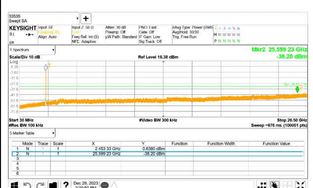
Out-Of-Band 10 Channel
