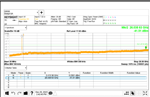
Out-Of-Band 2 Channel
