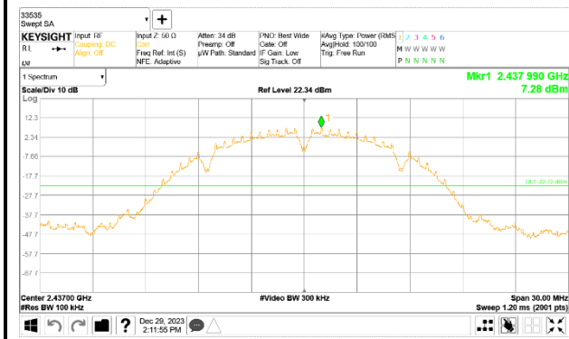
6 Channel Band-edge
