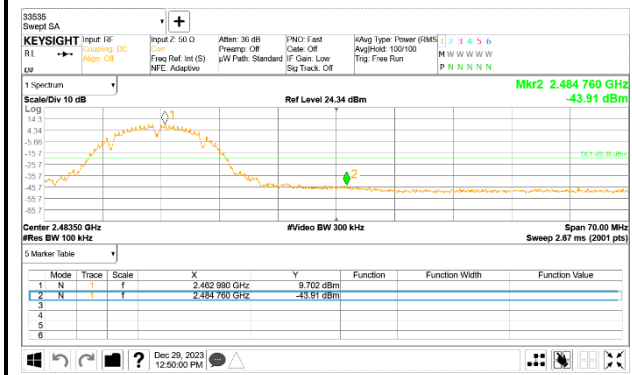
11 Channel Band-edge
