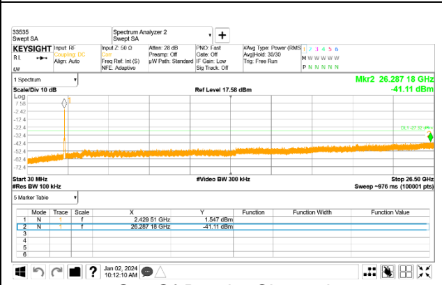
Out-Of-Band 6 Channel
