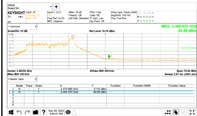
11 Channel Band-edge(8RU)
