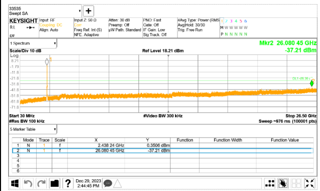
Out-Of-Band 6 Channel
