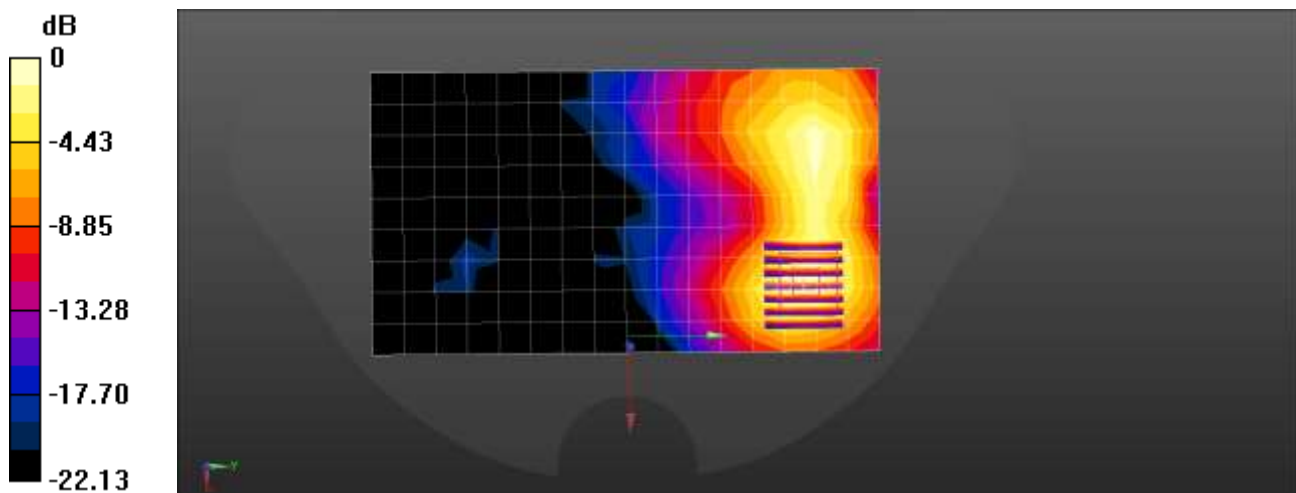
0 dB = 0.431 W/kg = -3.66 dBW/kg
