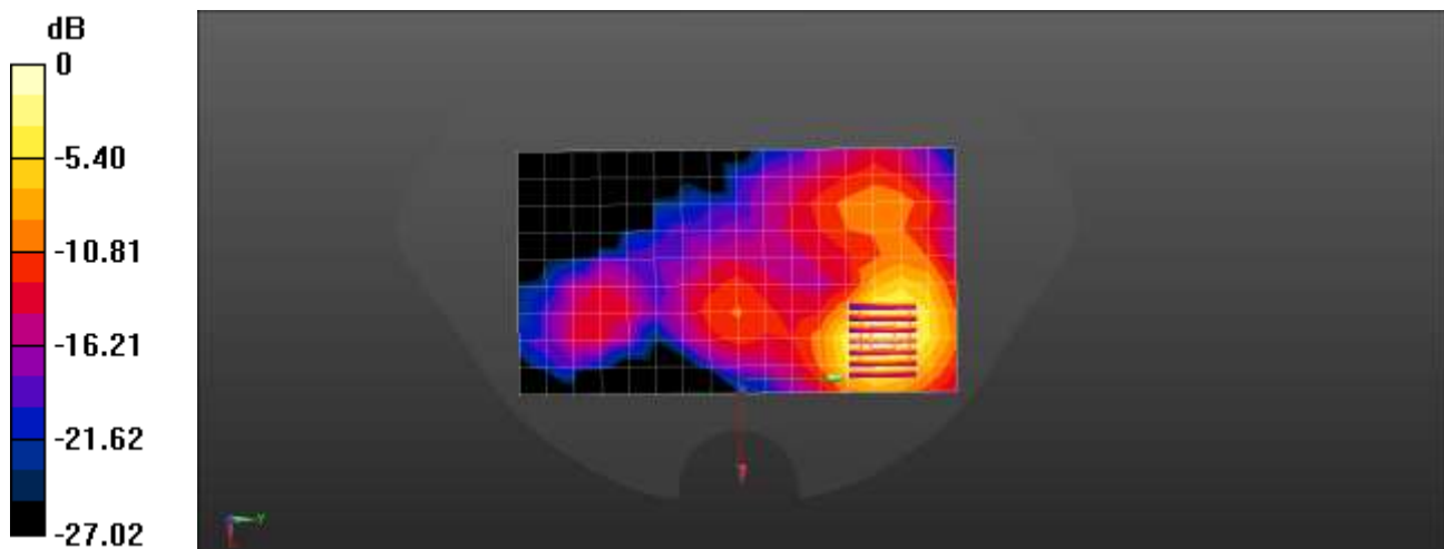
0 dB = 0.371 W/kg = -4.31 dBW/kg
