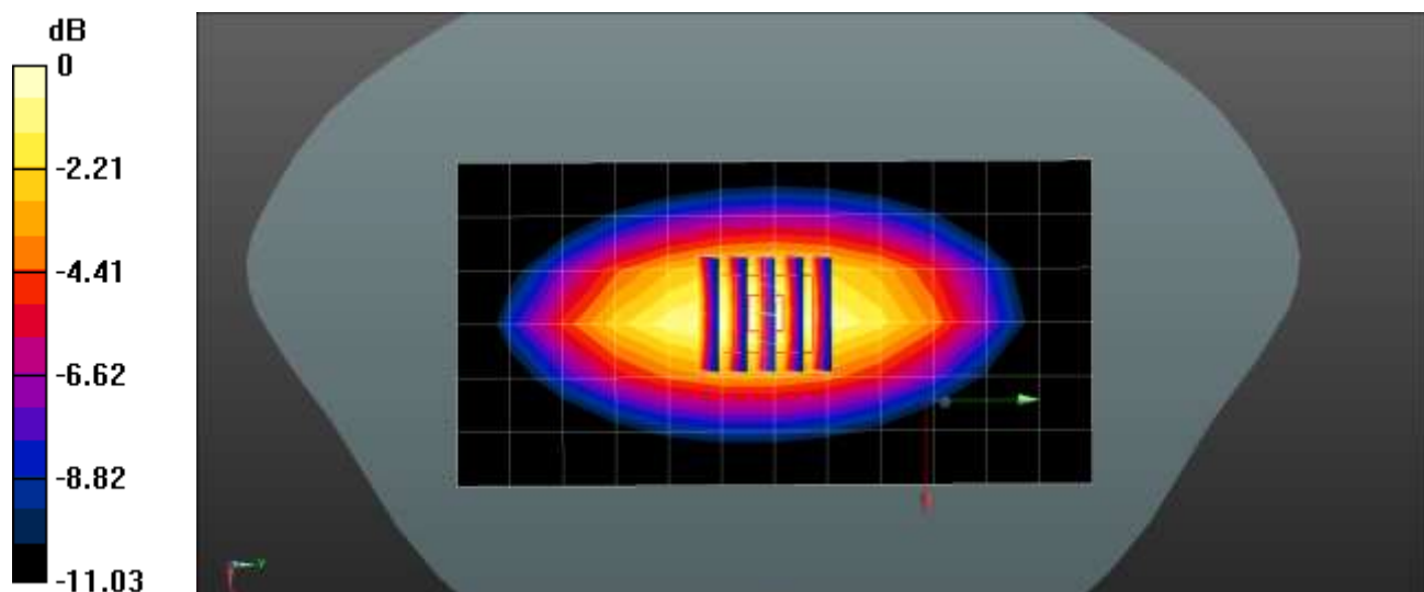
0 dB = 0.668 W/kg = -1.75 dBW/kg
