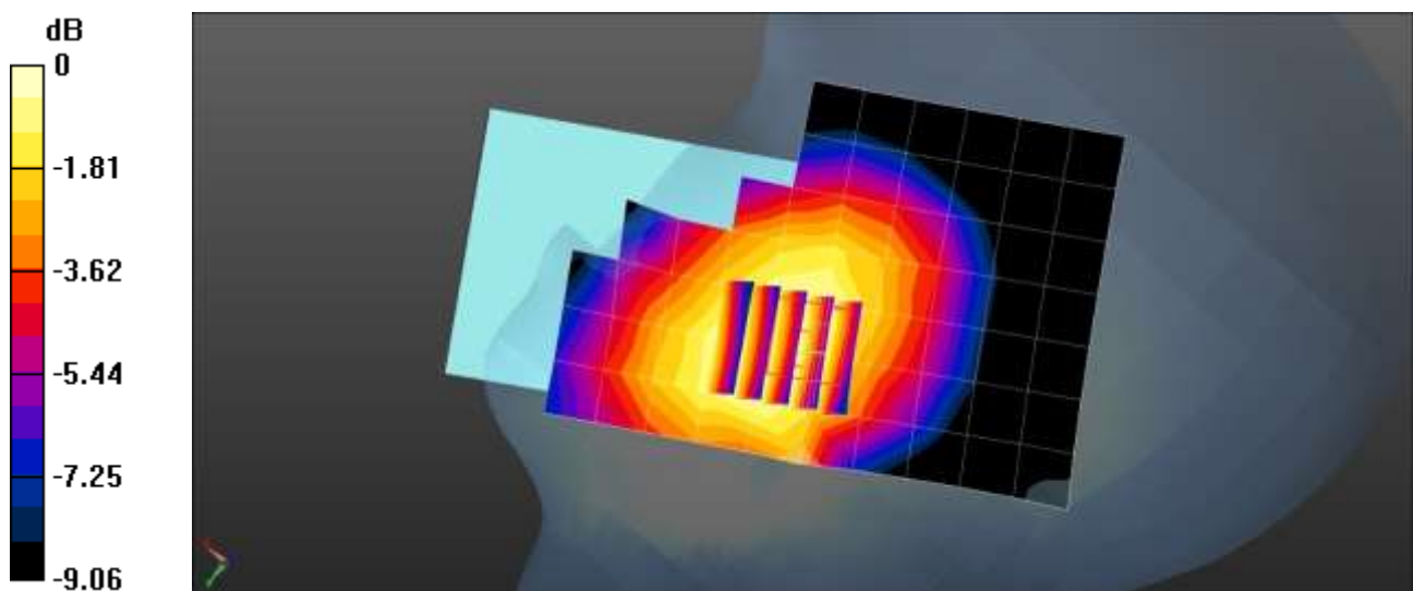
0 dB = 0.287 W/kg = -5.42 dBW/kg
