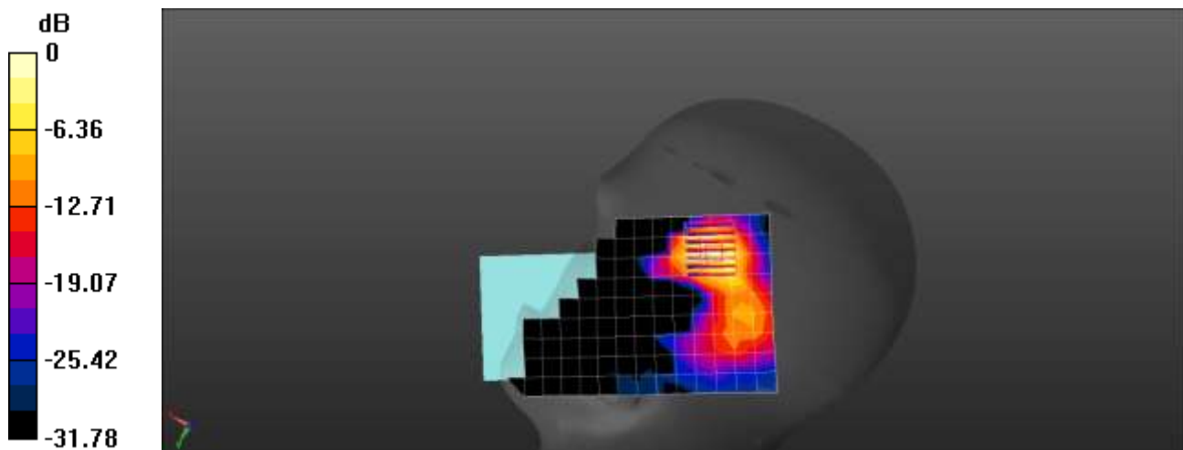
0 dB = 0.482 W/kg = -3.17 dBW/kg
