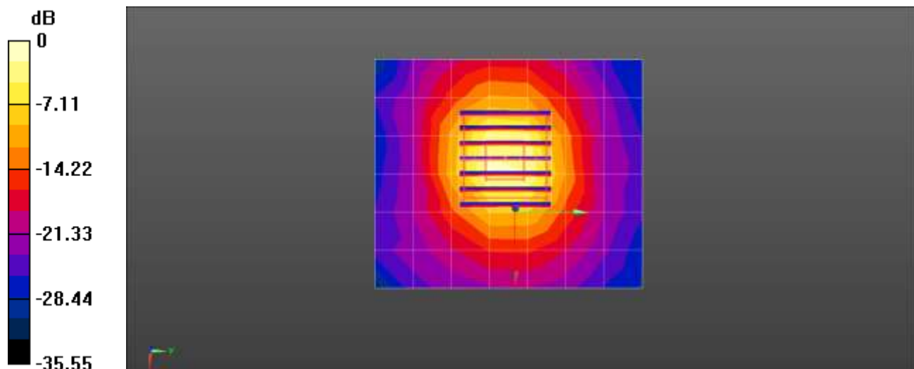
0 dB = 10.2 W/kg = 10.09 dBW/kg
