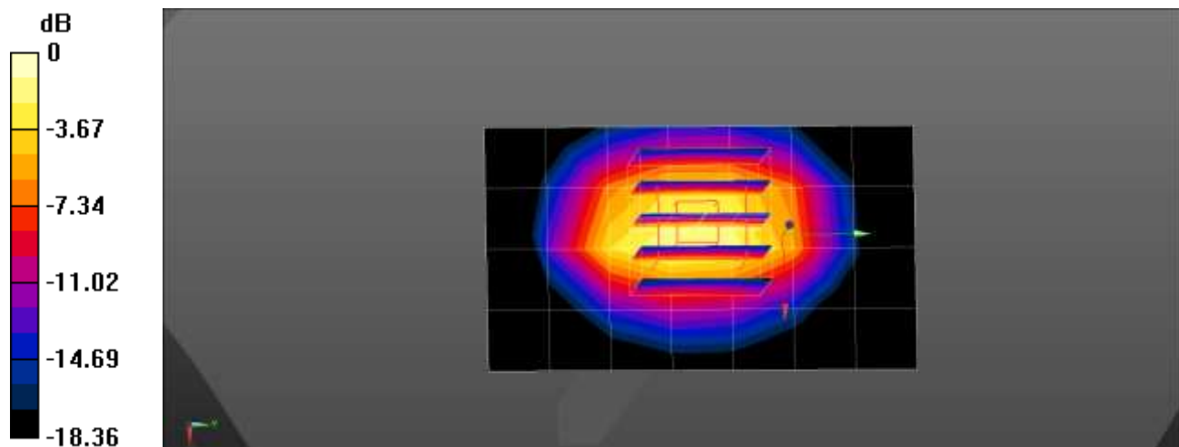
0 dB = 3.23 W/kg = 5.09 dBW/kg
