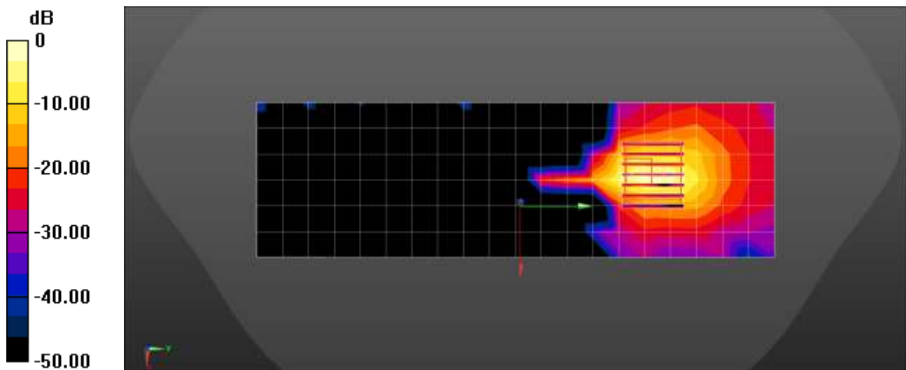
0 dB = 7.54 W/kg = 8.77 dBW/kg
