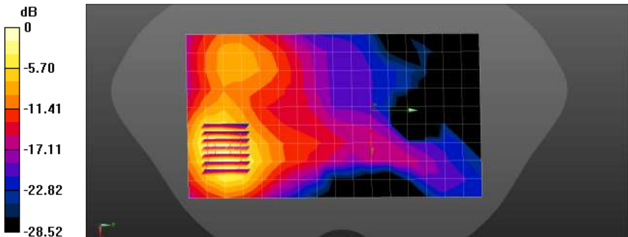
0 dB = 1.22 W/kg = 0.86 dBW/kg
