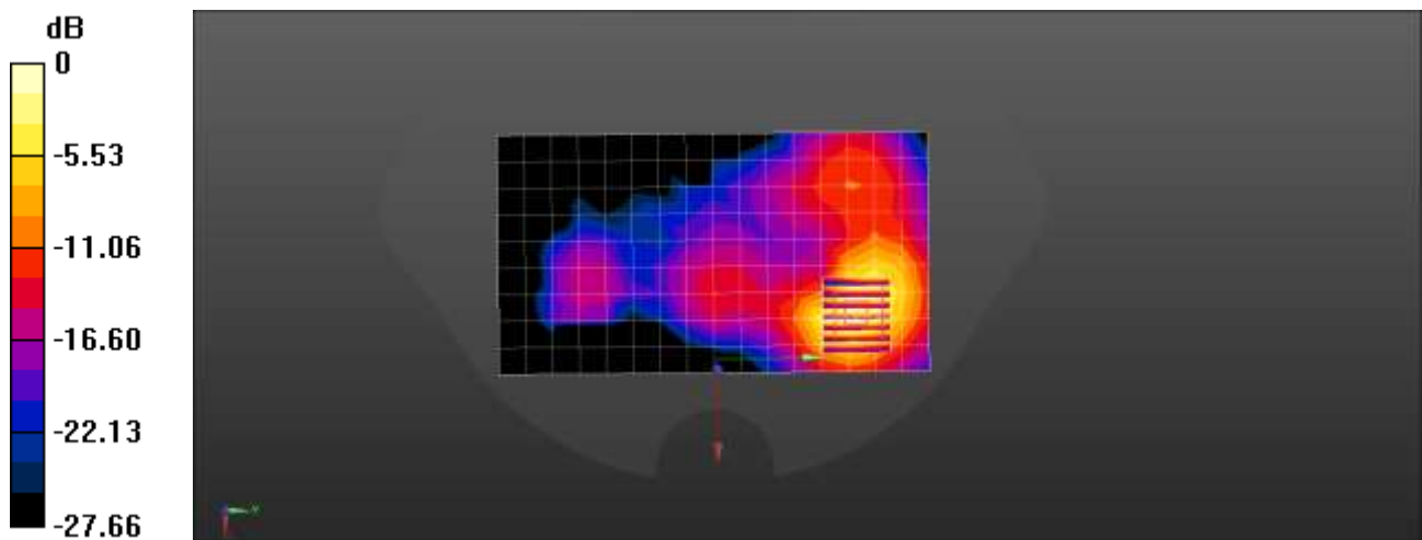
0 dB = 0.702 W/kg = -1.54 dBW/kg
