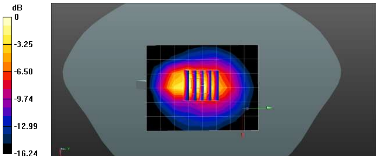
0 dB = 0.414 W/kg = -3.83 dBW/kg
