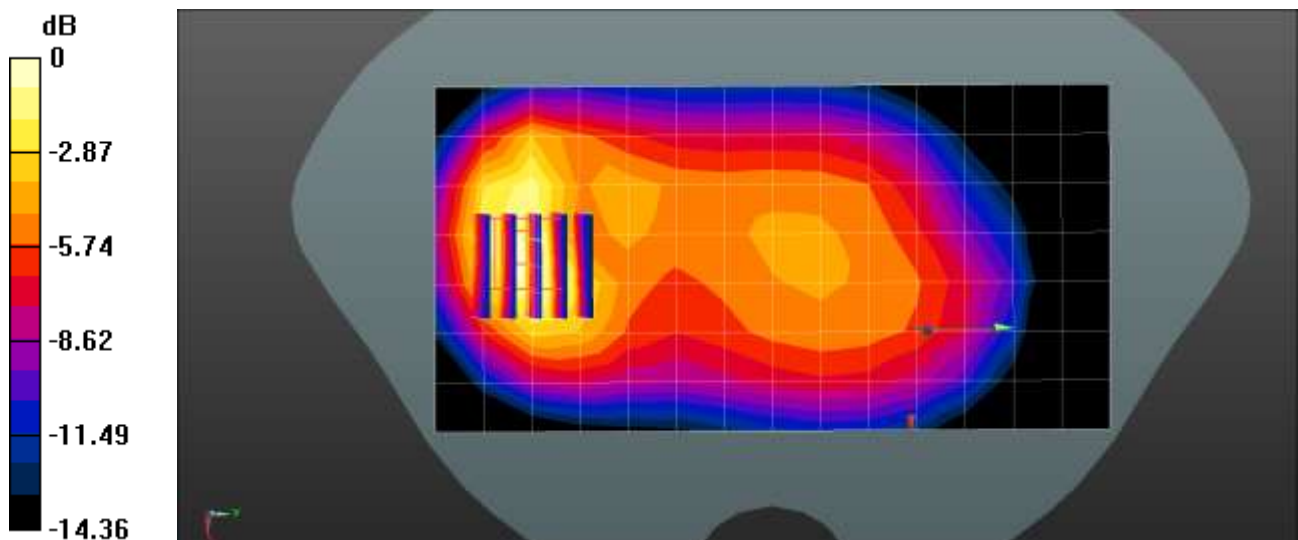
0 dB = 0.863 W/kg = -0.64 dBW/kg
