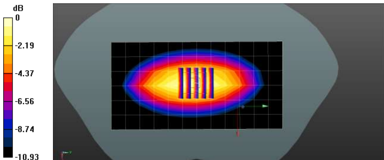
0 dB = 0.676 W/kg = -1.70 dBW/kg
