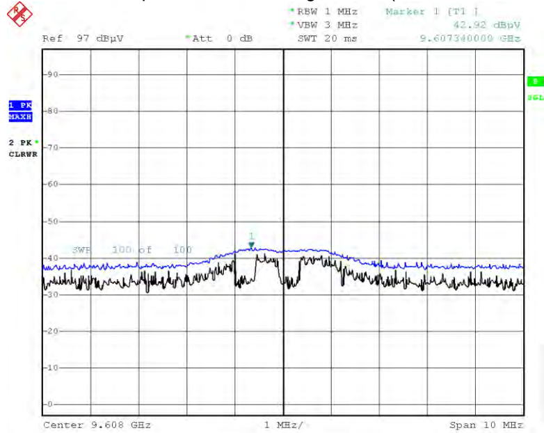
Radiated Spurious Emissions plot – Peak & Average Result (GFSK, Ch.0 4th Harmonic, Z-V)
