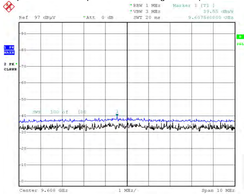
Radiated Spurious Emissions plot – Peak & Average Result (4th Harmonic, X-V)
