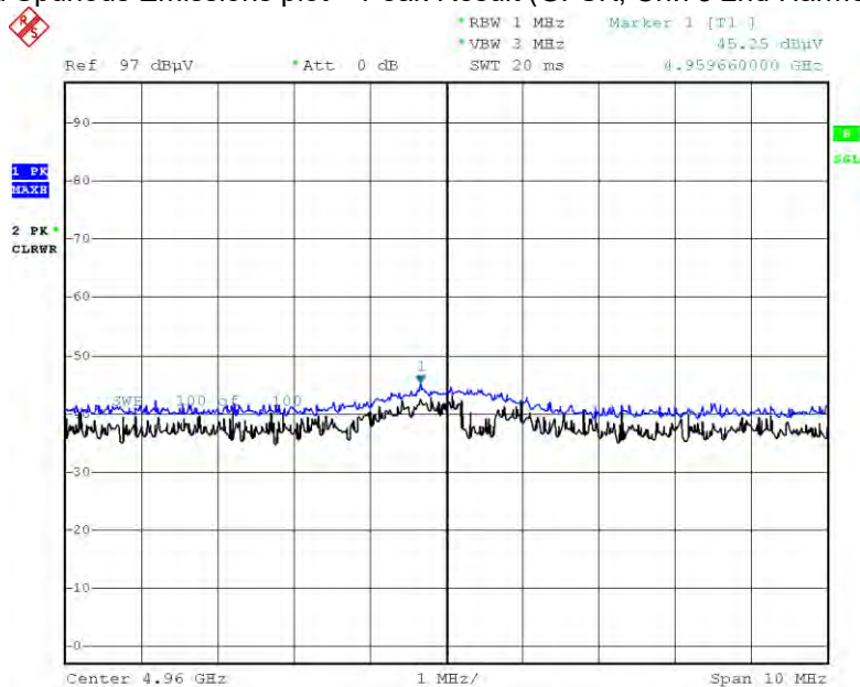
Radiated Spurious Emissions plot – Peak Result (GFSK, Ch.78 2nd Harmonic, X-H)
