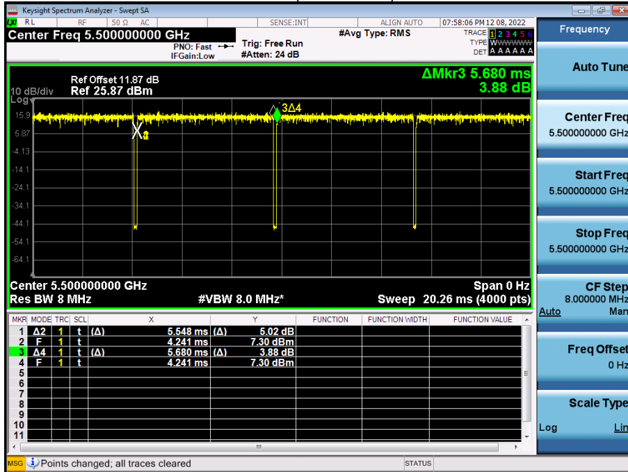
Bandwidth 20M Ch.100(5 500 MHz) 26 Tones MCS 0
