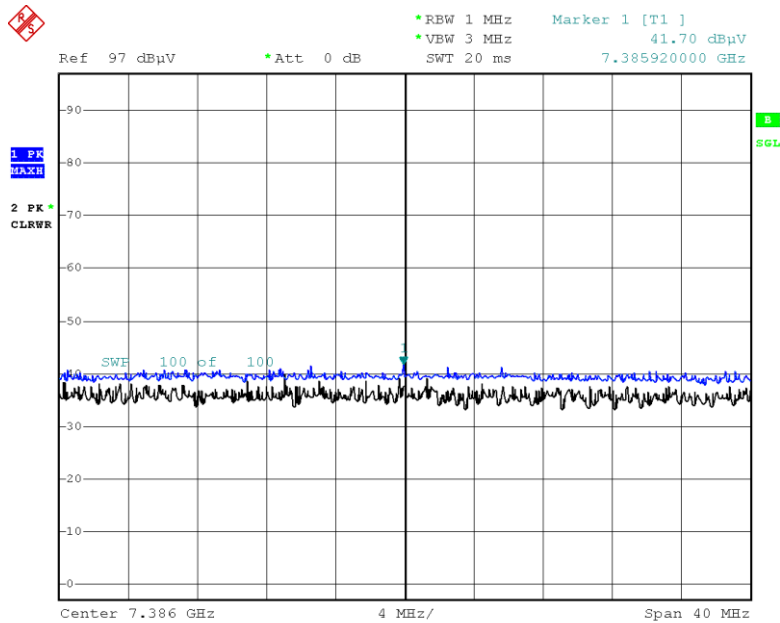
Radiated Spurious Emissions plot – Peak result (802.11ax(HE20)_SU, Ch.11 3rd Harmonic, X-V)
