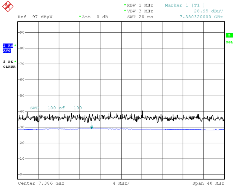
Radiated Spurious Emissions plot – Average result (802.11ax(HE20)_SU, Ch.11 3rd Harmonic, X-V)
