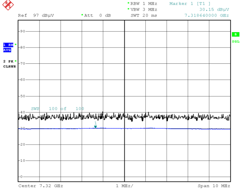
Radiated Spurious Emissions plot – Average Result (Ch. 19 3rd Harmonic)
