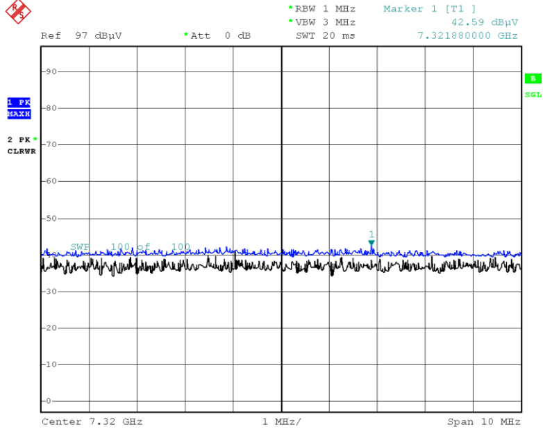
Radiated Spurious Emissions plot – Peak Result (Ch. 19 3rd Harmonic)
