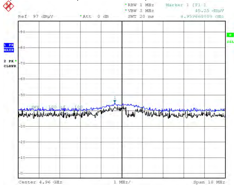
Radiated Spurious Emissions plot – Peak Result (GFSK, Ch.78 2nd Harmonic, X-H)
