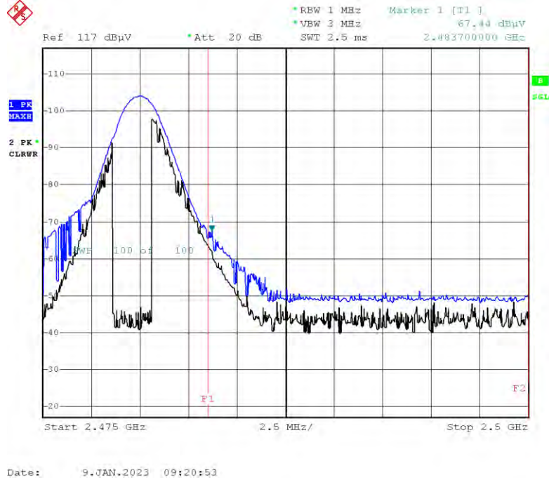
Radiated Restricted Band Edges plot – Average & Peak Result (8DPSK, Ch.78, X-H)
