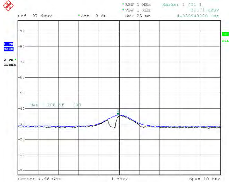
Radiated Spurious Emissions plot – Average Result (GFSK, Ch.78 2nd Harmonic, X-H)
