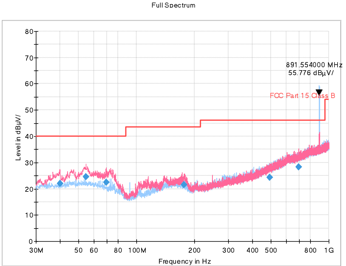
Figure 1: Radiated Emission (30 to 1 000) MHz, [EUT+TA] LTE B5 High ch Idle
