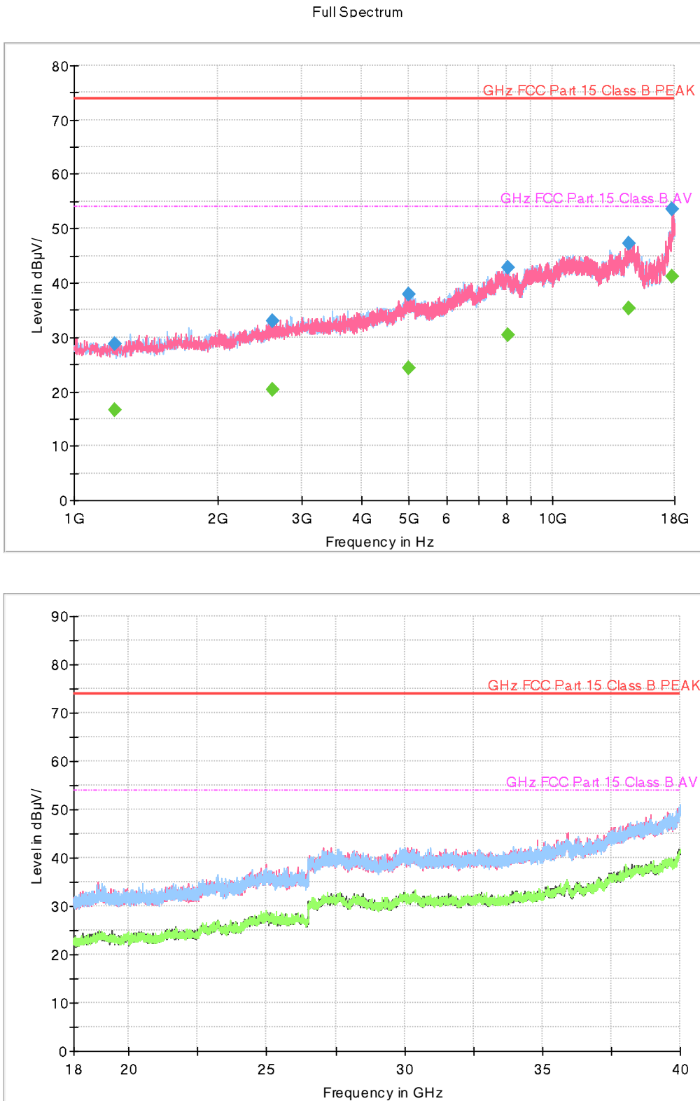
Figure 5: Radiated Emission (1 to 40) GHz, [EUT+TA] LTE B5 High ch Idle
