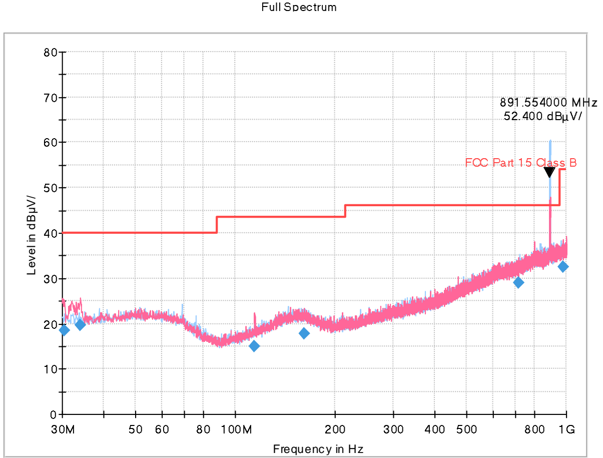
Figure 4: Radiated Emission (30 to 1 000) MHz, [EUT+Earphone] LTE B5 High ch Idle
