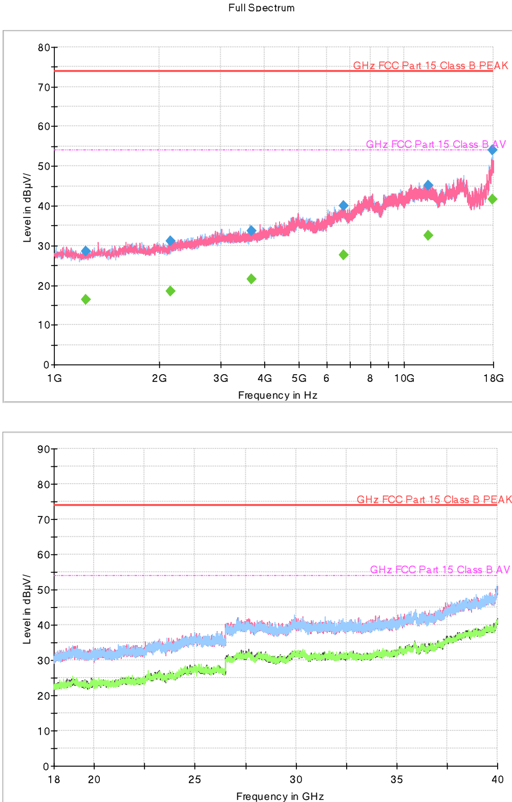
Figure 6: Radiated Emission (1 to 40) GHz, [EUT+Earphone] LTE B5 High ch Idle
