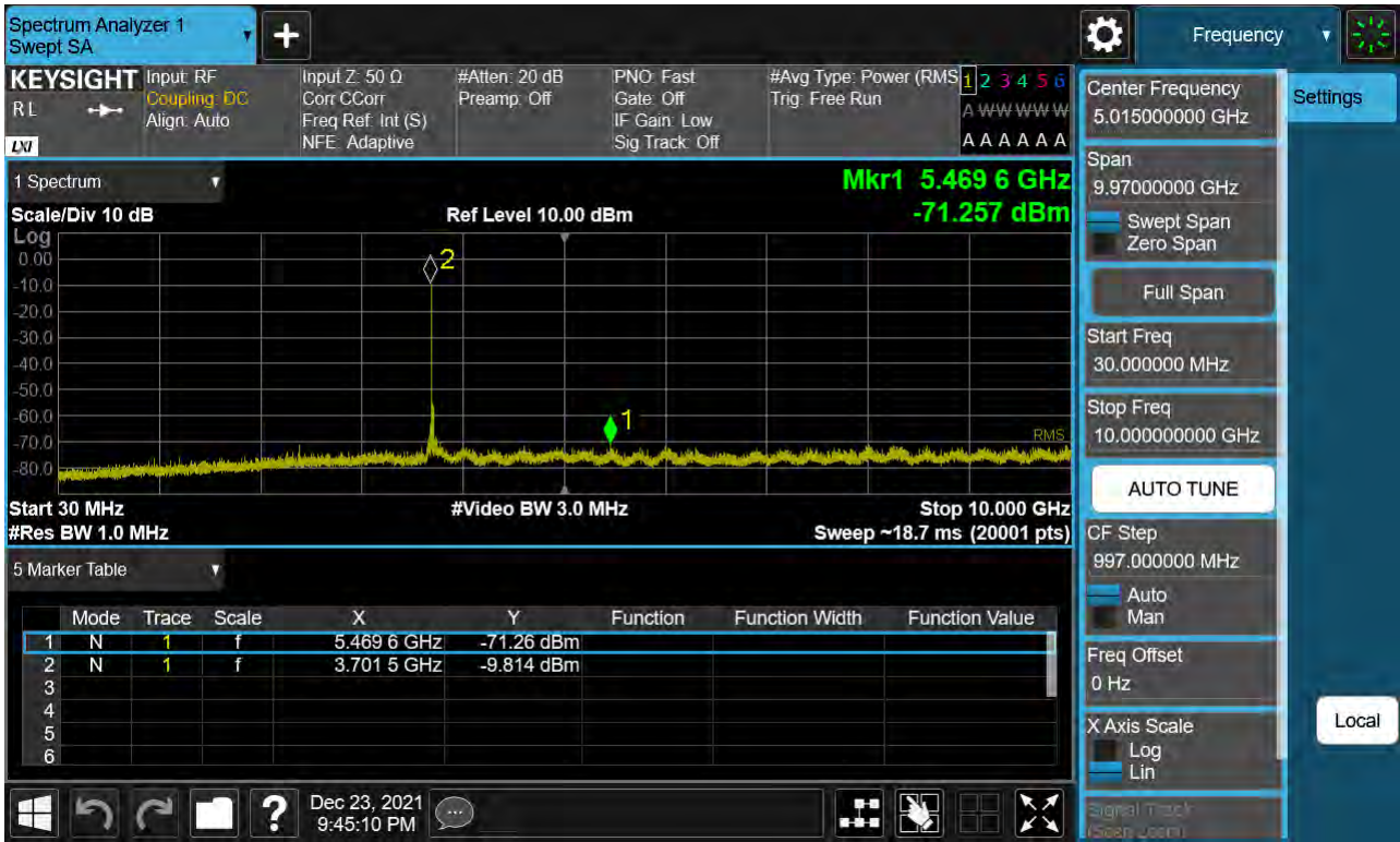
Sub6 n77. Conducted Spurious Plot_1 (647668ch_30 MHz_BPSK)
