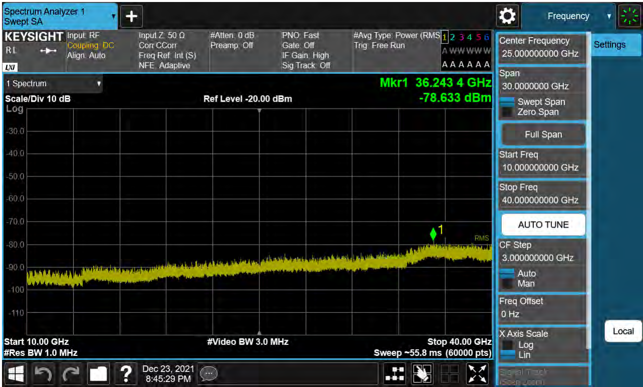
Sub6 n77. Conducted Spurious Plot_2 (665000ch_10 MHz_BPSK)
