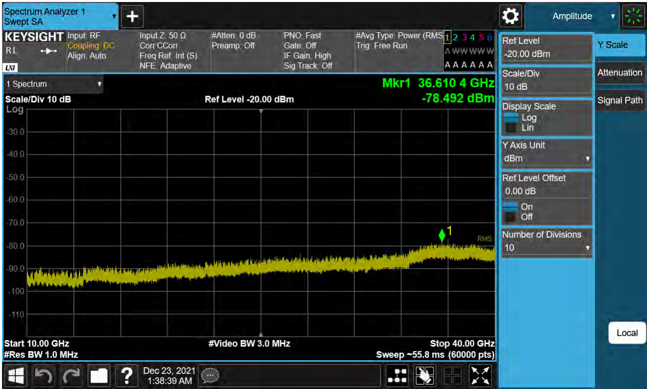
Sub6 n77. Conducted Spurious Plot_2 (633334ch_15 MHz_BPSK)
