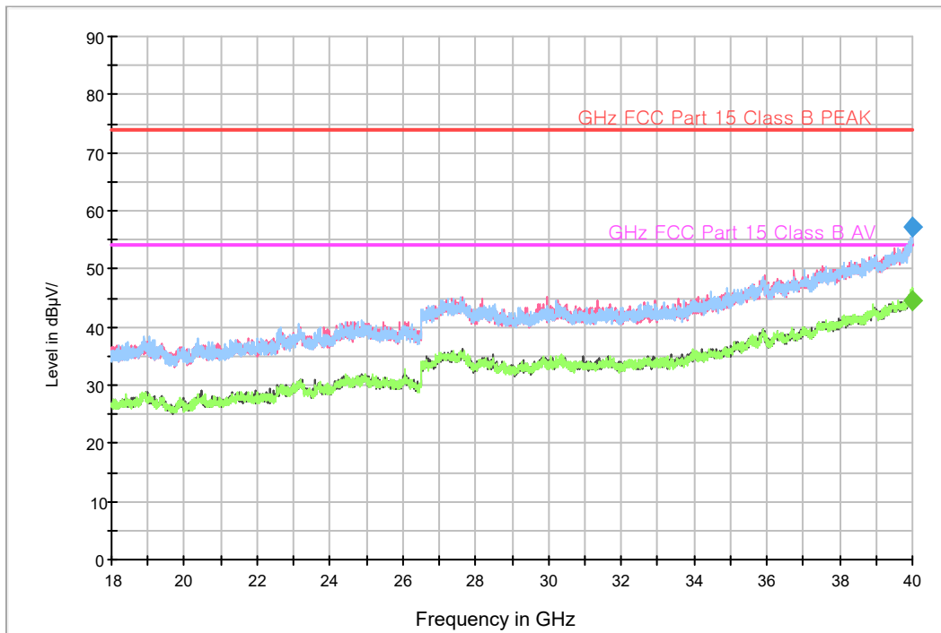
Tilting of GHz FCC PART 15 CLASS B_18~40GHz
