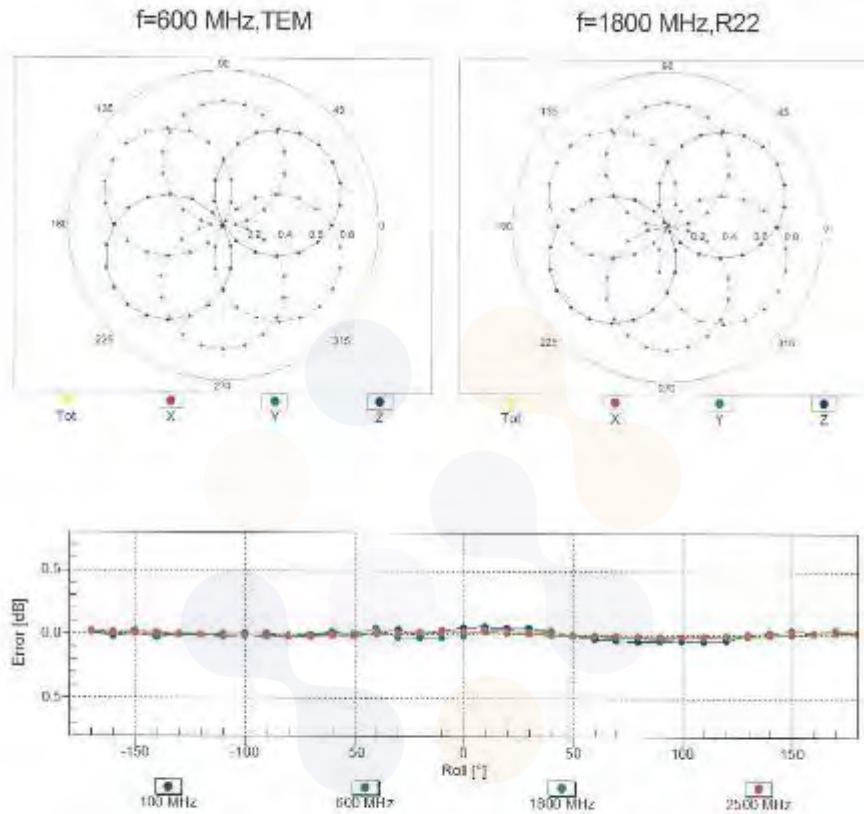
Uncertainty of Axial Isotropy Assessment: \pm 0.5\% ( k=2 )
