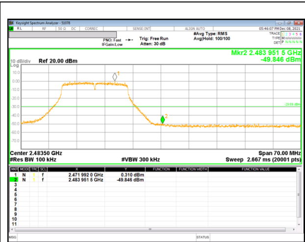
12 Channel Band-edge
