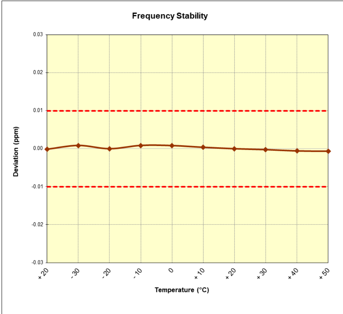
Figure 7-3. Frequency Stability Plot
