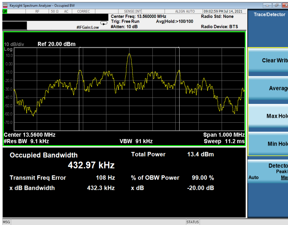
Figure 7-2. Occupied Bandwidth Plot
