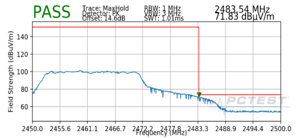
Plot 7-52. Radiated Restricted Upper Band Edge Measurement (Peak – 242 Tones)
