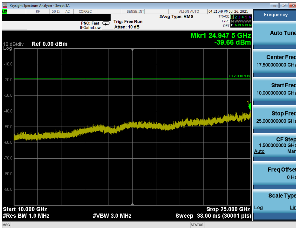
Plot 7-24. Conducted Spurious Plot (802.11ax OFDMA – 26 Tones – Ch. 6)
