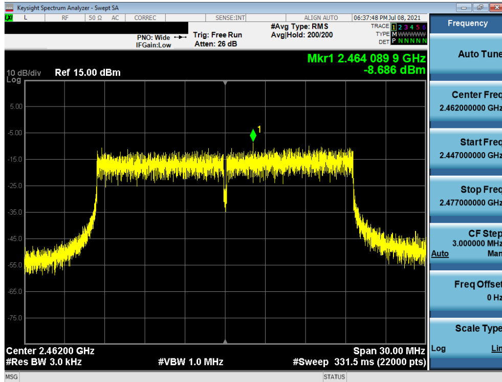
Plot 7-12. Power Spectral Density Plot (802.11ax OFDMA – 242 Tones – Ch. 11)
