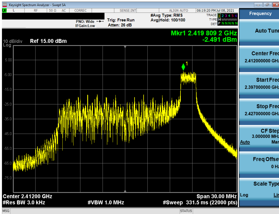
Plot 7-7. Power Spectral Density Plot (802.11ax OFDMA – 26 Tones – Ch. 1)
