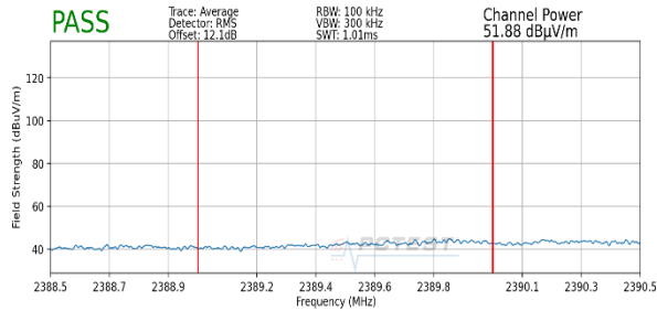
Plot 7-49. Radiated Restricted Lower Band Edge Measurement (Average – 242 Tones)
