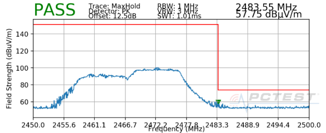
Plot 7-46. Radiated Restricted Upper Band Edge Measurement (Peak – 106 Tones)
