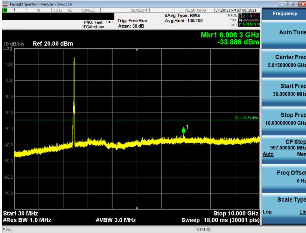
Plot 7-31. Conducted Spurious Plot (802.11ax OFDMA – 242 Tones – Ch. 11)
