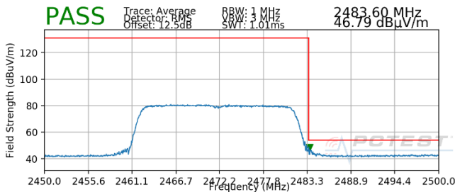
Plot 7-55. Radiated Restricted Upper Band Edge Measurement (Average – 242 Tones)
