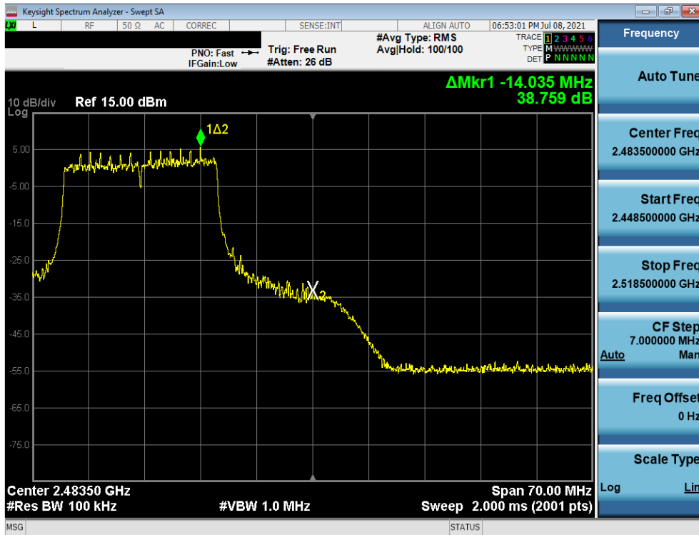
Plot 7-18. Band Edge Plot (802.11ax OFDMA – 242 Tones – Ch. 11)
