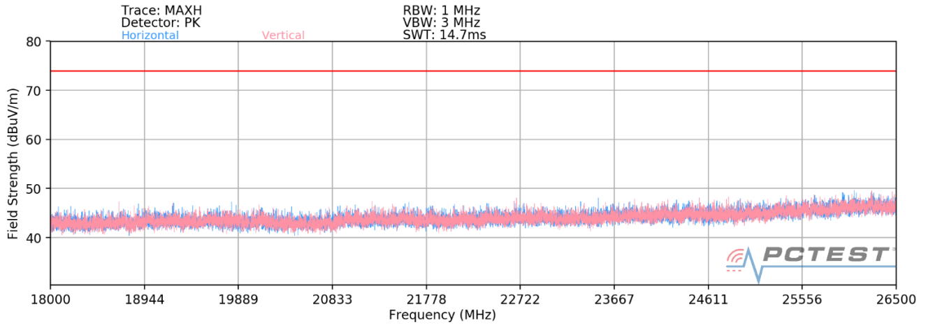
Plot 7-39. Radiated Spurious Plot above 18GHz (802.11ax OFDMA – 106 Tones)
