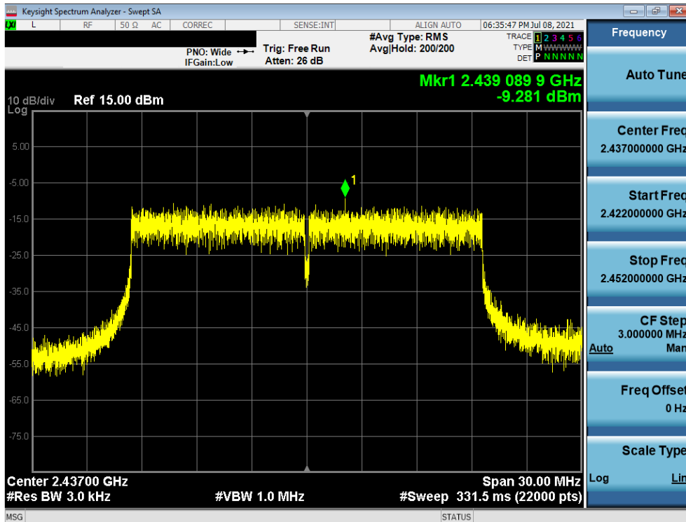
Plot 7-11. Power Spectral Density Plot (802.11ax OFDMA – 242 Tones – Ch. 6)
