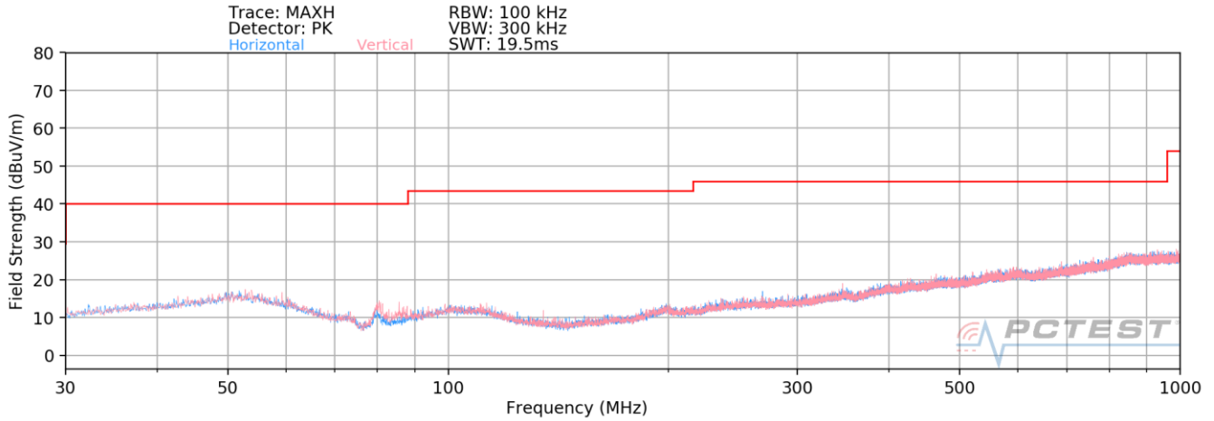
Plot 7-57. Radiated Spurious Plot below 1GHz (106 Tones)
