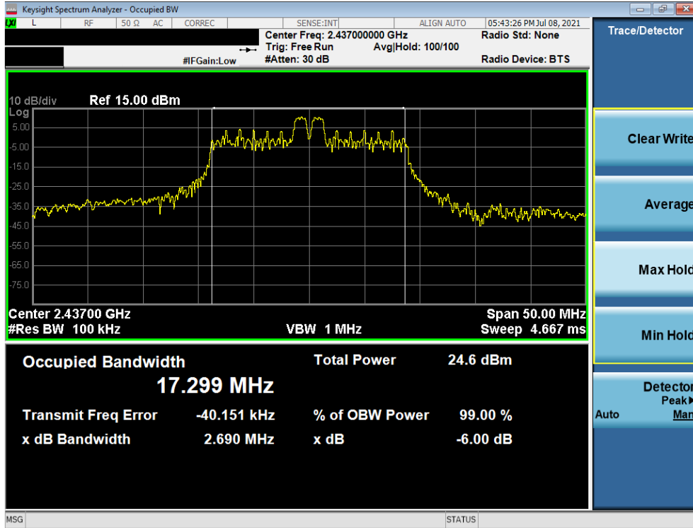
Plot 7-2. 6dB Bandwidth Plot (802.11ax OFDMA – 26 Tones – Ch. 6)
