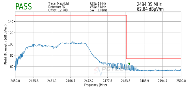
Plot 7-44. Radiated Restricted Upper Band Edge Measurement (Peak – 106 Tones)
