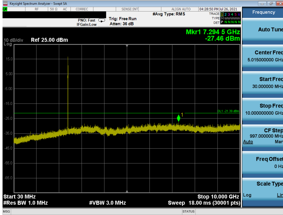
Plot 7-21. Conducted Spurious Plot (802.11ax OFDMA – 26 Tones – Ch. 1)
