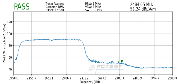
Plot 7-51. Radiated Restricted Upper Band Edge Measurement (Average – 242 Tones)
