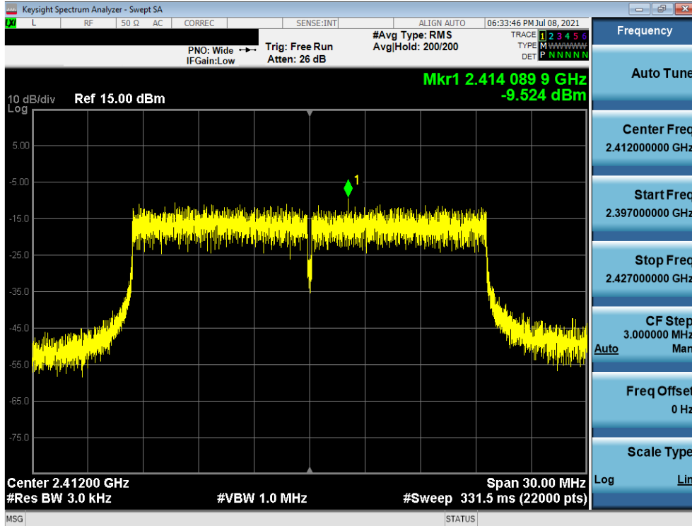
Plot 7-10. Power Spectral Density Plot (802.11ax OFDMA – 242 Tones – Ch. 1)
