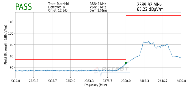
Plot 7-42. Radiated Restricted Lower Band Edge Measurement (Peak – 106 Tones)
