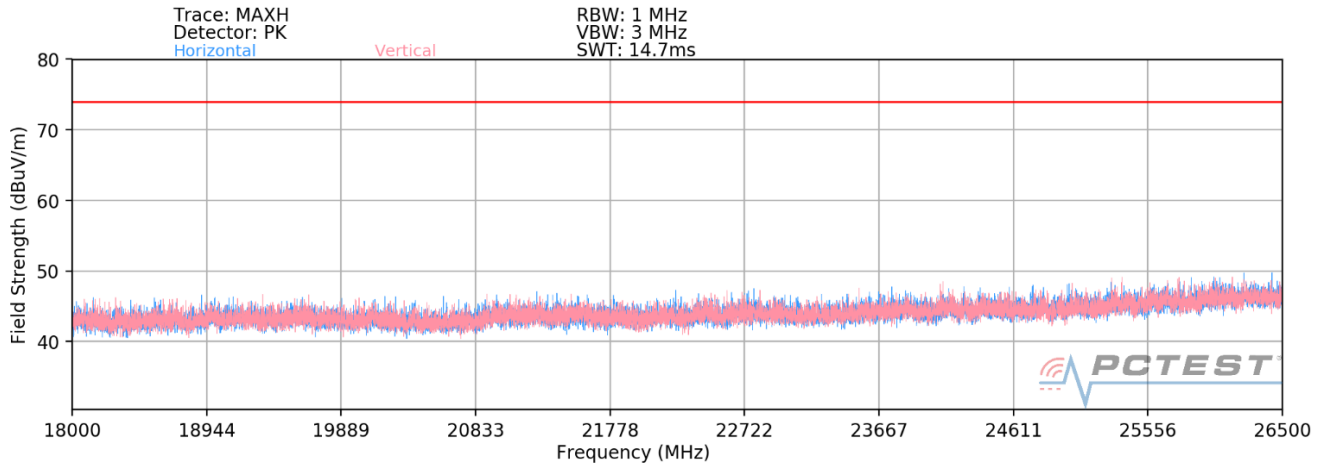
Plot 7-40. Radiated Spurious Plot above 18GHz (802.11ax OFDMA – 242 Tones)
