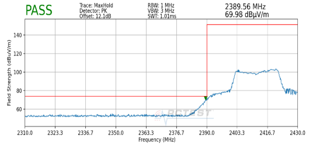
Plot 7-50. Radiated Restricted Lower Band Edge Measurement (Peak – 242 Tones)
