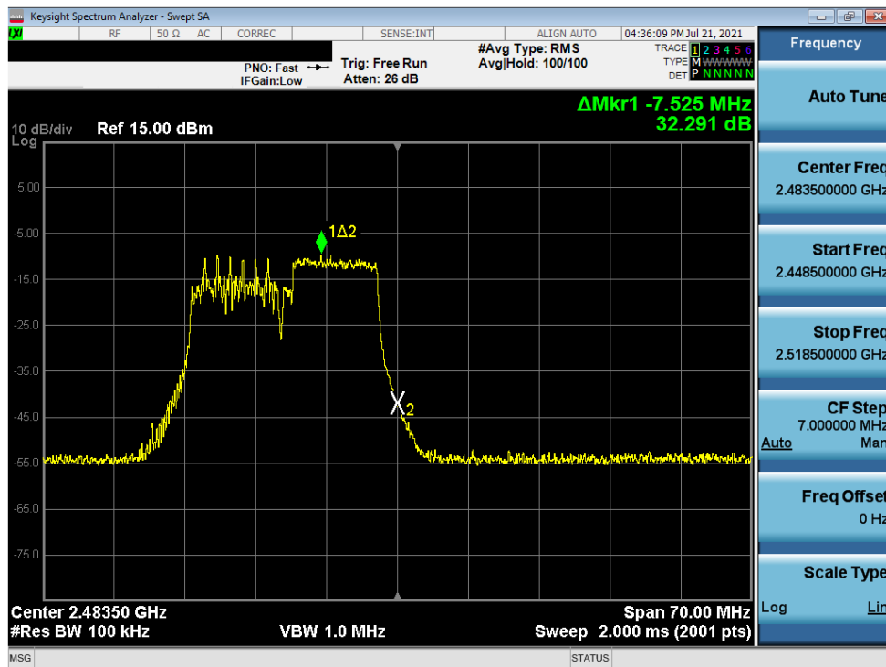
Plot 7-16. Band Edge Plot (802.11ax OFDMA – 106 Tones – Ch. 13)
