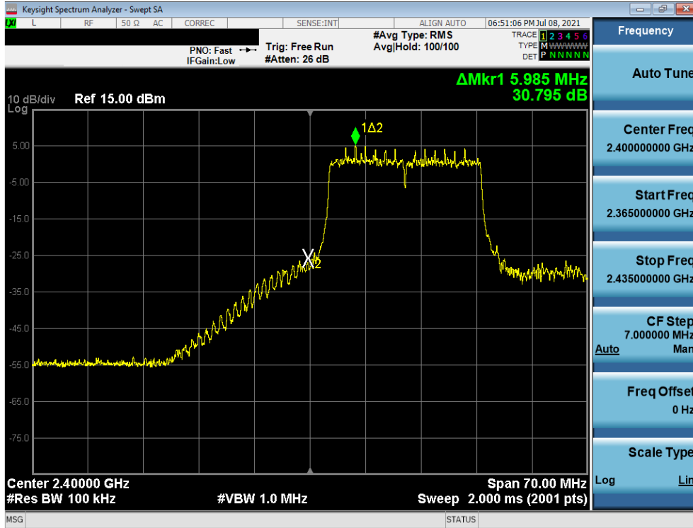
Plot 7-17. Band Edge Plot (802.11ax OFDMA – 242 Tones – Ch. 1)
