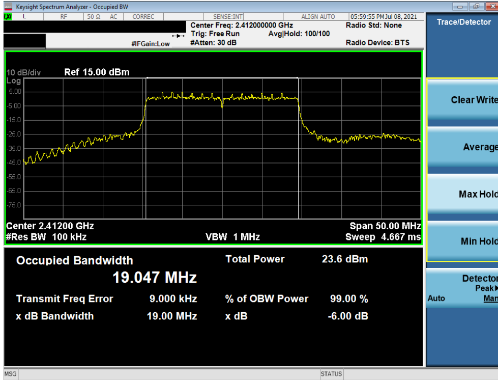
Plot 7-4. 6dB Bandwidth Plot (802.11ax OFDMA – 242 Tones – Ch. 1)
