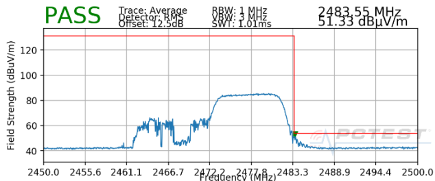
Plot 7-47. Radiated Restricted Upper Band Edge Measurement (Average – 106 Tones)
