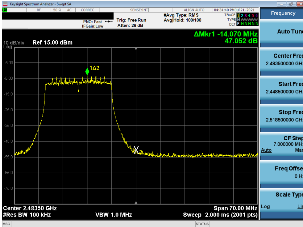
Plot 7-19. Band Edge Plot (802.11ax OFDMA – 242 Tones – Ch. 12)
