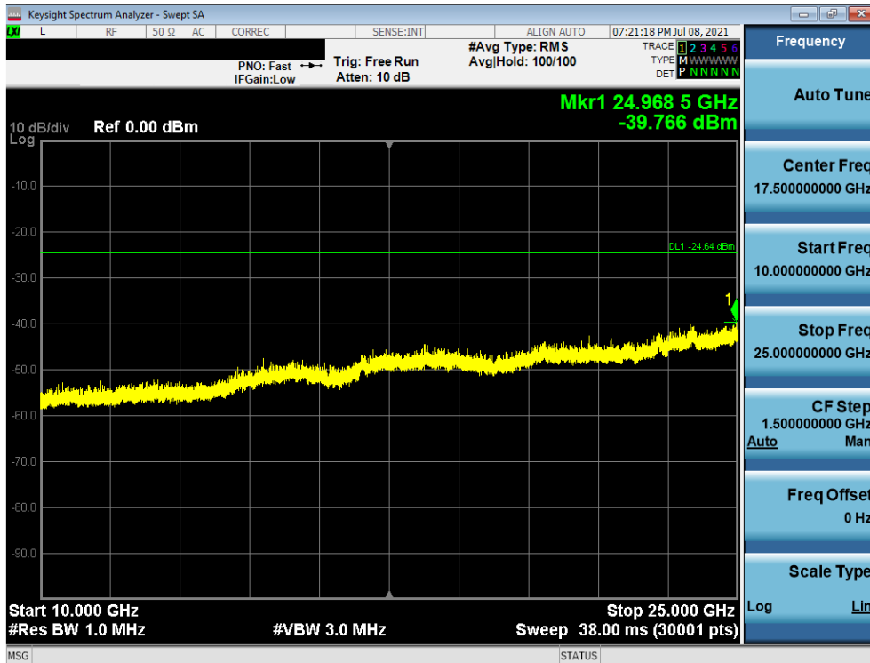
Plot 7-32. Conducted Spurious Plot (802.11ax OFDMA – 242 Tones – Ch. 11)
