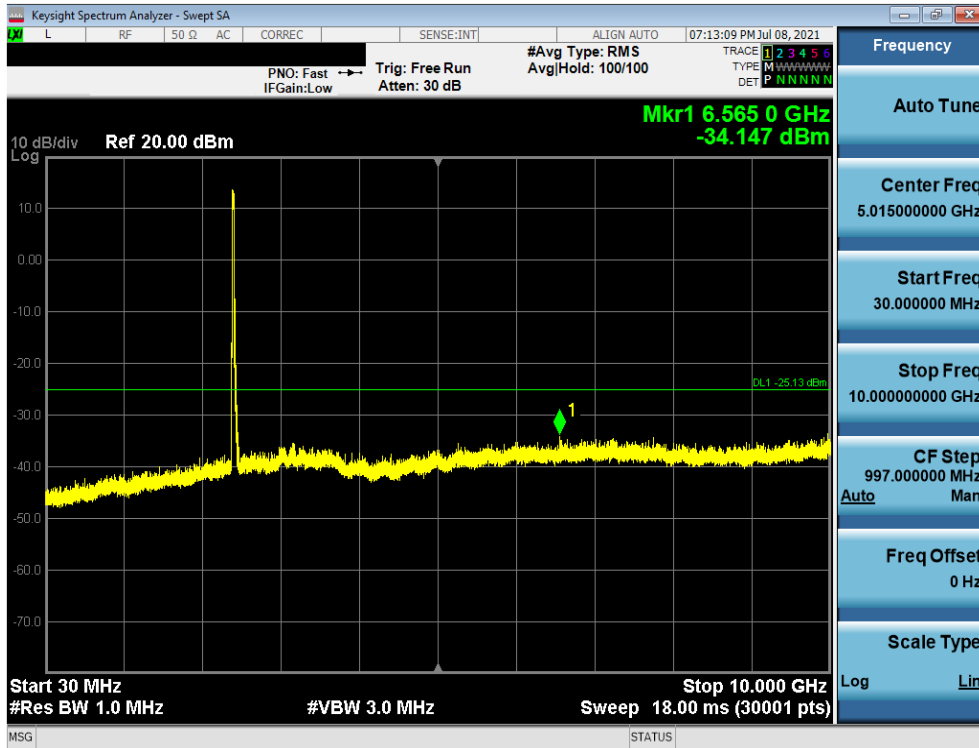
Plot 7-27. Conducted Spurious Plot (802.11ax OFDMA – 242 Tones – Ch. 1)
