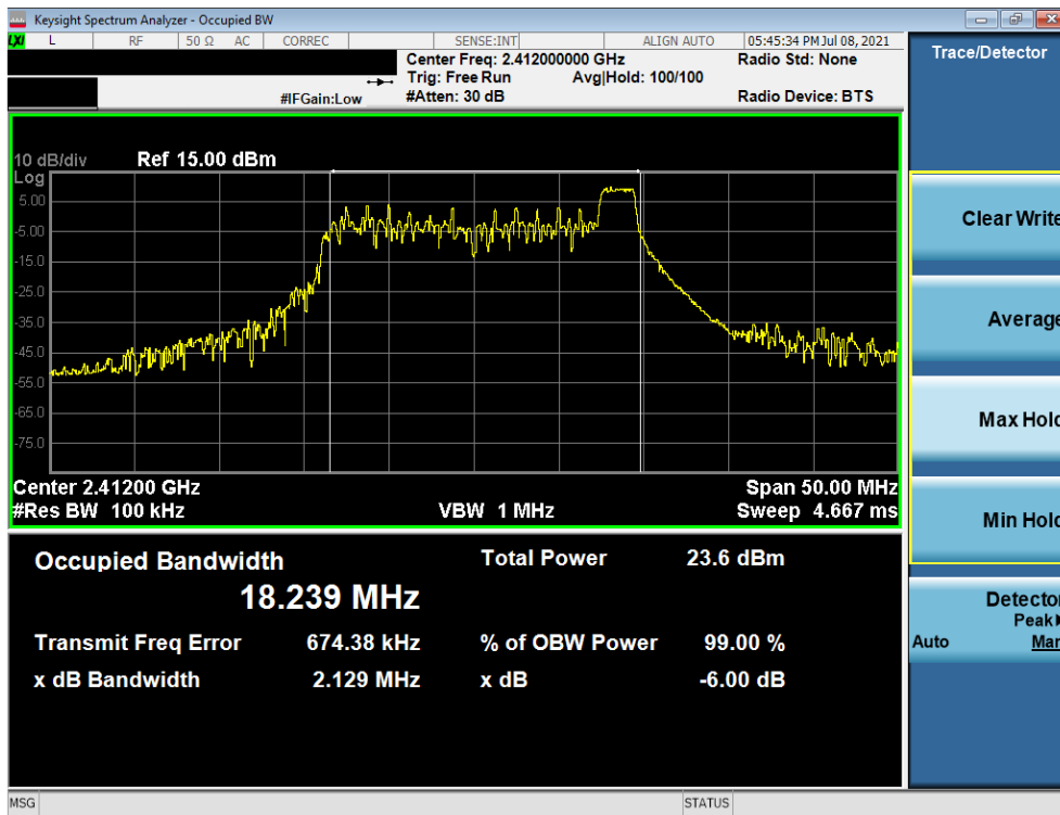
Plot 7-1. 6dB Bandwidth Plot (802.11ax OFDMA – 26 Tones – Ch. 1)
