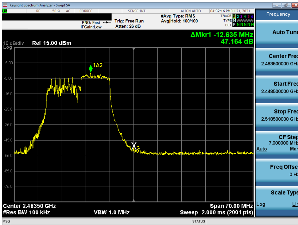
Plot 7-15. Band Edge Plot (802.11ax OFDMA – 106 Tones – Ch. 12)
