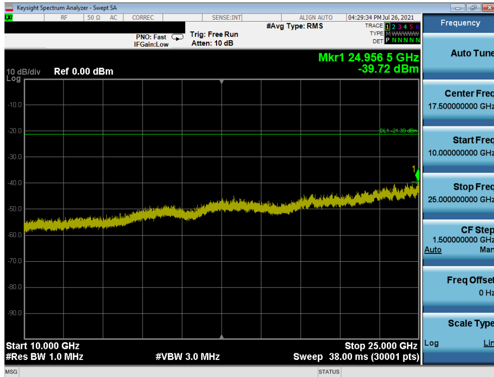
Plot 7-22. Conducted Spurious Plot (802.11ax OFDMA – 26 Tones – Ch. 1)
