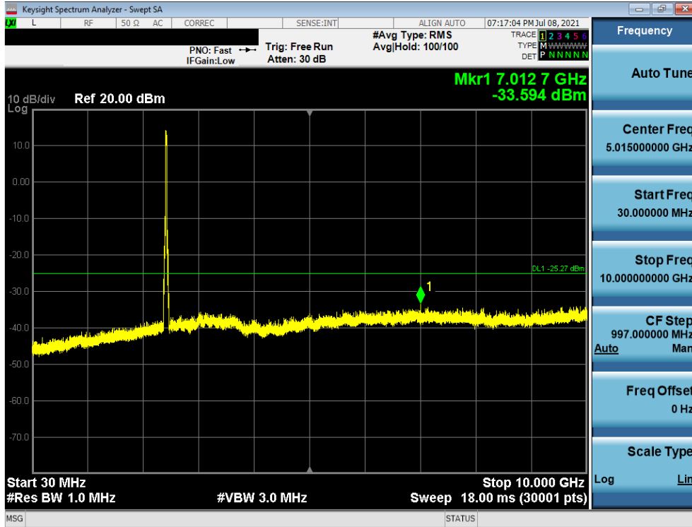
Plot 7-29. Conducted Spurious Plot (802.11ax OFDMA – 242 Tones – Ch. 6)
