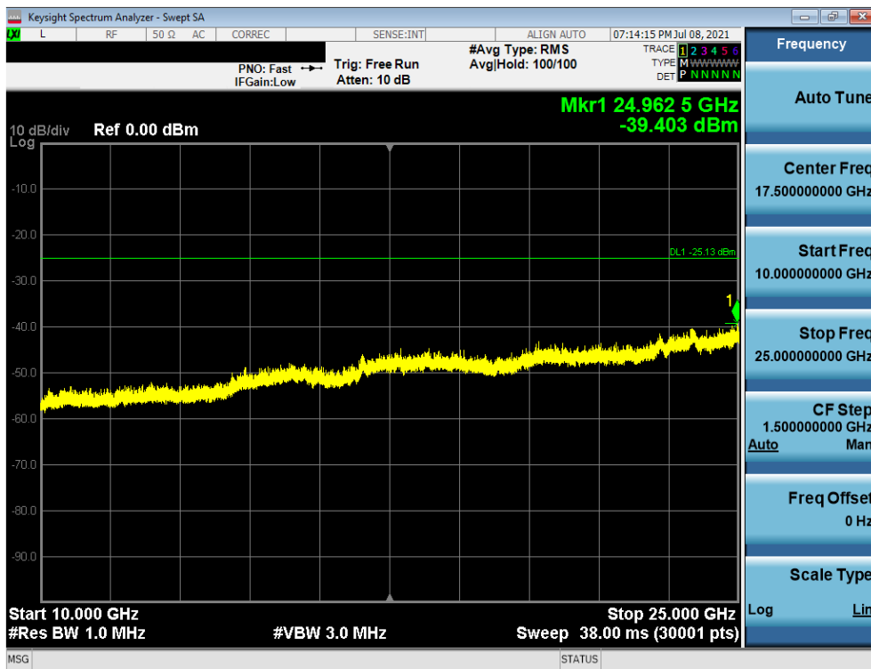
Plot 7-28. Conducted Spurious Plot (802.11ax OFDMA – 242 Tones – Ch. 1)
