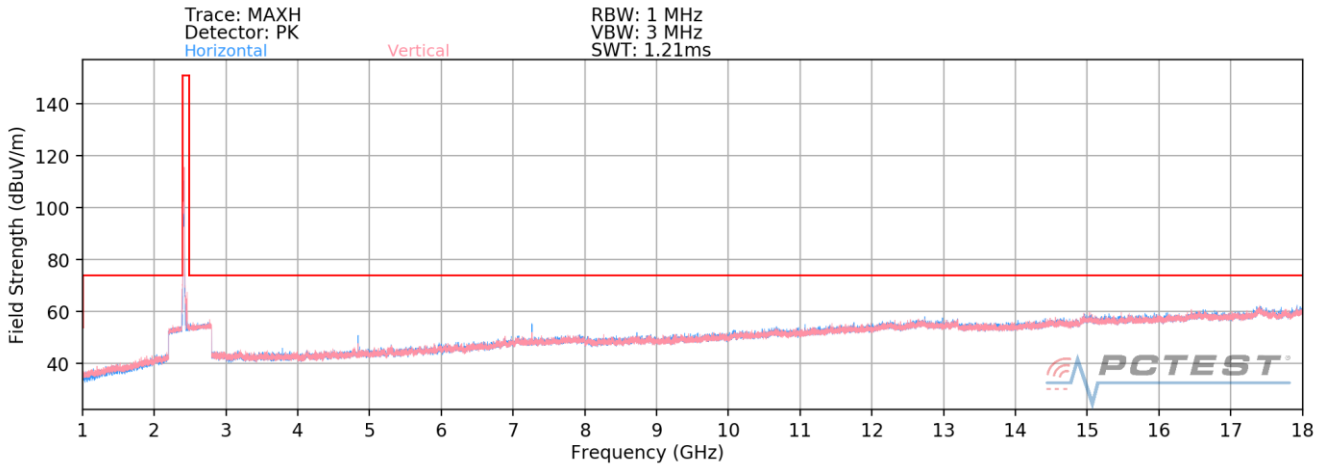
Plot 7-33. Radiated Spurious Plot above 1GHz (802.11ax OFDMA – 106 Tones – Ch. 1)
