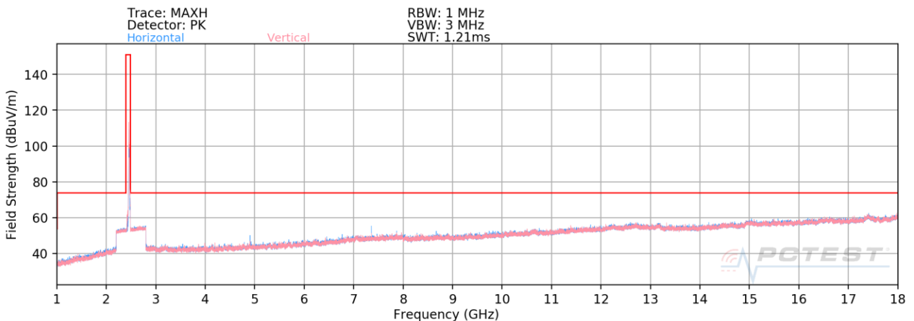
Plot 7-35. Radiated Spurious Plot above 1GHz (802.11ax OFDMA – 106 Tones – Ch. 11)
