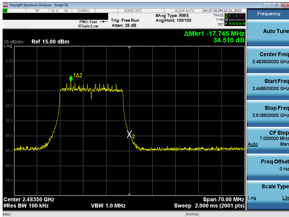
Plot 7-20. Band Edge Plot (802.11ax OFDMA – 242 Tones – Ch. 13)
