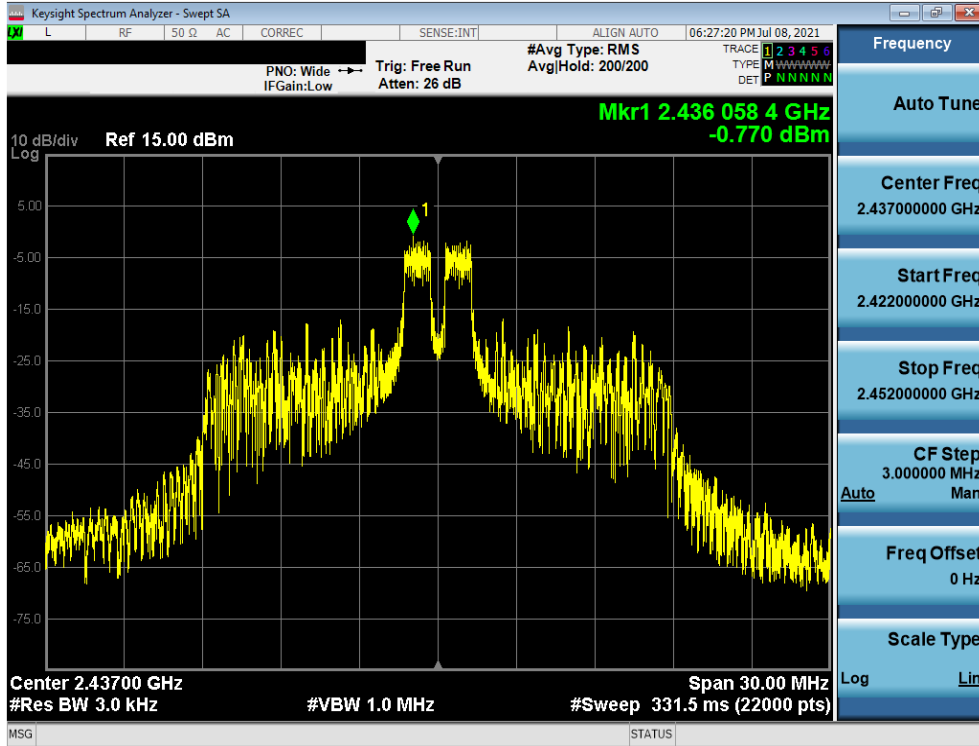
Plot 7-8. Power Spectral Density Plot (802.11ax OFDMA – 26 Tones – Ch. 6)
