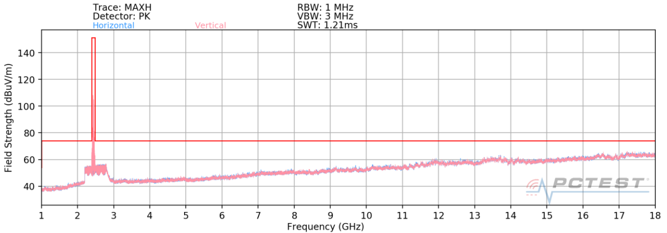
Plot 7-37. Radiated Spurious Plot above 1GHz (802.11ax OFDMA – 242 Tones – Ch. 6)
