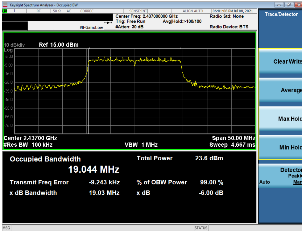
Plot 7-5. 6dB Bandwidth Plot (802.11ax OFDMA – 242 Tones – Ch. 6)
