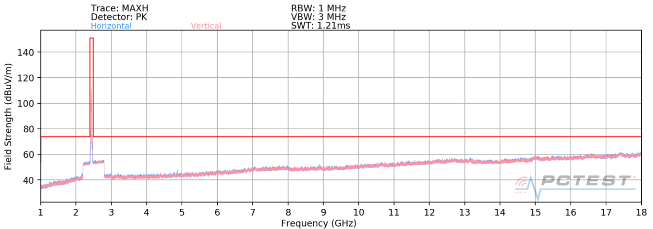
Plot 7-34. Radiated Spurious Plot above 1GHz (802.11ax OFDMA – 106 Tones – Ch. 6)
