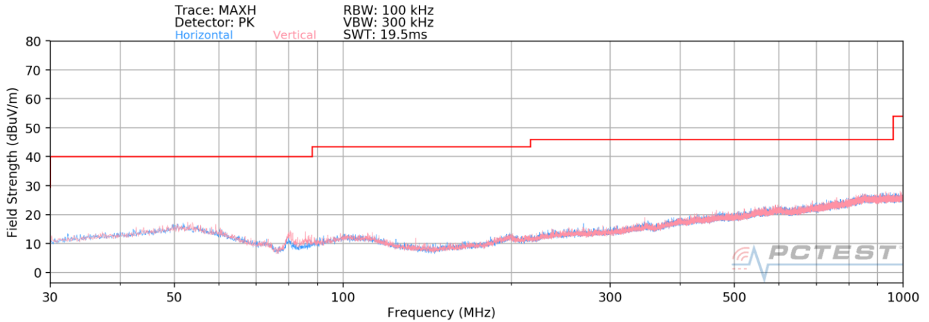
Plot 7-58. Radiated Spurious Plot below 1GHz (242 Tones)
