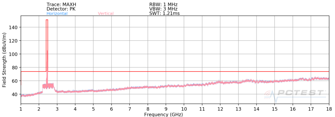
Plot 7-38. Radiated Spurious Plot above 1GHz (802.11ax OFDMA – 242 Tones – Ch. 11)
