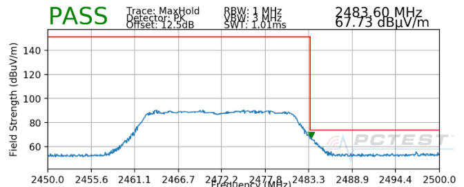
Plot 7-56. Radiated Restricted Upper Band Edge Measurement (Peak – 242 Tones)
