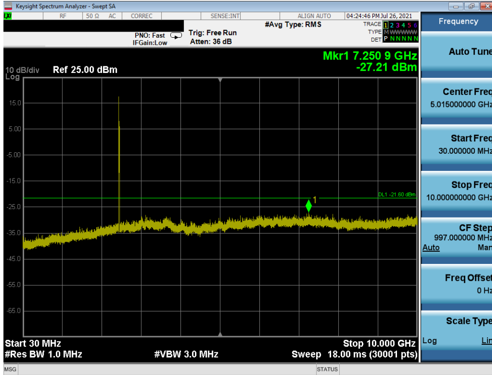
Plot 7-25. Conducted Spurious Plot (802.11ax OFDMA – 26 Tones – Ch. 11)
