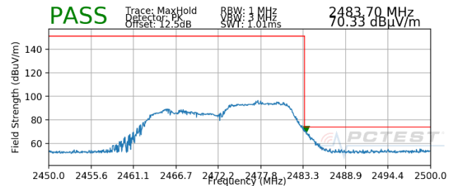
Plot 7-48. Radiated Restricted Upper Band Edge Measurement (Peak – 106 Tones)
