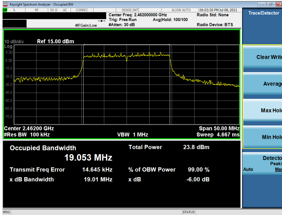
Plot 7-6. 6dB Bandwidth Plot (802.11ax OFDMA – 242 Tones – Ch. 11)
