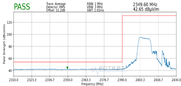
Plot 7-41. Radiated Restricted Lower Band Edge Measurement (Average – 106 Tones)
