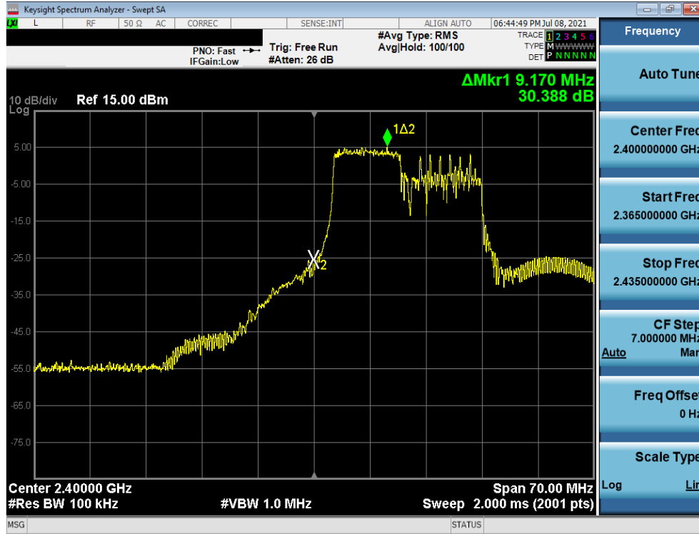
Plot 7-13. Band Edge Plot (802.11ax OFDMA – 106 Tones – Ch. 1)
