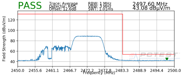
Plot 7-45. Radiated Restricted Upper Band Edge Measurement (Average – 106 Tones)
