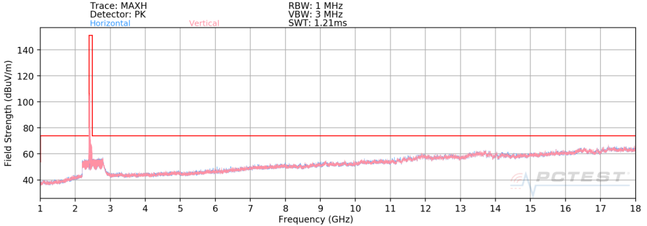
Plot 7-36. Radiated Spurious Plot above 1GHz (802.11ax OFDMA – 242 Tones – Ch. 1)
