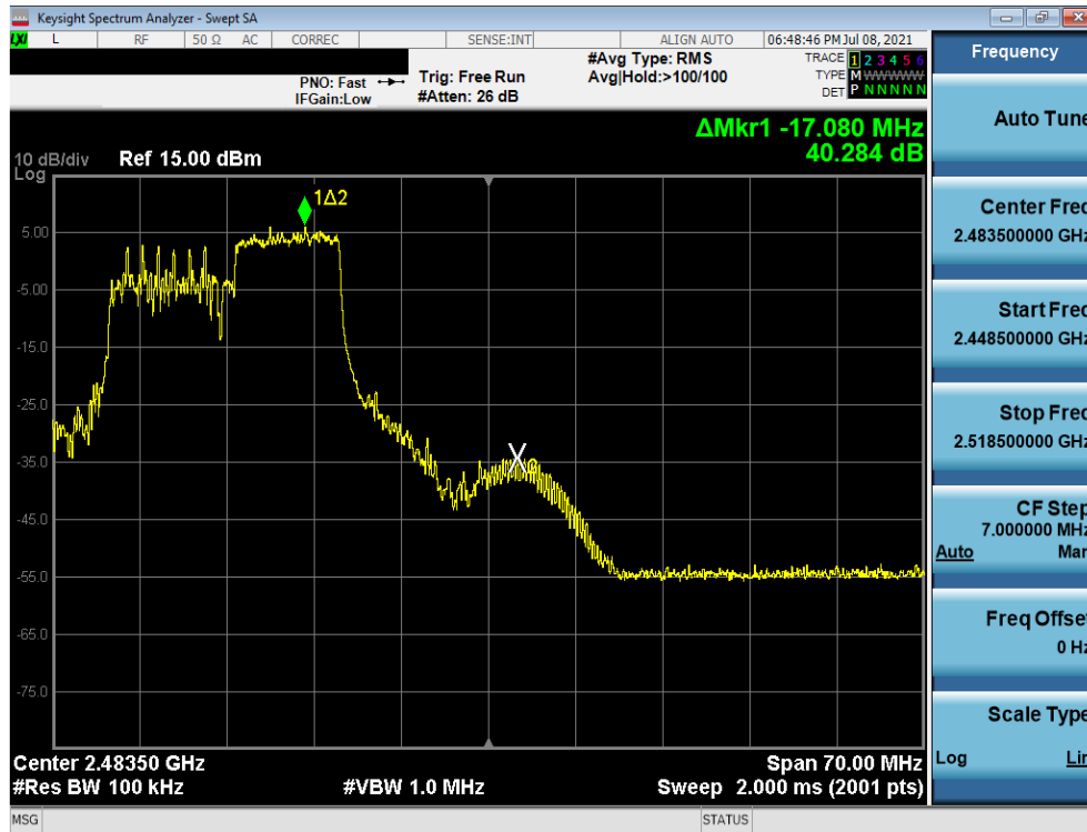
Plot 7-14. Band Edge Plot (802.11ax OFDMA – 106 Tones – Ch. 11)
