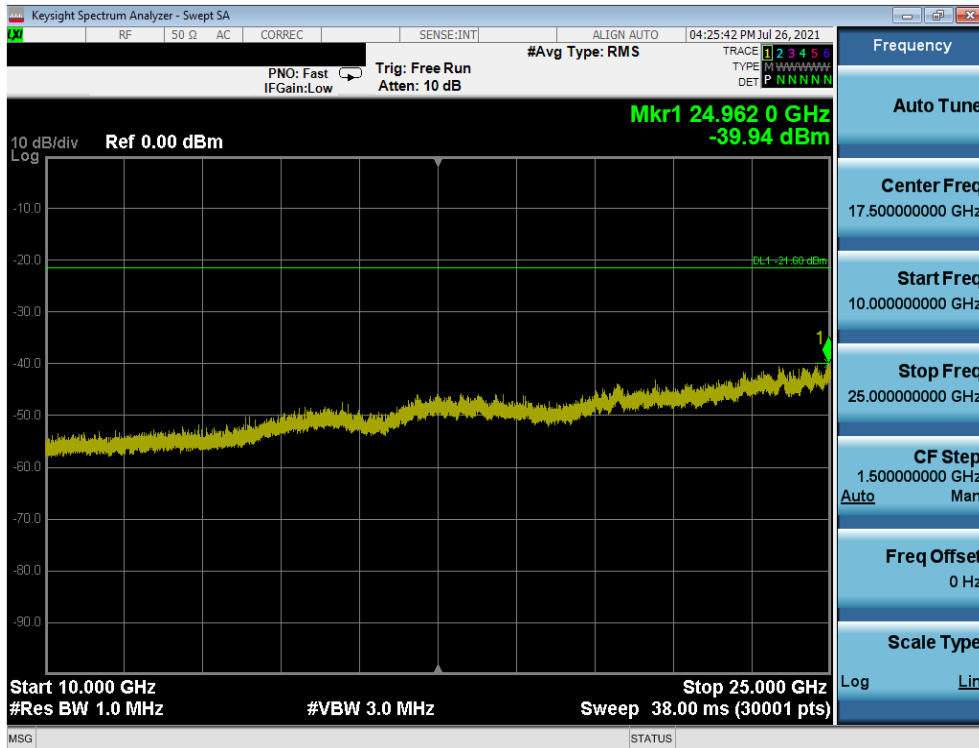
Plot 7-26. Conducted Spurious Plot (802.11ax OFDMA – 26 Tones – Ch. 11)
