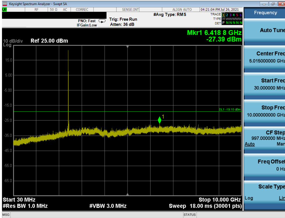
Plot 7-23. Conducted Spurious Plot (802.11ax OFDMA – 26 Tones – Ch. 6)
