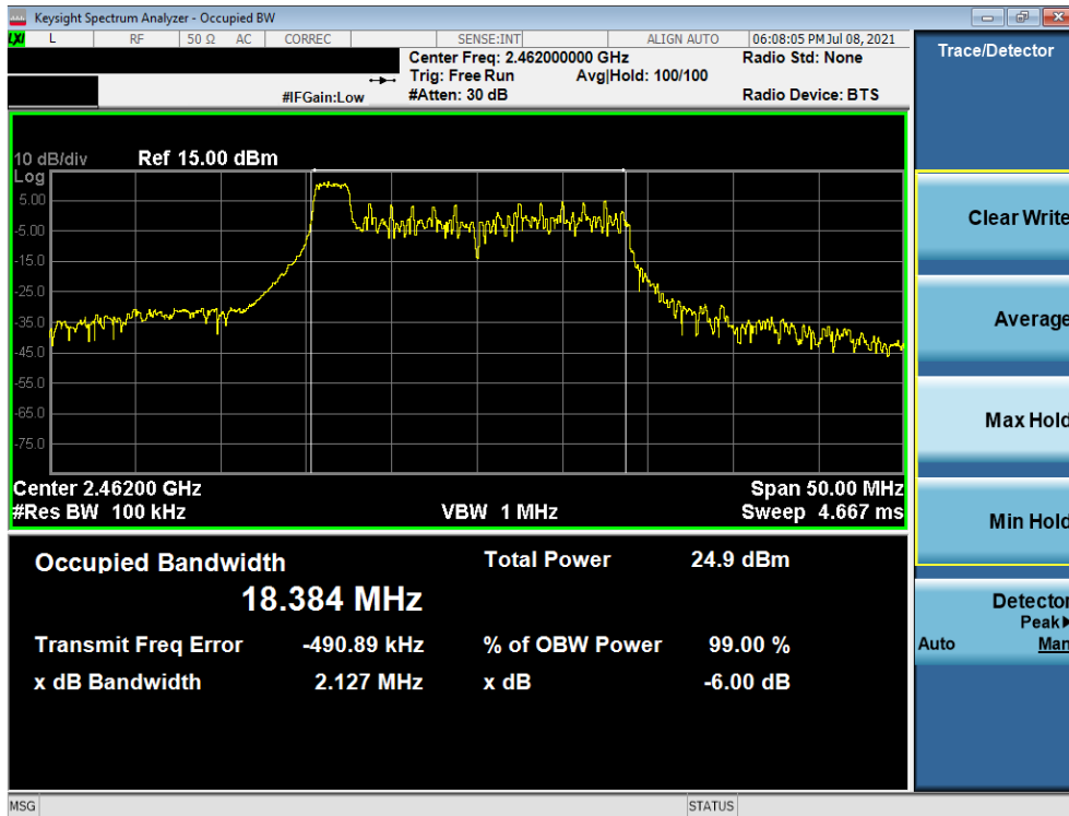
Plot 7-3. 6dB Bandwidth Plot (802.11ax OFDMA – 26 Tones – Ch. 11)
