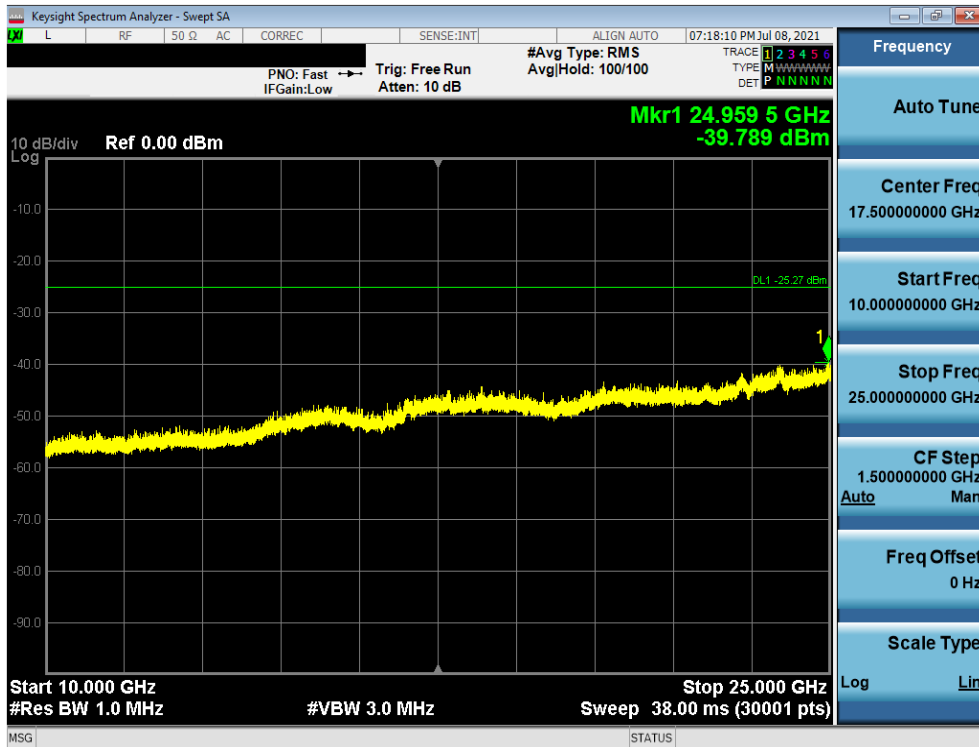
Plot 7-30. Conducted Spurious Plot (802.11ax OFDMA – 242 Tones – Ch. 6)
