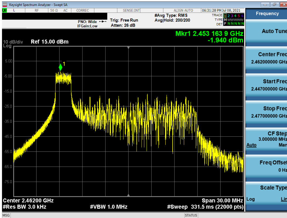
Plot 7-9. Power Spectral Density Plot (802.11ax OFDMA – 26 Tones – Ch. 11)
