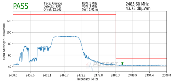
Plot 7-43. Radiated Restricted Upper Band Edge Measurement (Average – 106 Tones)
