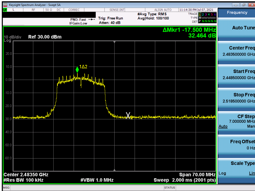
Plot 7-32. Band Edge Plot (802.11g – Ch. 13)
