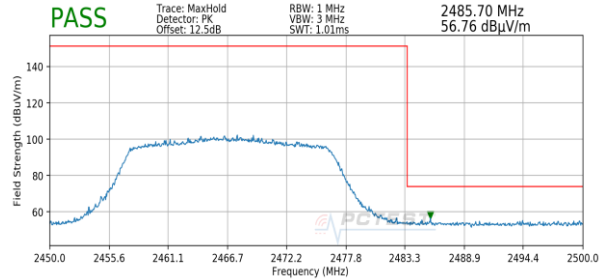
Plot 7-56. Radiated Restricted Band Edge Measurement (Peak)
