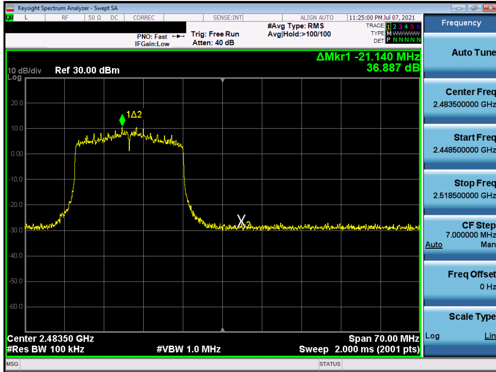
Plot 7-39. Band Edge Plot (802.11ax – Ch. 12)
