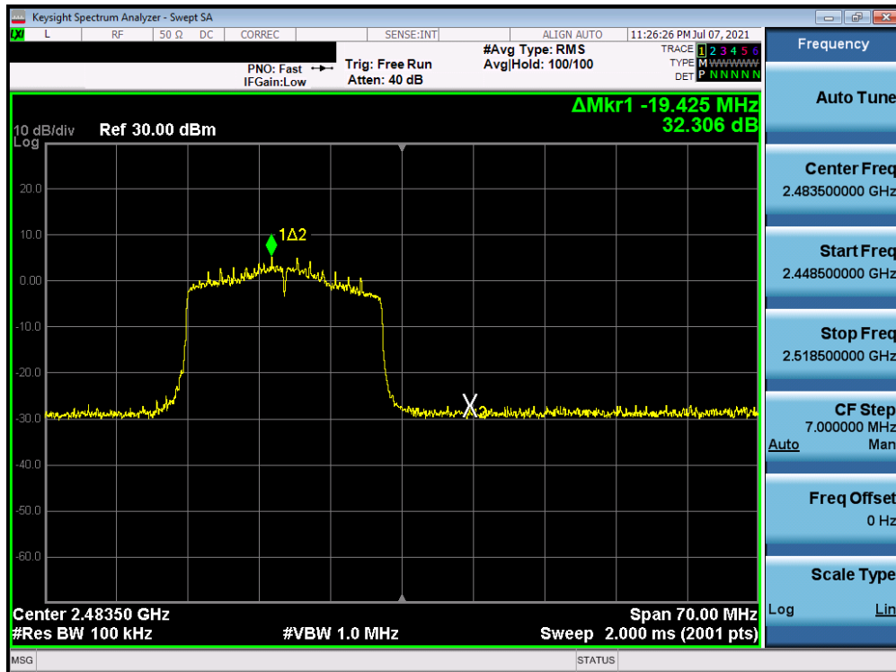
Plot 7-40. Band Edge Plot (802.11ax – Ch. 13)
