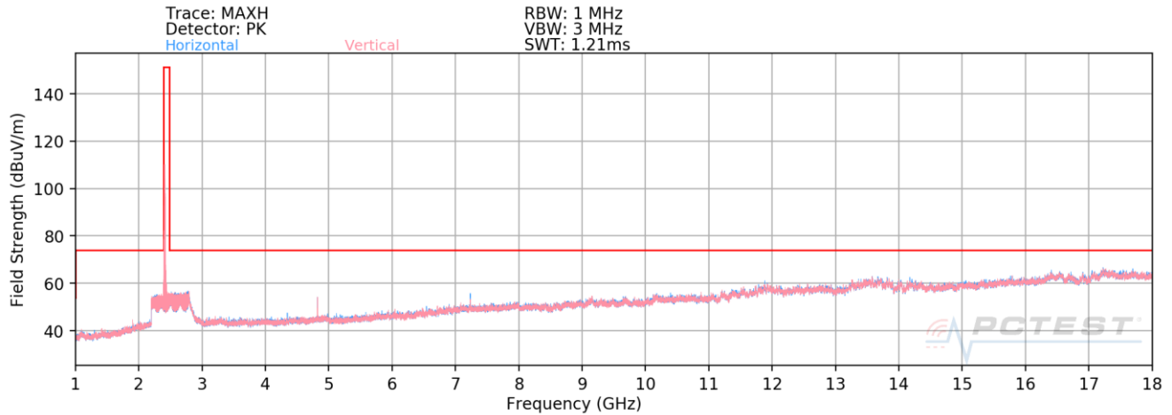
Plot 7-47. Radiated Spurious Plot above 1GHz (802.11b – Ch. 1)
