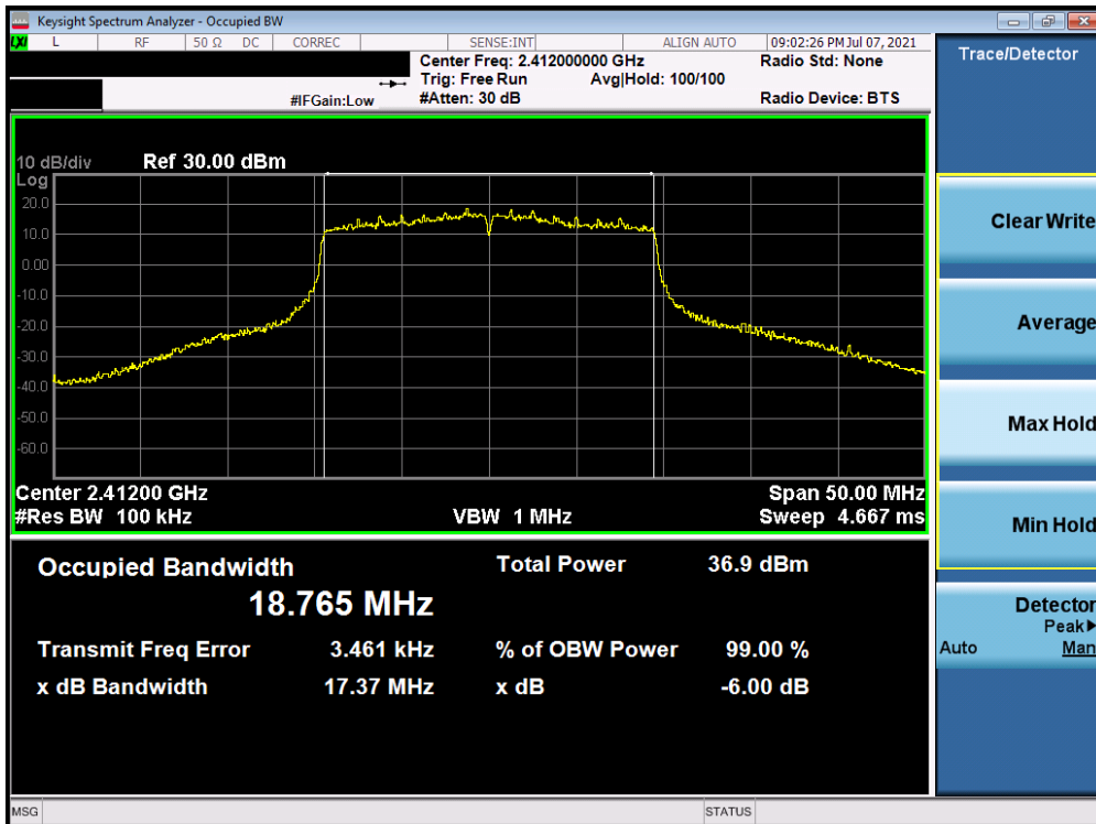
Plot 7-10. 6dB Bandwidth Plot (802.11ax – Ch. 1)
