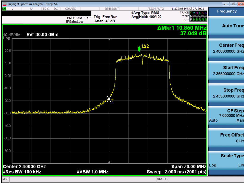
Plot 7-37. Band Edge Plot (802.11ax – Ch. 1)
