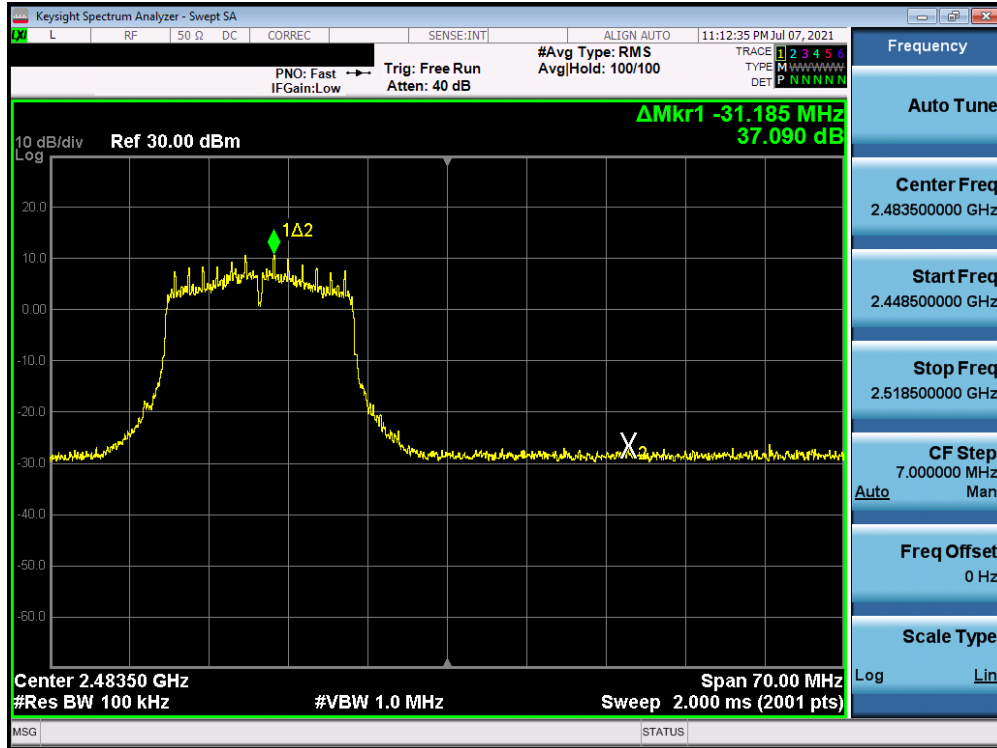
Plot 7-31. Band Edge Plot (802.11g – Ch. 12)
