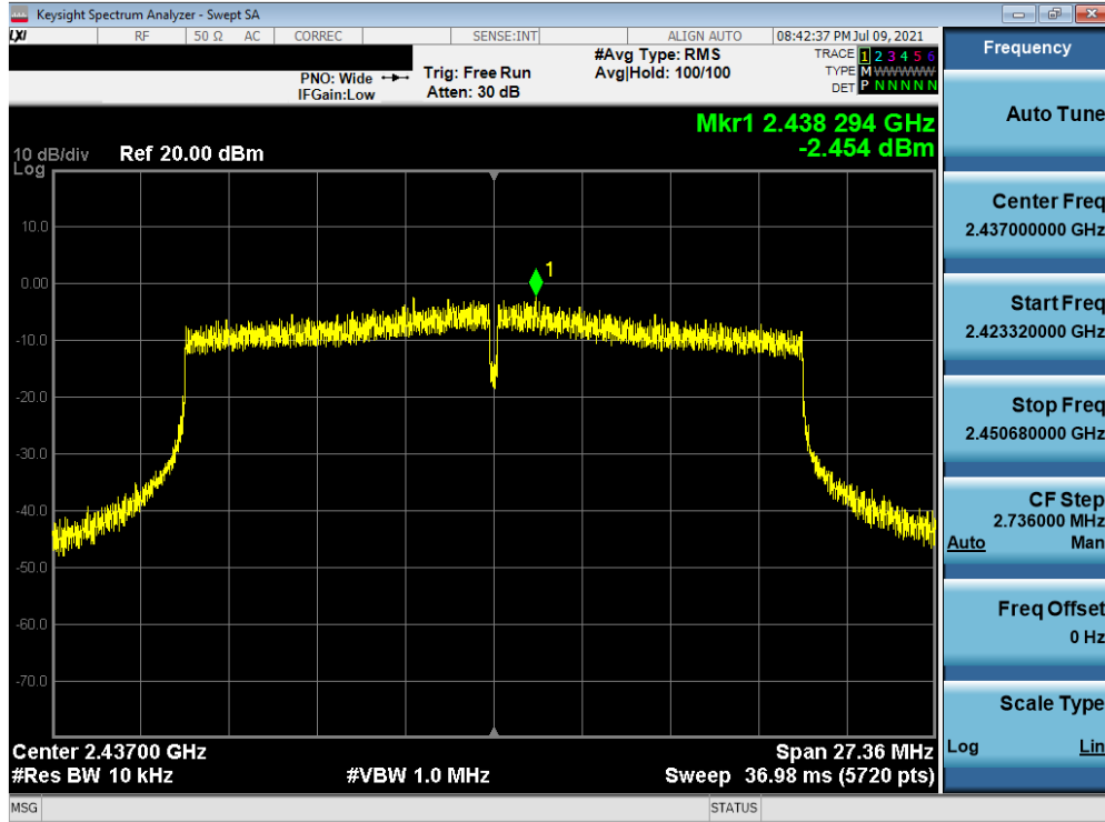
Plot 7-23. Power Spectral Density Plot (802.11ax – Ch. 6)
