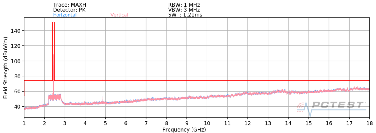
Plot 7-48. Radiated Spurious Plot above 1GHz (802.11b – Ch. 6)
