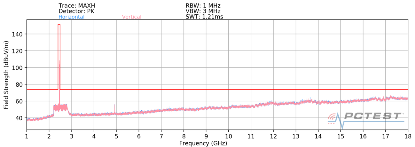
Plot 7-49. Radiated Spurious Plot above 1GHz (802.11b – Ch. 11)
