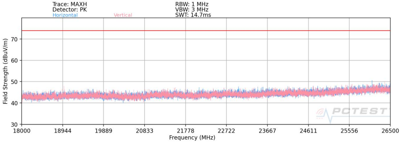
Plot 7-50. Radiated Spurious Plot above 18GHz
