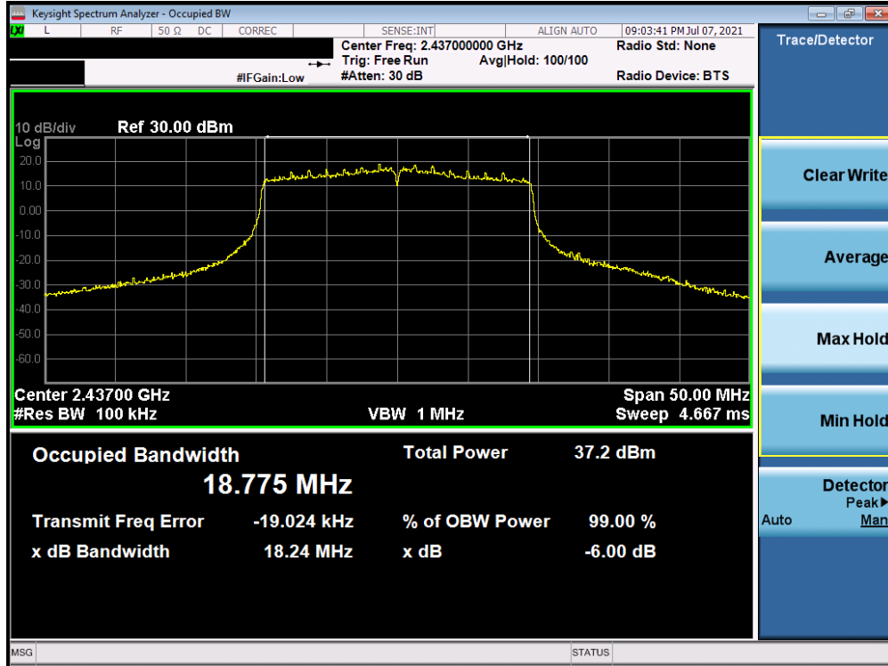
Plot 7-11. 6dB Bandwidth Plot (802.11ax – Ch. 6)
