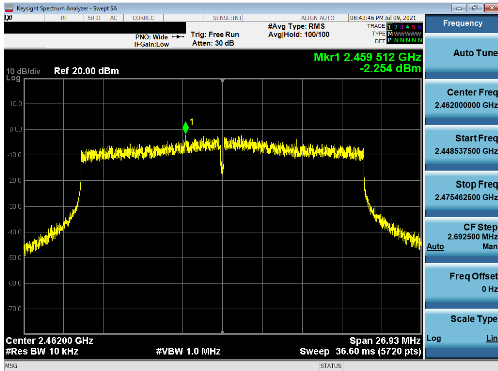
Plot 7-24. Power Spectral Density Plot (802.11ax – Ch. 11)
