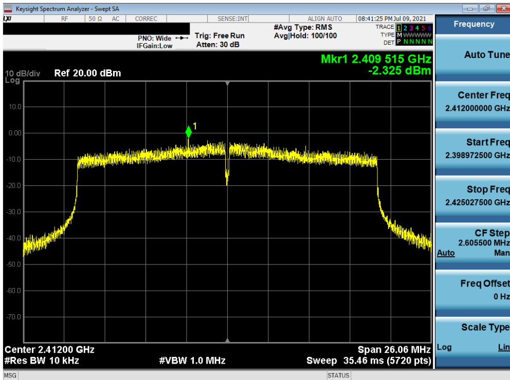
Plot 7-22. Power Spectral Density Plot (802.11ax – Ch. 1)
