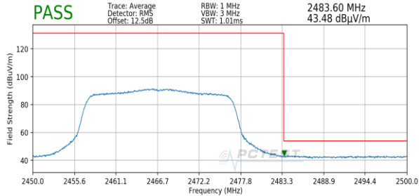
Plot 7-55. Radiated Restricted Band Edge Measurement (Average)
