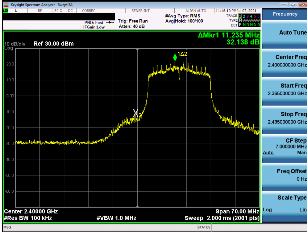
Plot 7-33. Band Edge Plot (802.11n (2.4GHz) – Ch. 1)
