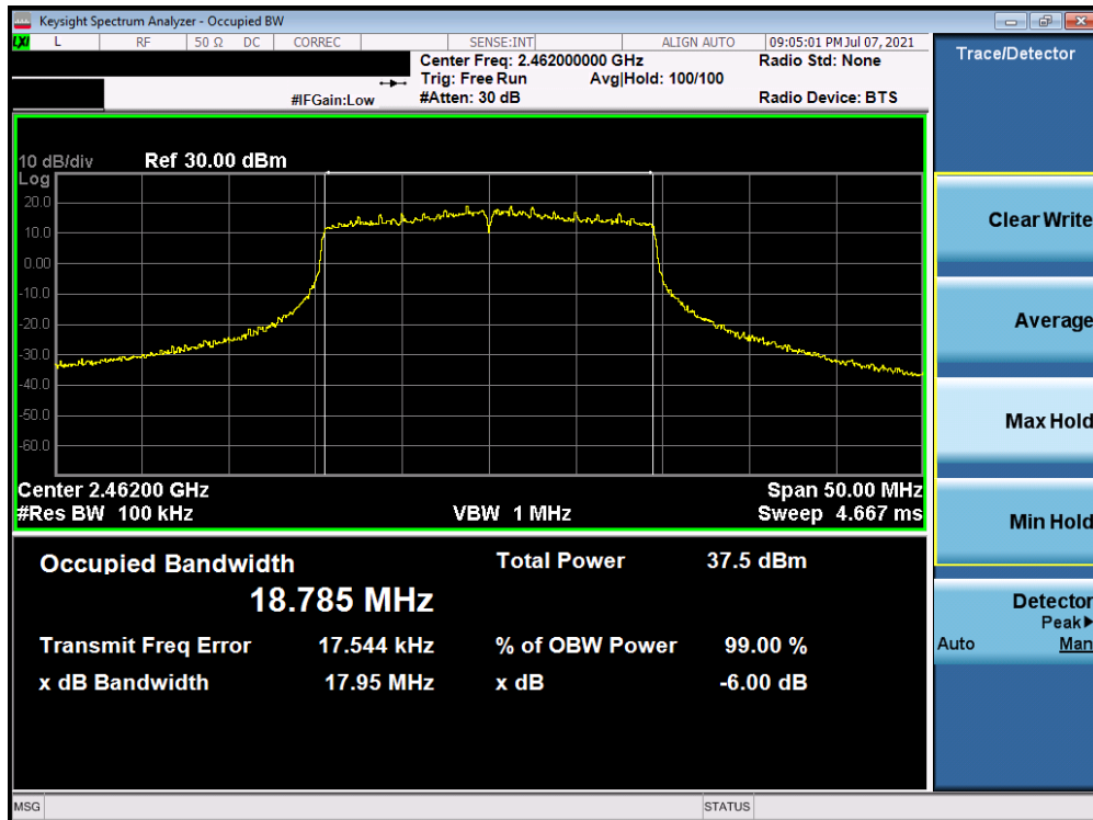
Plot 7-12. 6dB Bandwidth Plot (802.11ax – Ch. 11)
